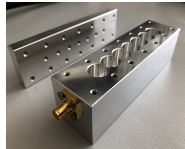
Figure 2: Custom Design Cavity Filter.
