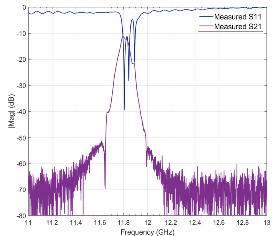
Figure 3: Measured S-Parameters of the 11.806 GHz Custom Designed Cavity Filter.
