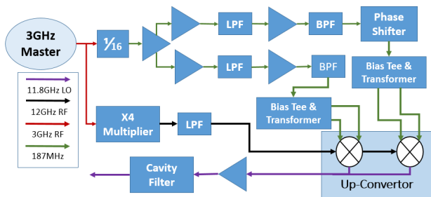
Figure 1: Single Side-band Up-Converter Schematic.
