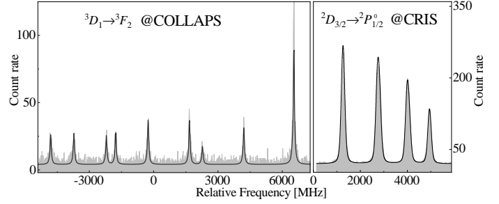
Figure 1: Hfs spectra of ^{49}\text{Sc} measured with the COLLAPS and CRIS methods on respectively ionic and atomic Sc beam. Data are fitted with a Voigt line profile using SATLAS [32].
