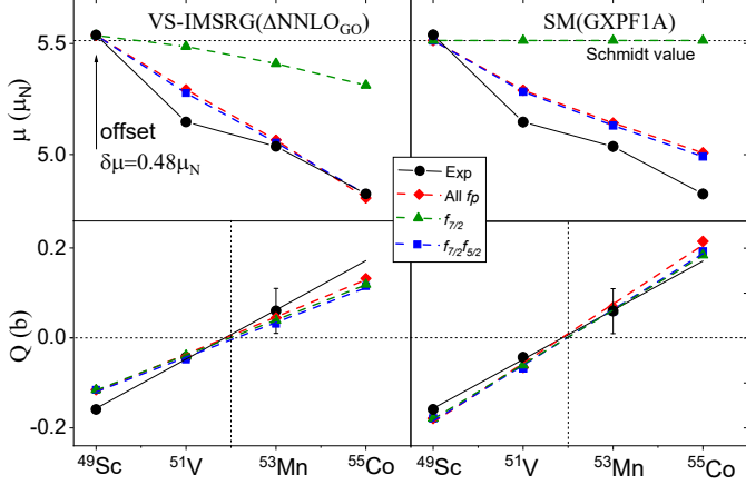
Figure 3: Nuclear moments of N = 28 isotones calculated with VS-IMSRG and SM with protons constrained on different orbits, and with neutron excitation forbidden. For a better visualization, an intended offset \delta\mu = 0.48 is added to the VS-IMSRG values.
