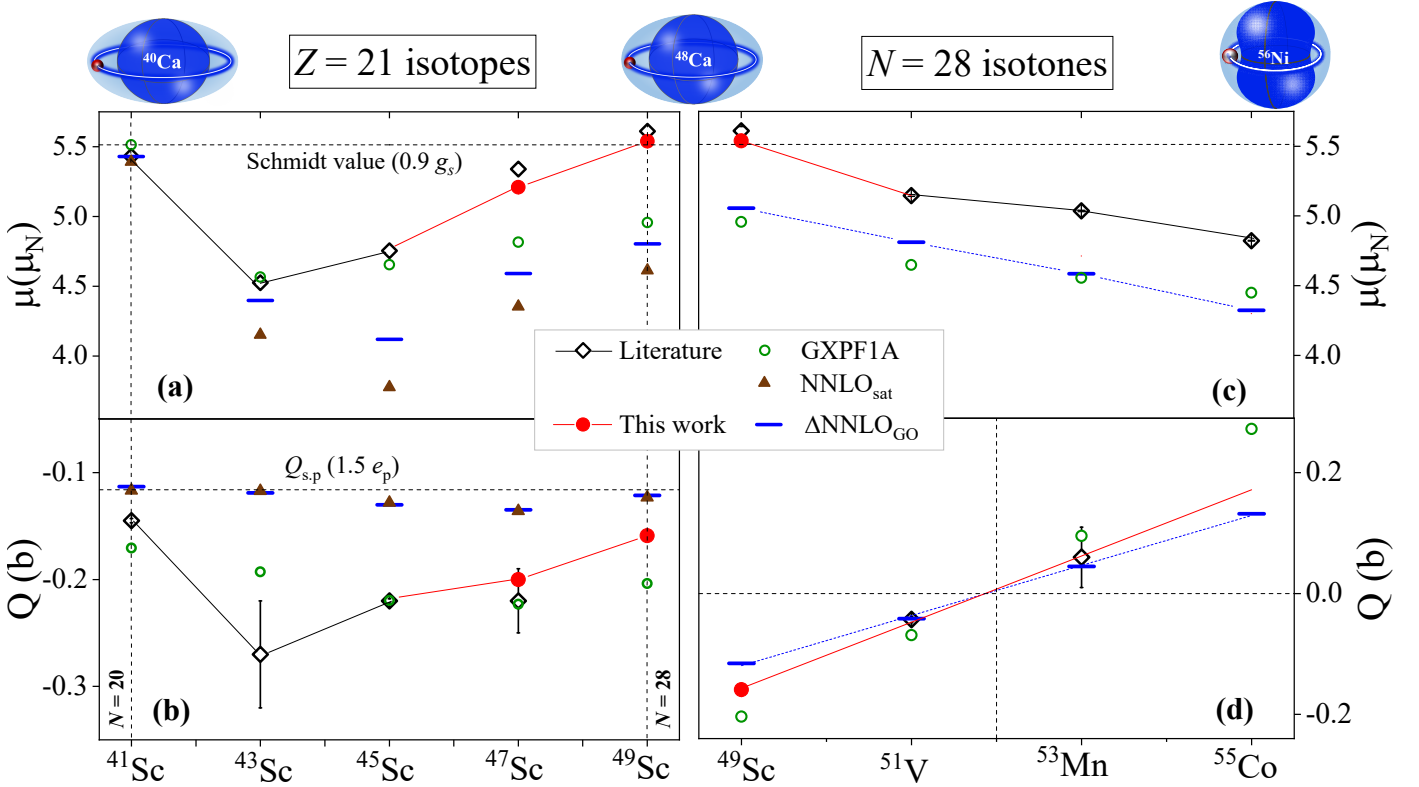
Figure 2: (a) Magnetic and (b) quadrupole moments of ^{41-49}\text{Sc} compared to SM GXPFI A calculations [41] using the effective g -factor ( g_s^{\text{eff}} = 0.9g_s^{\text{free}} ) and effective charges ( e_\pi = 1.5e , e_\nu = 0.5e ) and to VS-IMSRG calculations (using free g -factors and bare nucleon charges) based on the NNLO sat [23] and \Delta NNLO GO [24] interactions. Dashed horizontal lines indicate the effective SP magnetic and quadrupole moments of one proton in the \pi f_{7/2} orbit. (c) Magnetic and (d) quadrupole moments of N = 28 isotones, compared to theoretical calculations. ^{51}\text{V} , ^{53}\text{Mn} and ^{55}\text{Co} moments are taken from Refs. [42, 43, 44, 45, 46]. The red line in (d) is a linear fit of the data. Three sketches on the top with exaggerated deformation represent the shapes of ^{41,49}\text{Sc} with a proton outside ^{40,48}\text{Ca} and of ^{55}\text{Co} with a hole inside ^{56}\text{Ni} .
