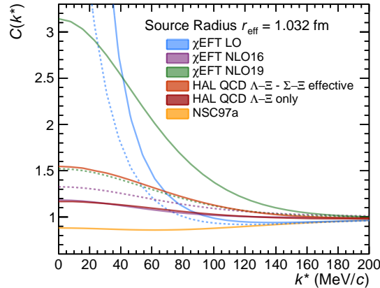
Figure 1: Theoretical \Lambda - \Xi^- correlation functions from predictions ([2, 11, 12, 16]) evaluated for the experimental source radius. See text for details. In the case of the LO and NLO \chi EFT potentials the solid (dotted) lines correspond to the lowest (highest) cutoff [11, 16].
