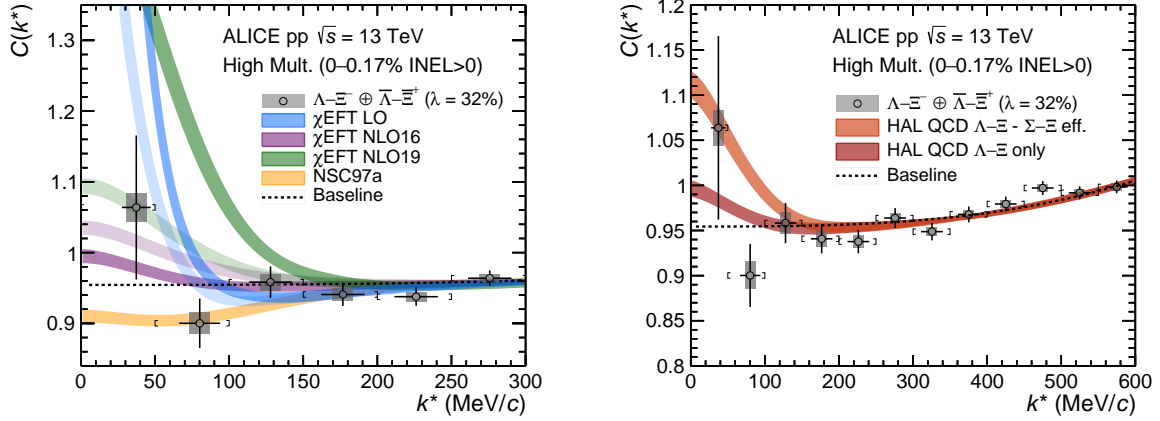
Figure 2: Experimental \Lambda - \Xi^- correlation function with statistical (vertical black lines) and systematic (gray boxes) uncertainties. The square brackets show the bin width of the measurement and the horizontal black lines represent the statistical uncertainty in the determination of the mean k^* for each bin. Left panel: Comparison to LO [11] and NLO [16] \chi EFT and NSC97a [12] potentials evaluated with the Lednický-Lyuboshits model [40, 41]. In the \chi EFT models the darker and light bands correspond to the version with the lower and higher cut-off value, respectively. Right panel: Comparison with Lattice QCD calculations by the HAL QCD Collaboration [2] using an effective potential including the coupling to \Sigma - \Xi (orange) and the \Lambda - \Xi^- elastic potential alone (red). The width of the bands in both panels correspond to the systematic uncertainties of the fit as described in the text. The dotted black line represents the result of the baseline fit assuming no \Lambda - \Xi^- strong interaction.
