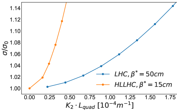
Figure 2: Relative increase in beam size at the IP from different settings of the colinearity knob for LHC and HL-LHC, creating a closed local coupling bump.
