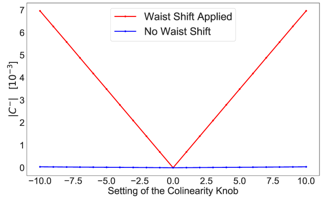
Figure 4: Impact of the colinearity knob on the global |C^-| with and without applying a rigid waist shift.
