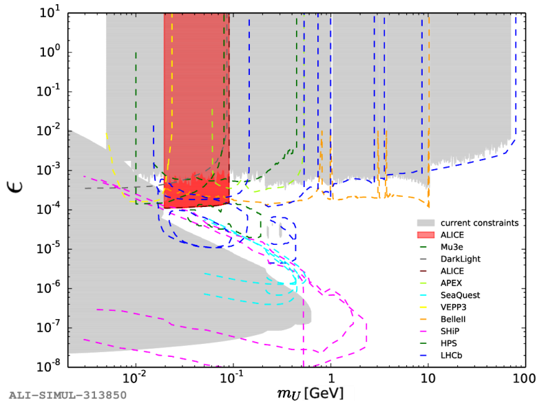
Figure 5: Dark photon limits in the coupling vs. mass plane. The red area indicates the expected 90% C.L. constraints from ALICE measurements before 2030. Figure adapted from Refs. [2, 115].
