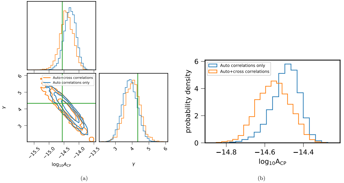
Figure 3. Comparison of common-spectrum process parameters when using auto-correlations only and the full auto+cross-correlated HD model. left: 2D posterior for common-spectrum process power law parameters. Green lines mark \gamma = 13/3 and A_{CP} = 2.8 \times 10^{-15} , while the contours represent the 1-, 2- and 3- \sigma confidence intervals. right: 1D posterior for common-spectrum process power law amplitude, using fixed spectral index \gamma = 13/3 .
