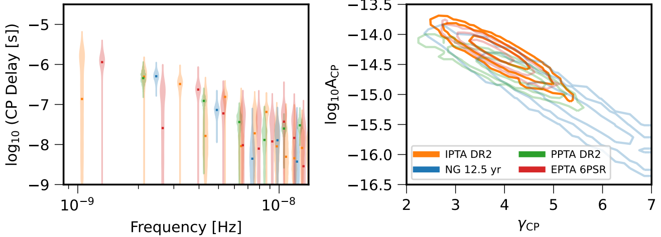
Figure 9. Comparison of IPTA DR2 to other recent data sets. left: Free spectral common-spectrum process model. The inclusion of legacy data not used in recent PTA analyses allows IPTA DR2 to reach lower frequencies despite missing the most recently collected data. right: 2D posterior for CP parameters log-amplitude and spectral index, where the contours represent the 1-, 2-, and 3- \sigma confidence intervals. All recent data sets are in broad agreement on the characteristics of a common-spectrum process.
