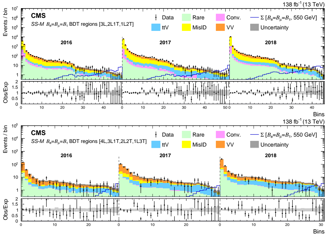
Figure 14: The SS\text{-}M \mathcal{B}_e = \mathcal{B}_\mu = \mathcal{B}_\tau BDT regions for the 3-lepton (upper) and 4-lepton (lower) channels for the 2016–2018 data sets. The lower panel shows the ratio of observed events to the total expected background prediction. The gray band on the ratio represents the sum of statistical and systematic uncertainties in the SM background prediction. The expected SM background distributions and the uncertainties are shown after fitting the data under the background-only hypothesis. For illustration, an example signal hypothesis for the production of the type-III seesaw heavy fermions in the flavor-democratic scenario for m_\Sigma = 550 GeV, before the fit, is also overlaid.
