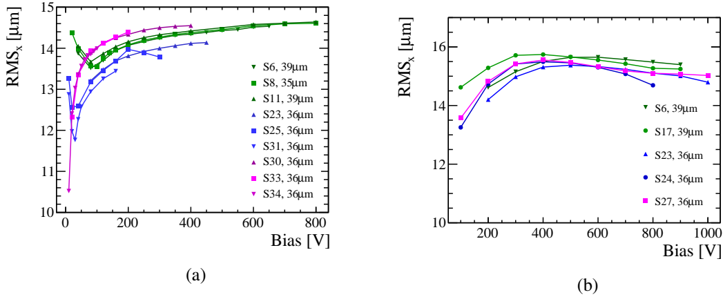
Figure 8. The spatial resolution as a function of bias voltage for non-irradiated sensors (a) and for uniformly irradiated sensors to the 8 \times 10^{15} \text{1 MeV n}_{\text{eq}} \text{cm}^{-2} (b). Green for HPK n-on-p, blue for Micron n-on-p and purple for Micron n-on-n.
