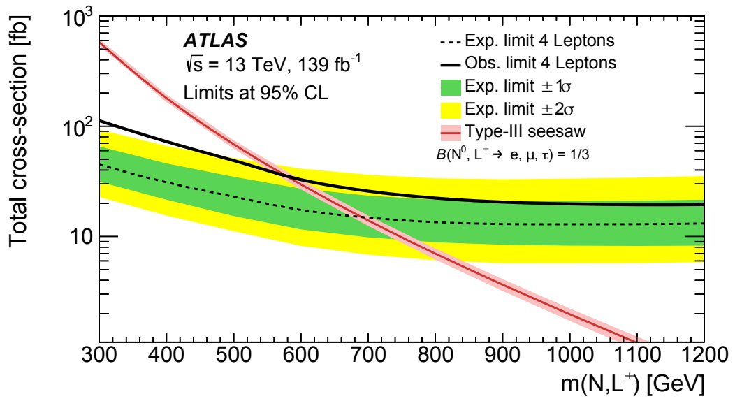
Figure 9: Expected and observed 95% CL_s exclusion limits in the four lepton channel for the type-III seesaw process with the corresponding one- and two-standard-deviation bands, showing the 95% CL upper limit on the cross-section. The theoretical signal cross-section prediction, given by the NLO calculation [35, 36], is shown with the corresponding uncertainty bands for the expected limit.
