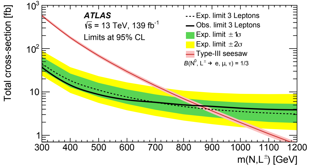
Figure 8: Expected and observed 95% CL_s exclusion limits in the three lepton channel for the type-III seesaw process with the corresponding one- and two-standard-deviation bands, showing the 95% CL upper limit on the cross-section. The theoretical signal cross-section prediction, given by the NLO calculation [35, 36], is shown with the corresponding uncertainty bands for the expected limit.
