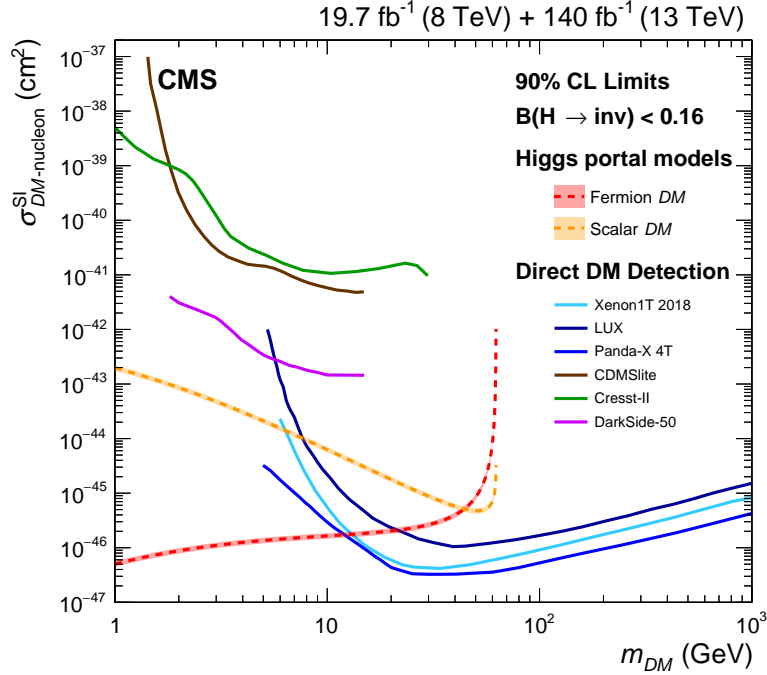
Figure 13: The 90% CL upper limits on the spin-independent DM-nucleon scattering cross section in Higgs-portal models, assuming a scalar (dashed orange) or fermion (dashed red) DM candidate. Limits are computed as functions of m_{DM} and are compared to those from the XENON1T [80], CRESST-II [81], CDMSlite [82], LUX [83], Panda-X 4T [84], and DarkSide-50 [85] experiments, which are shown as solid lines.
