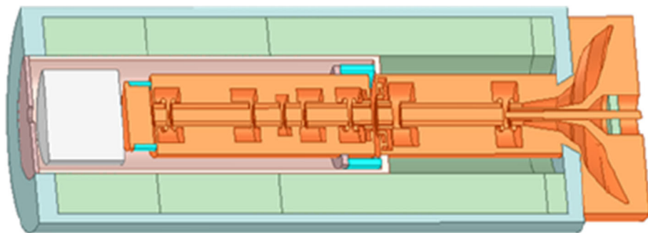
Fig. 4 Artist's view of the Two-Stage MBK for FCC-ee
