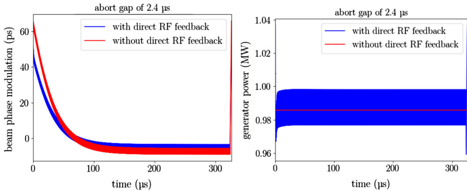
Fig. 1 Variation of bunch-by-bunch phase with and without the direct RF feedback (left plot) and instantaneous generator power within one turn (right plot)
