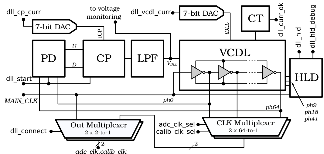
Figure 4. Delay-Locked Loop (DLL) block diagram: PD—Phase Detector, CP—Charge Pump, LPF—Low Pass Filter, VCDL—Voltage Controlled Delay Line, CT—Current Test, HLD—Harmonic Lock Detector.
