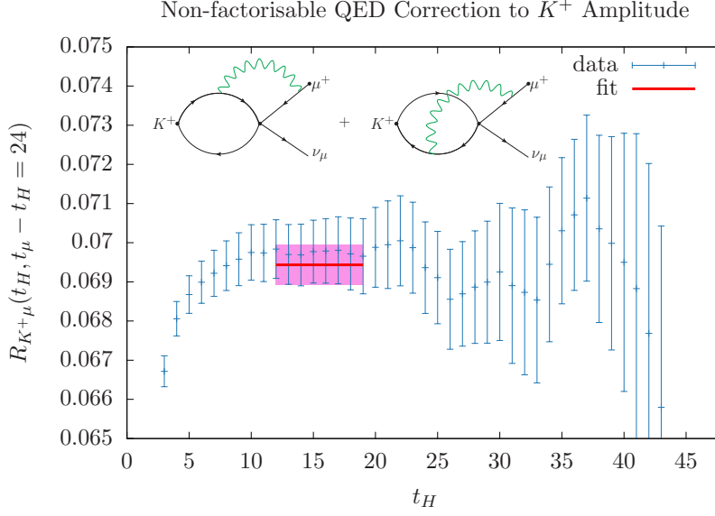
Figure 4: The non-factorisable correlator ratio defined in Equation (29). The red line and pink error band is the result of a combined fit of the hadron-leptonic correlators, in which only t_{\mu} - t_H = 24 is shown here. For this combined fit, \chi^2/dof = 29/31 = 0.94 , p -value = 0.812.
