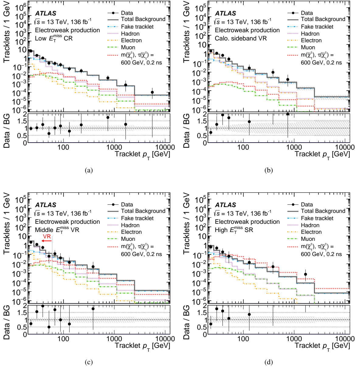
Figure 5: Pixel tracklet p_T spectrum fit results in the low-, middle- and high- E_T^{\text{miss}} regions for the electroweak production channel. The fake-tracklet, hadron, electron and muon templates are fitted to observed data events in a background-only fit. An example of the expected-signal prediction with m_{\tilde{\chi}_1^\pm} = 600 \text{ GeV} and \tau_{\tilde{\chi}_1^\pm} = 0.2 \text{ ns} is overlaid in red. The last bin includes overflow entries. The bottom panel shows the ratio of data to the background-only prediction.
