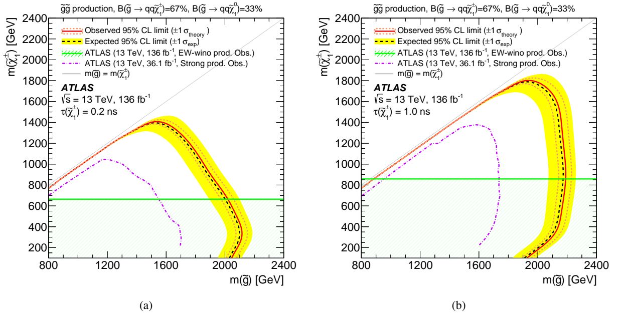
Figure 9: Exclusion limits at 95% CL obtained in the strong production channel. The limits are shown as a function of the lightest chargino's mass versus the gluino's mass, for chargino lifetimes of (a) 0.2 ns and (b) 1.0 ns. The black dashed line shows the median expected value, and the yellow band shows the 1\sigma uncertainty around the expected limits. The red line shows the observed limits and the red dotted lines show the 1\sigma uncertainty from the signal cross-section. The observed exclusion limits from this search in the direct electroweak wino production channel in the minimal AMSB model with (a) \tau_{\tilde{\chi}_1^\pm} = 0.2 ns and (b) \tau_{\tilde{\chi}_1^\pm} = 1.0 ns are overlaid in green. The violet broken line shows the observed limits from the previous ATLAS result [16].
