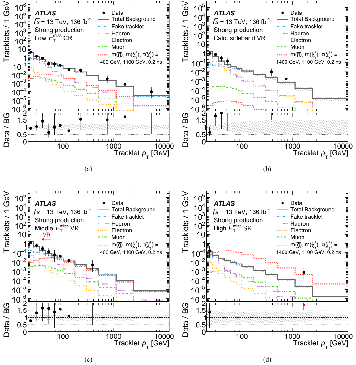
Figure 6: Pixel tracklet p_T spectrum fit results in the low-, middle- and high- E_T^{\text{miss}} regions for the strong production channel. The fake-tracklet, hadron, electron and muon templates are fitted to observed data events in a background-only fit. An example of the expected-signal prediction with m_{\tilde{g}} = 1400 GeV, m_{\tilde{\chi}_1^\pm} = 1100 GeV and \tau_{\tilde{\chi}_1^\pm} = 0.2 ns is overlaid in red. The last bin includes overflow entries. The bottom panel shows the ratio of data to the background-only prediction. The arrow indicates a value outside of the range of the bottom inset.
