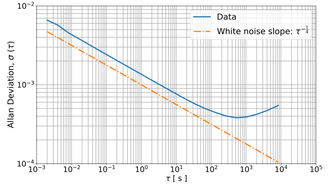
FIG. 20. Stability measurement of the current source. Depicted (solid line) is the fractional overlapping Allan deviation of a 18 hours long-term current measurement. The bias stability is about 4 \times 10^{-4} at 500 s averaging time. Comparison to a white noise slope (dotted-dashed line) shows that for shorter averaging time the deviation is caused by white noise.
