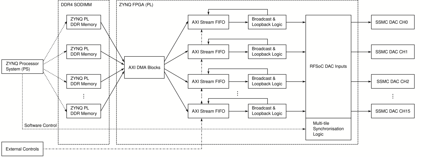
FIG. 4. The FPGA logic for the DAC waveforms generation. The figure shows the data flow from the processor system (PS), going through the DDR memory and into the AXI Stream FIFO before it is sent out through the sixteen DAC channels. A multi-tile synchronisation logic ensures that all channels are synchronised.
