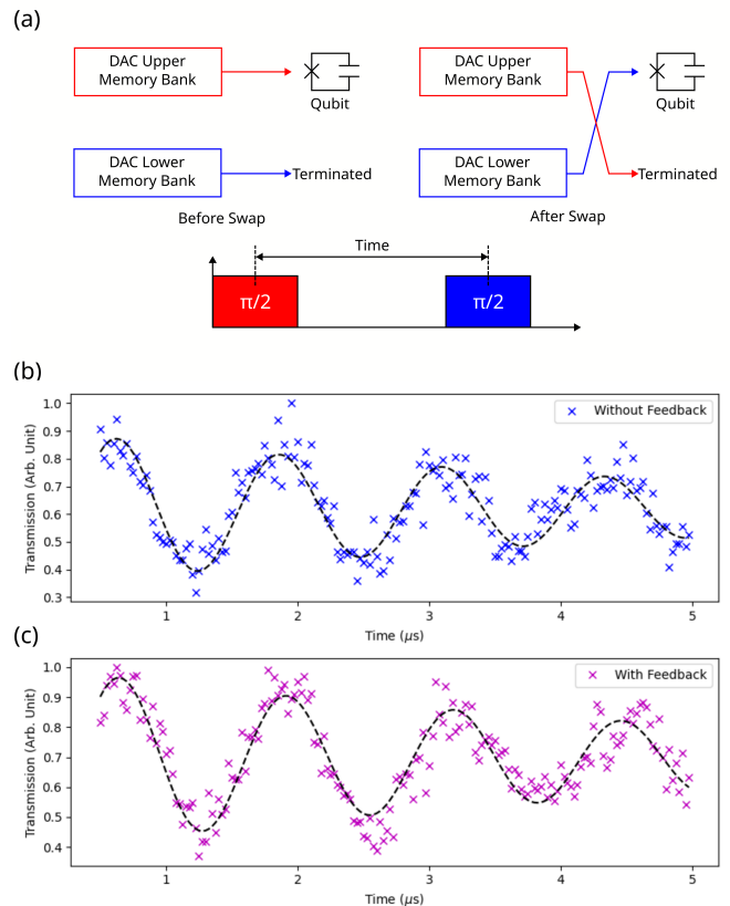
FIG. 15. Ramsey fringes performed with the feedback control (i.e. swapping of the DAC memory banks). (a) To test the effects of the feedback, we carried out a Ramsey experiment where the first \pi/2 -pulse originated from the original memory bank and the second \pi/2 -pulse was generated from the swapped memory bank. The Ramsey fringes (b) without and (c) with feedback control. Each point was averaged over 1000 measurements. The fits yield dephasing times of 4.84 \mu\text{s} and 5.08 \mu\text{s} , respectively. This experiment was performed at a different cooldown as compared to Fig. 14.
