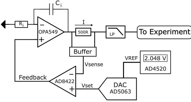
FIG. 18. Current control circuit. The output current of an operational amplifier is stabilised by integral feedback. The setpoint is generated by a DAC, which is referenced to a precise voltage reference. Details like supply voltages, decoupling capacitors and connectors have been omitted for clarity.
