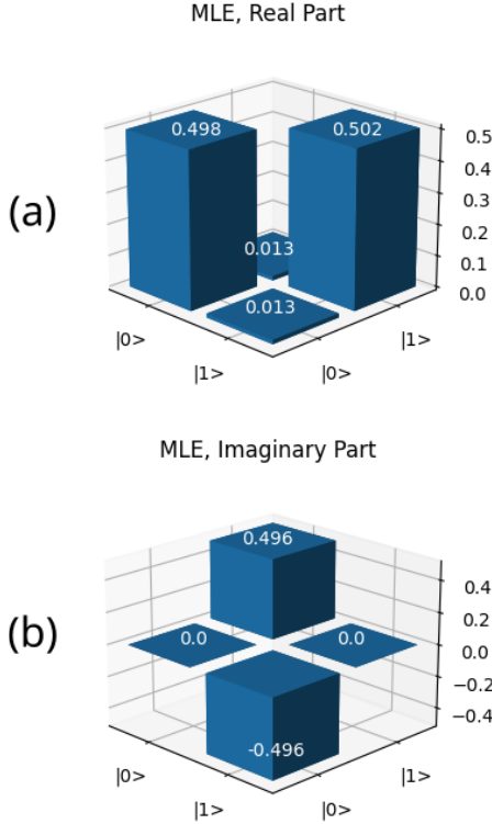
FIG. 16. Quantum State Tomography for \frac{1}{\sqrt{2}}(|0\rangle - i|1\rangle) . The figure shows the (a) real and (b) imaginary parts of the Maximum Likelihood Estimate (MLE) fit. A \pi/2 -pulse is applied before prerotation. The state fidelity from MLE is 99.8%.
