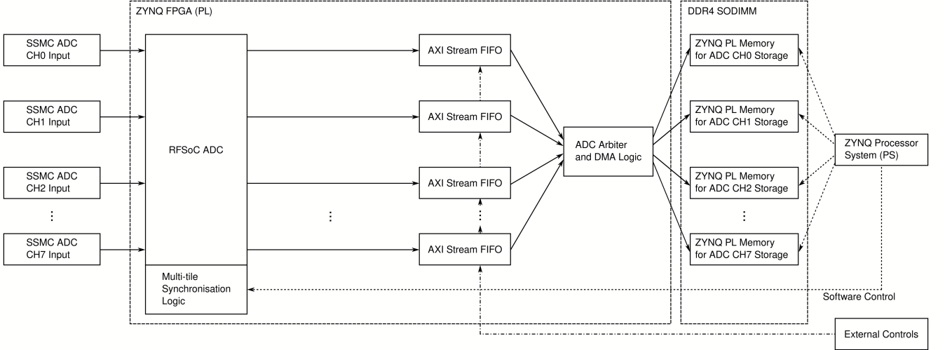
FIG. 5. The FPGA logic for the ADC waveforms acquisition. The data from the eight ADC channels are streamed to the AXI Stream FIFO gets moved into the DDR memory via the ADC Arbiter and DMA Logic, only when a trigger is received. The ADC arbiter and DMA logic then transfers the data to the programmable logic (PL) memory for storage when an instruction is received from the processor system (PS). A multi-tile synchronisation logic ensures that all channels are synchronised.
