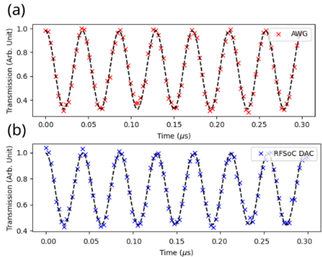
FIG. 13. Rabi oscillation of the qubit using (a) AWG and (b) RFSoc DAC, respectively. The qubit was driven with pulse durations up to 300 ns in 3 ns intervals. Each point was averaged over 1000 measurements. Through a sine wave fit, we approximate the Rabi oscillation frequency f_{\text{Rabi}} as 23.3 MHz for the AWG and 23.5 MHz for the RFSoc. We also obtain the \pi -pulse duration t_{\pi} of 21.5 ns for the AWG and 21.2 ns for the RFSoc.
