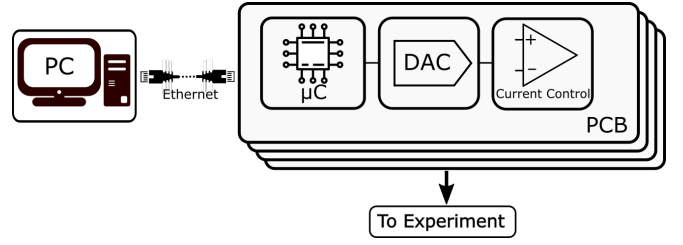
FIG. 17. Working principle of the DC current source. A host PC sends current values data to a microcontroller via an Ethernet interface. Subsequently the microcontroller changes the setpoint of the current control circuit via reprogramming the DAC.
