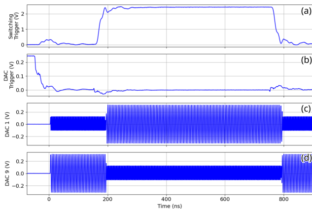
FIG. 11. DAC playback switching with hardware trigger signals. (a) The switching trigger sent to the RFSoc. (b) The DAC trigger sent to the RFSoc. (c-d) Upon receiving the switching trigger, the upper DAC memory banks (DACs 0 to 7) switches with the lower banks (DACs 8 to 15). The delay from the trigger to completion of switching of the channels took approximately 20 \pm 5 ns.
