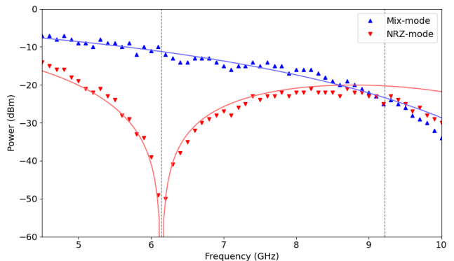
FIG. 8. Output power of the RFSoc DAC from 4.5 to 10 GHz, corresponding to parts of the first three Nyquist zones. The zones are delineated by the dashed lines.
