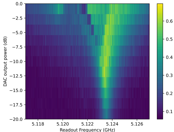
FIG. 12. Cavity transmission response. We plot the amplitude of the Fourier transform of the readout signal from the ADC as a function of DAC power and cavity driving frequency. The cavity was driven for 10 \mu\text{s} near its resonance frequency over 20 dB of power with a rest period of 200 ms. At each point, the amplitude was averaged over 100 shots. The dressed cavity frequency is at 5.12375 GHz and from the data we are able to resolve the frequency at -12 dB. The bare frequency of 5.12 GHz is slightly visible at the highest power of the instrument.
