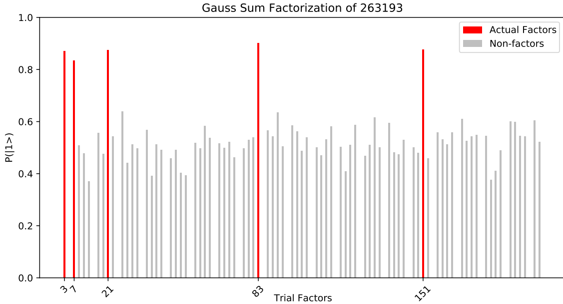
FIG. 24. Excited state probability for each trial factors up to 200 in the factorization of 263193. We apply the preprocessing technique in [42] to skip over multiples of 2 and 5 as they provide bad contrast compared to the actual factors. The expected factors in this regime are 3, 7, 21, 83, 151 (highlighted in red). We can see that the major peaks near 1 correspond to the factors, allowing us to identify factors and composite factors. The lowest excited state probability for the factors is 0.834 while the highest excited state probability of the non-factors is 0.639 at l = 27 . The behaviour of this non-factor is discussed in more detail in Ref. [42].
