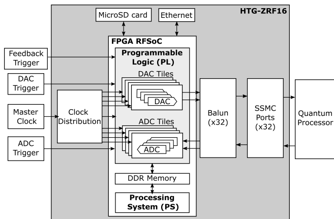
FIG. 3. Some of the features on the HTG-ZRF16 board that are used in this setup. The board takes in multiple triggers and a clock signal as reference for the FPGA logic. The clock distribution subsystem distributes it to the FPGA as well as the DACs and ADCs tiles. The DACs and ADCs tiles generates differential microwave signals, which are converted to single-ended signals and transmitted out via SSMC ports. The board also supports communication via microSD card and Ethernet.
