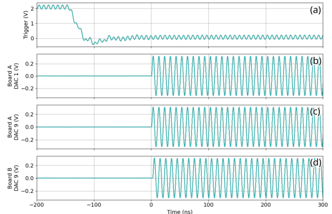
FIG. 10. Synchronisation of the DAC channels from multiple boards. (a) Using a synchronised trigger signal, 10 runs of the DAC were captured. (b-d) The DAC outputs from two RFSoc boards (Boards A and B) were connected to an oscilloscope and synchronisation between channels of the same board and between multiple boards were achieved.
