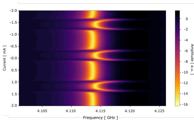
FIG. 21. Transmission spectrum of a cavity dispersively coupled to a tunable superconducting transmon qubit. Shown are the spectra for current values from -2.0 mA to 2.0 mA. In this range the frequency of the qubit is going through 3 periodic changes. A continuous wave using a vector network analyzer was used for the readout drive.
