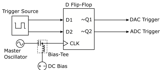
FIG. 9. Schematic of the d-type flip-flop circuit. The two independent falling-edge trigger signals for the DAC outputting and the ADC sampling ( Q1 and Q2 ) are provided by the trigger source ( D1 and D2 ) and are synchronised to a master oscillator using a dual-channel d-type flip-flop. An appropriate DC bias is supplied to the clock input of the flip-flop, so that the AC clock signal from the oscillator moves through the on/off levels.
