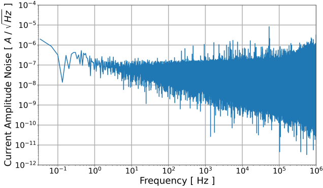
FIG. 19. High frequency amplitude noise of the DC current source. The total noise in the band of 0.1 Hz to 10 kHz is 1.3 \times 10^{-7} A rms .
