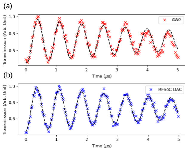
FIG. 14. Ramsey fringes. We vary \tau up to 5 \mu\text{s} and apply a frequency detuning of 1 MHz using (a) the AWG and (b) the RFSoc. Each point was averaged over 1000 measurements. The data is fitted to a sine wave with an exponential decay, yielding an oscillation of frequency 1.367 MHz and dephasing time of 6.66 \mu\text{s} for the RFSoc and similar values of 1.38 MHz and 6.52 \mu\text{s} for the AWG, respectively.
