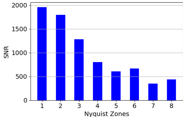
FIG. 7. SNR measurements of DAC output at different ADC Nyquist zones. The signal in the first zone is at 800 MHz and the ones in the higher zones are its aliases. The DAC output is passed through filters to only select the alias frequency that corresponds to each ADC Nyquist zone. For example: The DAC outputs a 4732.16 MHz signal (using its second zone) and is filtered with a 2.7-6.0 GHz bandpass filter; it is sampled in the ADC's as 800 MHz (using its fifth zone). The SNRs were calculated in frequency domain using the signal peak amplitude and the average noise within a bandwidth of 100 MHz.
