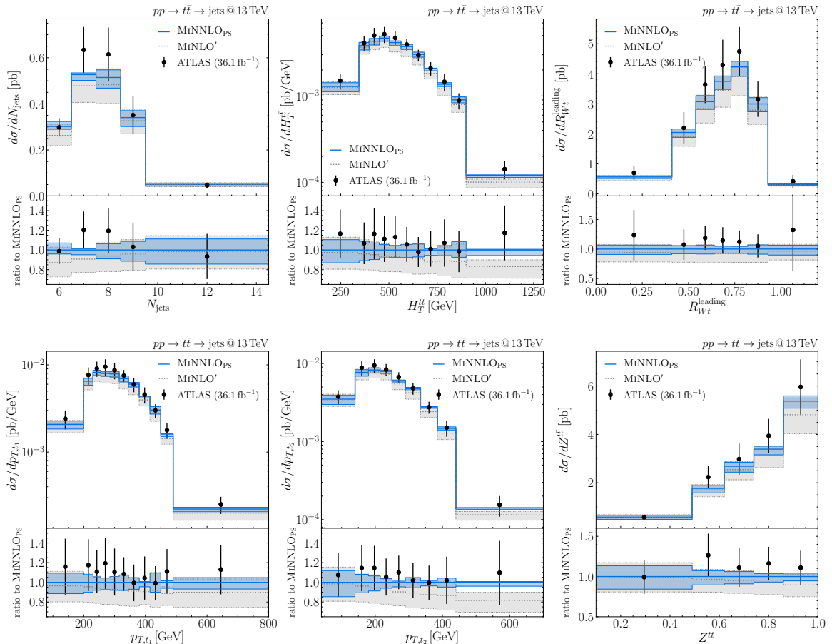
Figure 5. Comparison of \text{MiNNLO}_{\text{PS}} (blue, solid) and \text{MiNLO}' (black, dashed) predictions with ATLAS data [48] (black points with errors) in setup-hadronic .
