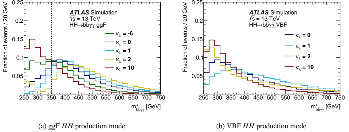
Figure 5: The m_{b\bar{b}\gamma\gamma}^* distributions after the common preselection for (a) nonresonant ggF HH and (b) VBF HH signals with several \kappa_\lambda values. The value of m_{b\bar{b}\gamma\gamma}^* = 350 GeV is chosen as the boundary between categories targeting the SM and BSM \kappa_\lambda signals.
