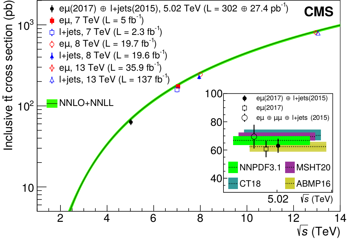
Figure 2: Inclusive t\bar{t} cross section in pp collisions as a function of the center-of-mass energy in the separate \ell +jets and dilepton channels along with the combined measurement at 5.02 TeV presented in this analysis are displayed. Some of the previous CMS measurements at \sqrt{s} = 7, 8 [6, 7], and 13 TeV [2, 11] are also shown. The NNLO+NNLL theoretical prediction [27] using the NNPDF3.1 [23] PDF set with \alpha_s(m_Z) = 0.118 and m_t = 172.5 GeV is shown in the main plot. In the inset, predictions at 5.02 TeV using the MSHT20 [48], CT18 [49], and ABMP16 [50] NNLO PDF sets, the latter with \alpha_s(m_Z) = 0.115 and m_t = 170.4 GeV, are compared, along with the NNPDF3.1 NNLO prediction, to the individual and combined results from this analysis. The vertical bars and bands represent the total uncertainties in the data and in the predictions, respectively. Points corresponding to measurements at the same \sqrt{s} are horizontally shifted for better readability.
