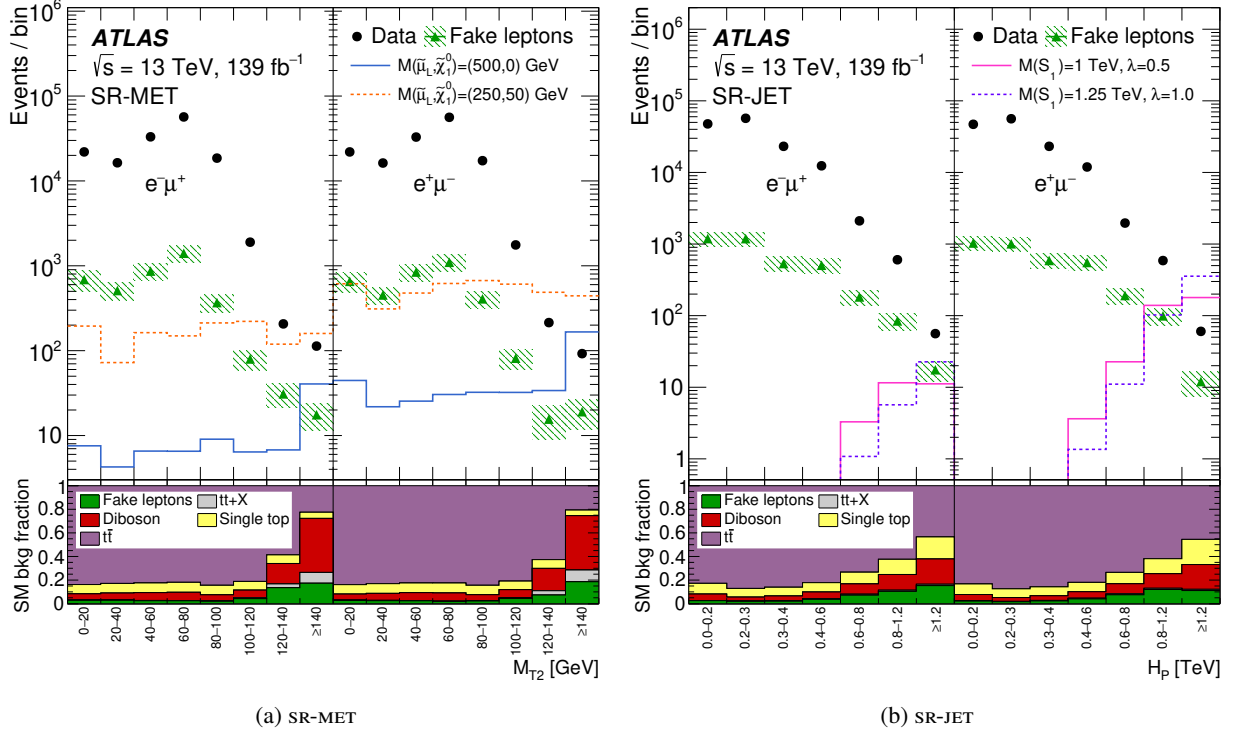
Figure 2: Distributions of data in the e^+ \mu^- and e^- \mu^+ channels of the general signal regions, binned in M_{T2} for SR-MET, and H_p for SR-JET, to correspond to the ratio measurement binning. The data has the muon charge and sagitta-bias corrections applied and corresponding uncertainties are added in quadrature in the error bar with the statistical uncertainty of the data. The fake-lepton background estimate is also shown, along with its uncertainty components added in quadrature, illustrating larger yields in the e^- \mu^+ channel as expected. The lower panel shows the fraction that each SM process contributes to the total SM background in each bin, estimated using standard MC simulations. The dominant background is t\bar{t} , whilst the importance of the fake-lepton background increases in higher bins of each variable. Benchmark RPV-supersymmetry signal models are shown for SR-MET, and benchmark scalar leptoquark models are shown for SR-JET, which all strongly favour the e^+ \mu^- final state over e^- \mu^+ , as expected.
