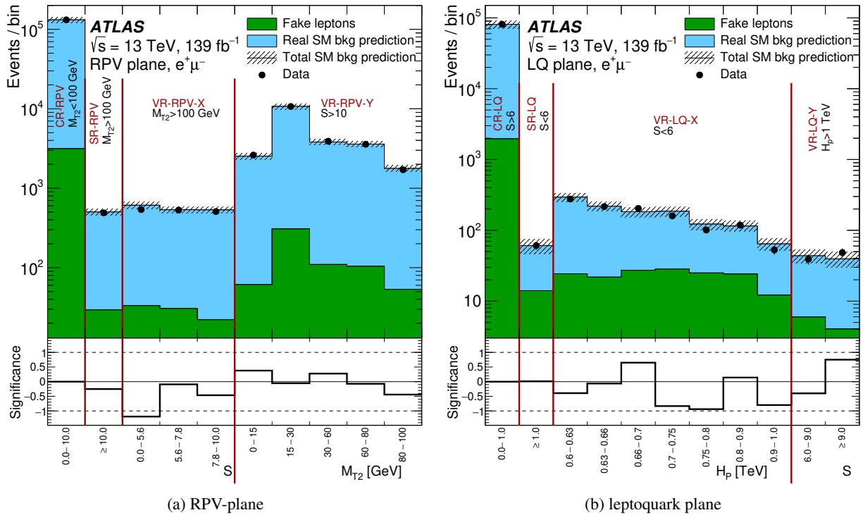
Figure 5: Distributions of data in the e^+\mu^- channel of the signal, control, and validation regions, used for the R -parity-violating supersymmetry model and leptoquark model limit fits. Note that ‘VR-LQ-x’ has a lower bound of H_p > 600 GeV, as it is not necessary to validate the ratio extrapolation any further away, kinematically, from the signal region. The data has the muon charge and sagitta-bias corrections applied. The fake-lepton background estimate and data-driven real SM background prediction derived from the fit are also shown. The sum of these is the total SM background estimate, and its error bar includes contributions from the fake-lepton background estimate, muon charge-bias and sagitta-bias uncertainties on the denominator data yields used to fit the SM background estimate. The lower panel shows the significance of any deviation between the observed data yields and total SM background prediction in each bin, defined in Ref. [52].
