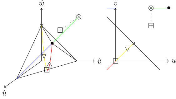
FIG. 2. Schematic correspondence between various interesting points and lines in the two-parameter three-point form factor space (right) and their images in the three-parameter six-point amplitude kinematic space (left) under the map (7)–(9). See Table I for the coordinates of the marked points.
