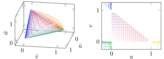
FIG. 1. Correspondence between various lines in the two-parameter three-point form factor space (right) and their images in the three-parameter six-point amplitude kinematic space (left) under the map (7)–(9). The white regions in the right plot map to points outside of the region 0 < \hat{u}, \hat{v}, \hat{w} < 1 in the left plot.
