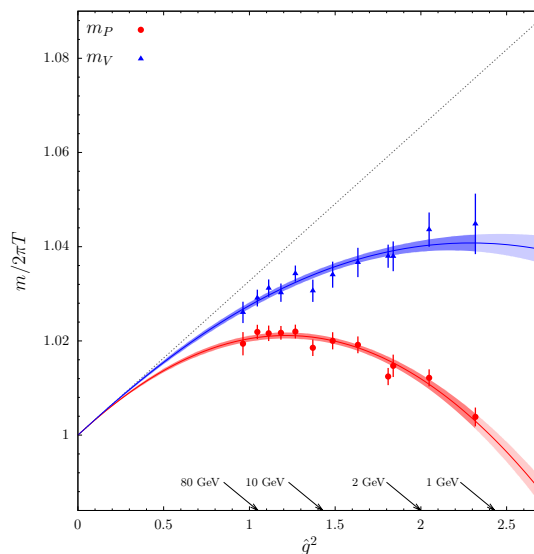
Figure 5. Pseudoscalar (red) and vector (blue) screening masses versus \hat{g}^2 . The bands represent the best fits in eqs. (7.2) and (7.4), while the dashed line is the analytically known contribution.
