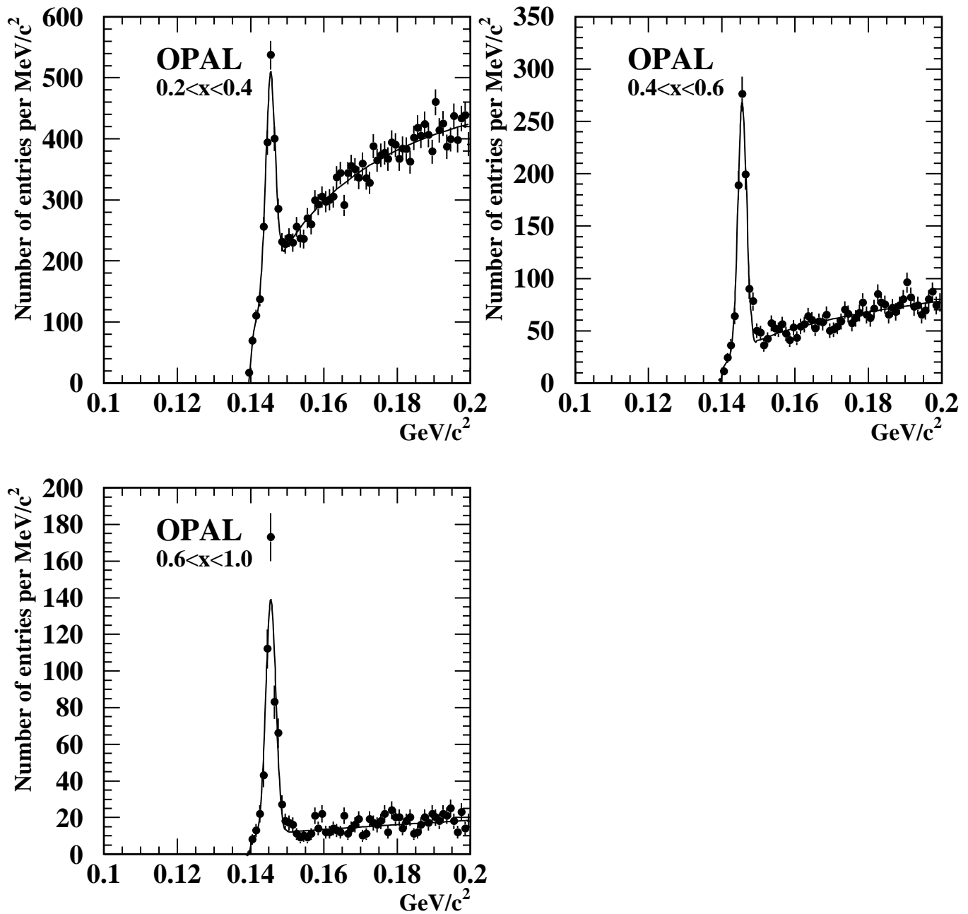
Figure 1: Distributions of the difference between the invariant mass of the D^* candidate and D^0 candidate in different x_{D^*} ranges. The points show the data while the solid lines are the results of the fits described in the text.
