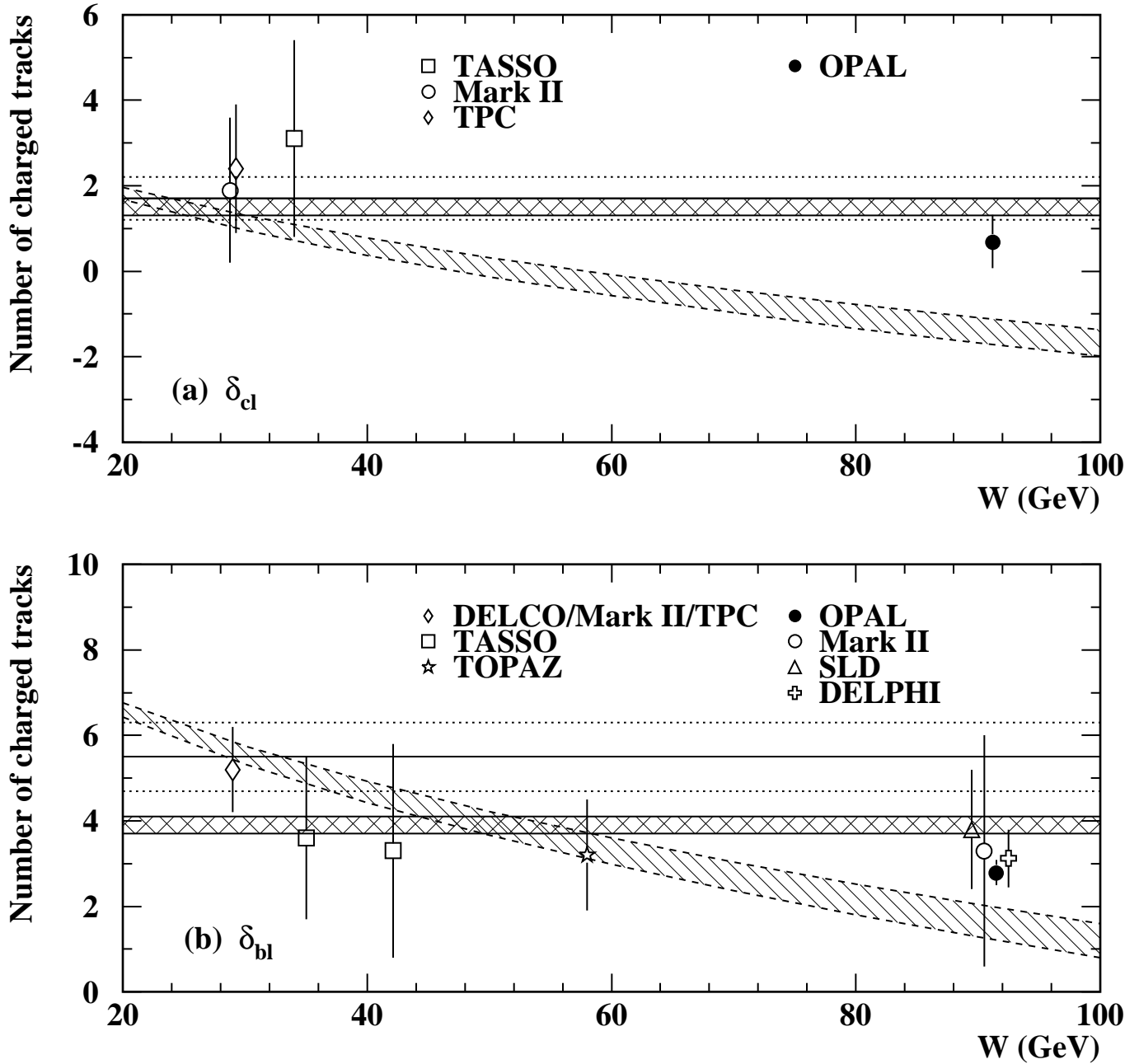
Figure 3: The difference in charged particle multiplicity between (a) c quark and light quark events, \delta_{cl} and (b) b quark and light quark events, \delta_{bl} , as a function of centre of mass energy. The single hatched areas represent the naive model while the cross hatched areas are the QCD upper limits as described in the text. The original MLLA predictions are shown as the solid lines with the dotted lines indicating the errors on these predictions not including higher order corrections. The data points around 91 GeV have been separated horizontally for clarity.
