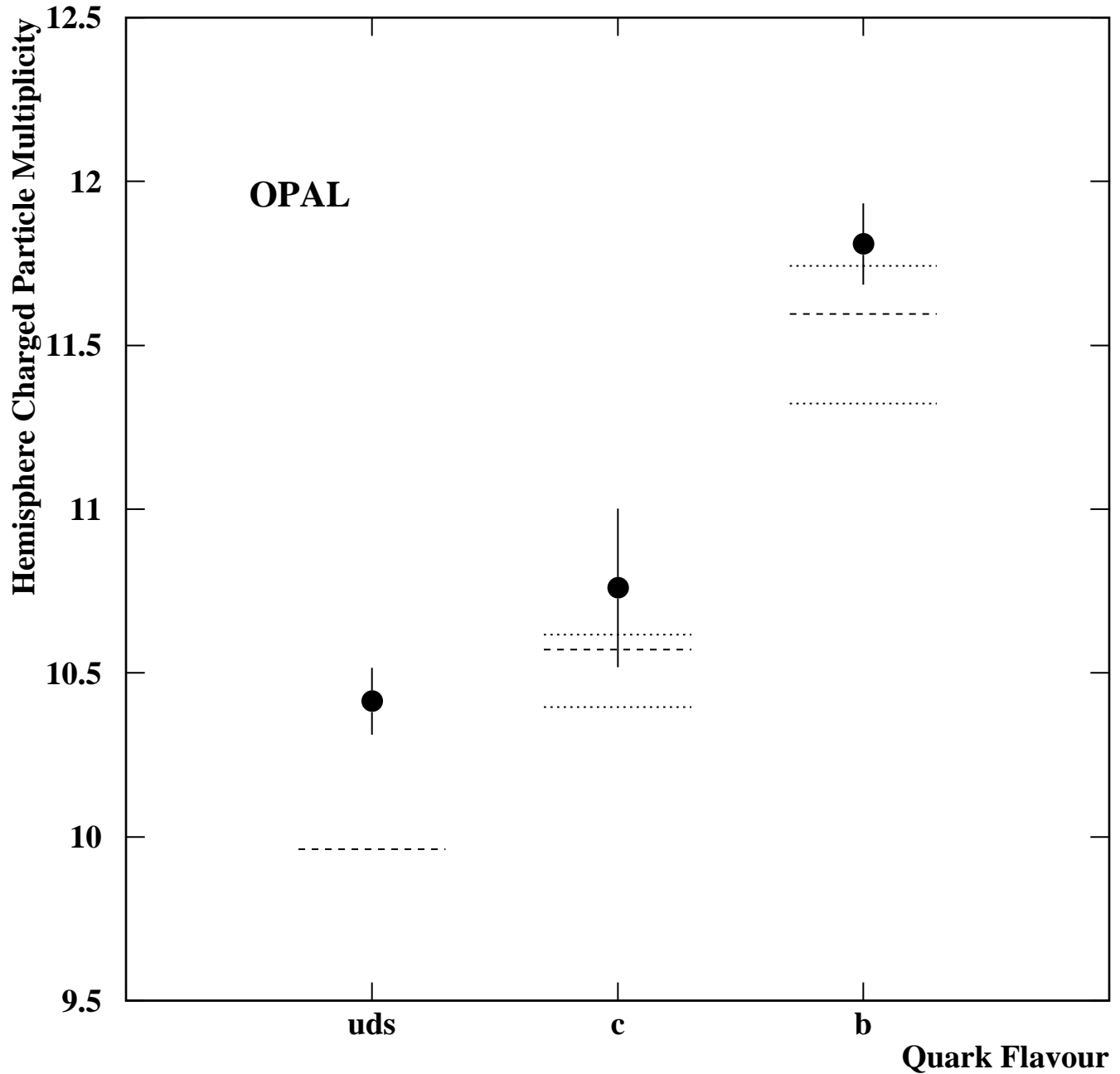
Figure 2: Values of the hemisphere charged particle multiplicities, \bar{n}_{uds} , \bar{n}_c and \bar{n}_b , obtained from the data. The error bars are the quadratic sum of the statistical and systematic errors but do not include the overall systematic scale uncertainty of 1.8%. The dashed horizontal lines are the predictions of Jetset 7.4 with the dotted lines reflecting the variation of the Peterson parameters \epsilon_c and \epsilon_b from 0.026 to 0.066 and 0.0025 to 0.0080 respectively; the multiplicity increases with \epsilon .
