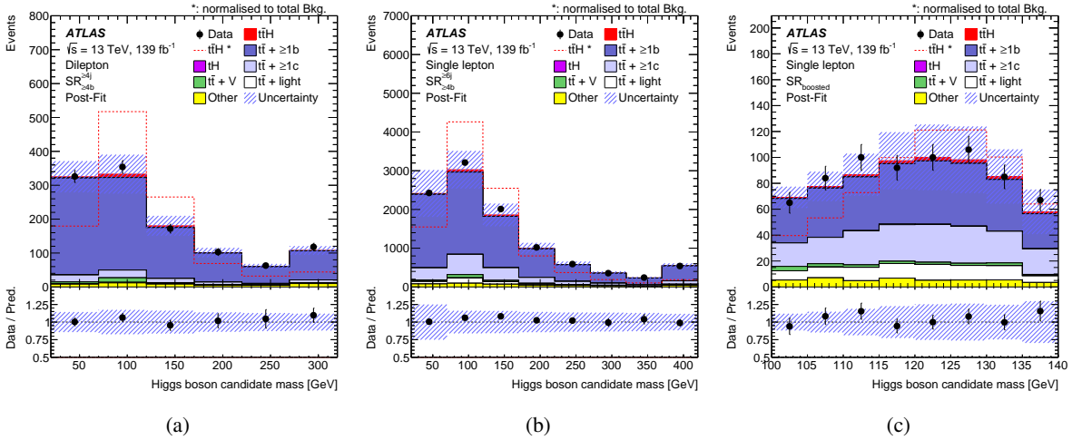
Figure 13: Post-fit distributions of the reconstructed Higgs boson candidate mass for the (a) dilepton SR_{\geq 4j}^{\geq 4b} , (b) single-lepton resolved SR_{\geq 4b}^{\geq 6j} and (c) single-lepton boosted SR_{\geq 4b}^{\text{boosted}} signal regions. The t\bar{t}H signal yield (solid red) is normalised to the fitted \mu value from the inclusive fit. The dashed line shows the t\bar{t}H signal distribution normalised to the total background prediction. The uncertainty band includes all uncertainties and their correlations. The first (last) bin includes the underflow (overflow).
