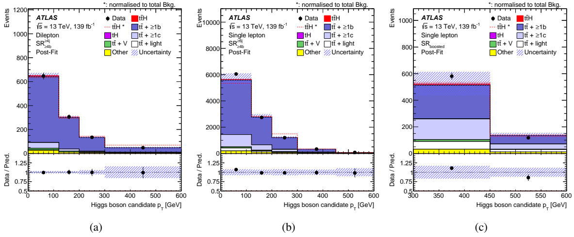
Figure 17: Post-fit distributions of the reconstructed Higgs boson candidate p_T^H for the (a) dilepton \text{SR}_{\ge 4b}^{\ge 6j} , (b) single-lepton resolved \text{SR}_{\ge 4b}^{\ge 6j} and (c) single-lepton boosted \text{SR}_{\text{boosted}} signal regions. The t\bar{t}H signal yield (solid red) is normalised to the fitted \mu value from the inclusive fit. The dashed line shows the t\bar{t}H signal distribution normalised to the total background prediction. The uncertainty band includes all uncertainties and their correlations. The last bin includes the overflow.
