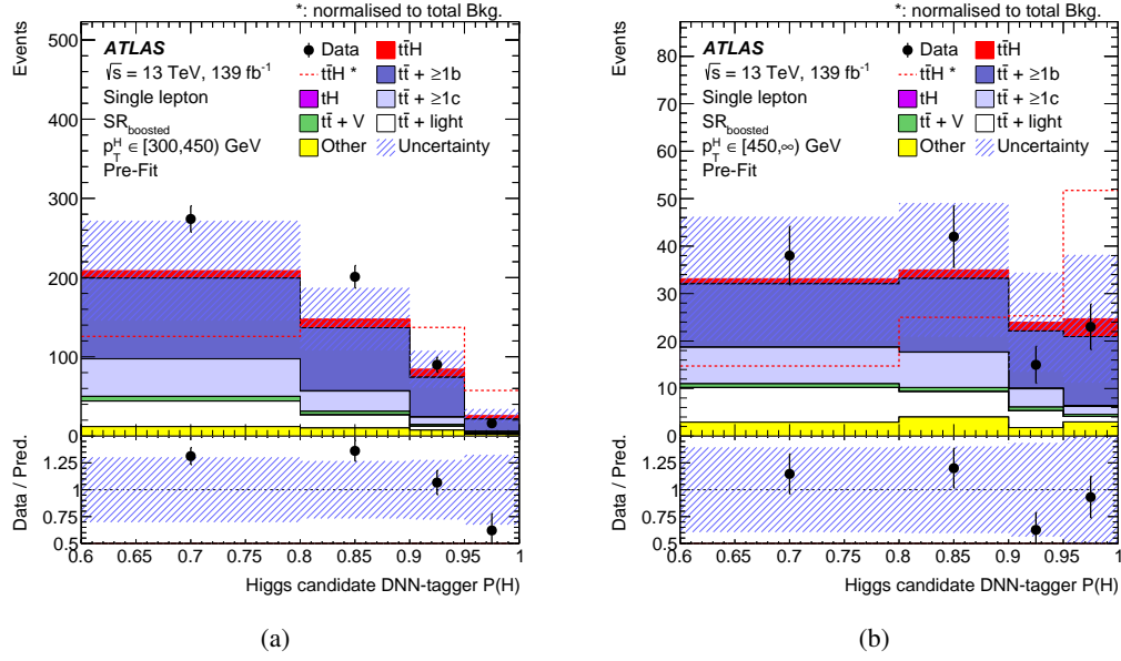
Figure 2: Comparison between data and prediction for the DNN P(H) output for the Higgs boson candidate prior to any fit to the data in the single-lepton boosted channel for (a) 300 \leq p_T^H < 450 GeV and (b) p_T^H \geq 450 GeV. The dashed line shows the t\bar{t}H signal distribution normalised to the total background prediction. The uncertainty band includes all uncertainties and their correlations.
