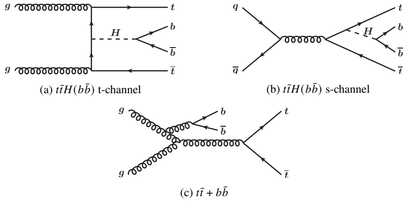
Figure 1: Representative tree-level Feynman diagrams for the production of a Higgs boson in association with a top-quark pair ( t\bar{t}H ) in (a) the t-channel and (b) the s-channel and the subsequent decay of the Higgs boson into b\bar{b} , and for (c) the main t\bar{t} + b\bar{b} background.
