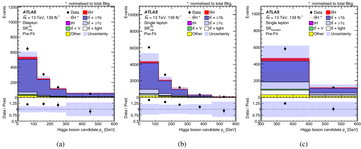
Figure 4: Pre-fit distributions of the reconstructed Higgs boson candidate p_T^H for the (a) dilepton \text{SR}_{\ge 4b}^{\ge 6j} , (b) single-lepton resolved \text{SR}_{\ge 4b}^{\ge 6j} and (c) single-lepton boosted \text{SR}_{\text{boosted}} signal regions. The dashed line shows the t\bar{t}H signal distribution normalised to the total background prediction. The uncertainty band includes all uncertainties and their correlations, except for the uncertainty in the k(t\bar{t} + \ge 1b) normalisation factor which is not defined pre-fit. The last bin includes the overflow.
