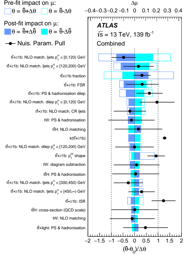
Figure 15: Ranking of the 20 nuisance parameters with the largest post-fit impact on \mu in the fit. Nuisance parameters corresponding to statistical uncertainties in the simulated event samples are not included. The empty blue rectangles correspond to the pre-fit impact on \mu and the filled blue ones to the post-fit impact on \mu , both referring to the upper scale. The impact of each nuisance parameter, \Delta\mu , is computed by comparing the nominal best-fit value of \mu with the result of the fit when fixing the considered nuisance parameter to its best-fit value, \hat{\theta} , shifted by its pre-fit (post-fit) uncertainties \pm\Delta\theta ( \pm\Delta\hat{\theta} ). The black points show the pulls of the nuisance parameters relative to their nominal values, \theta_0 . These pulls and their relative post-fit errors, \Delta\hat{\theta}/\Delta\theta , refer to the lower scale. The ‘ljets’ (‘dilep’) label refers to the single-lepton (dilepton) channel.
