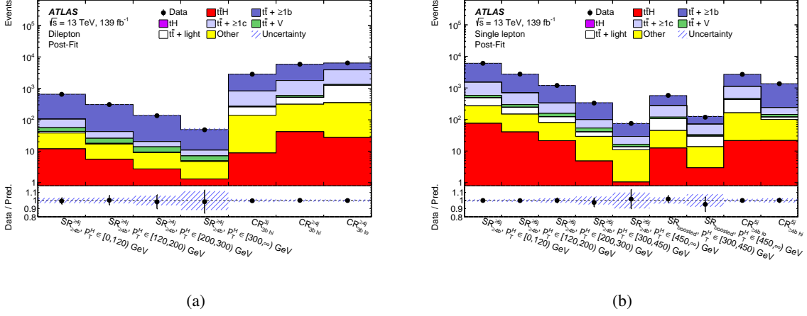
Figure 5: Comparison of predicted and observed event yields in each of the control and signal regions in the (a) dilepton and (b) single-lepton channels after the fit to the data. The uncertainty band includes all uncertainties and their correlations.
