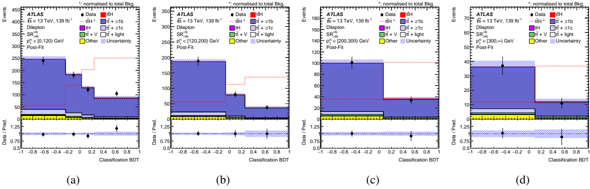
Figure 6: Comparison between data and prediction for the BDT discriminant in the dilepton SRs after the inclusive fit to the data, for (a) 0 \leq p_T^H < 120 \text{ GeV} , (b) 120 \leq p_T^H < 200 \text{ GeV} , (c) 200 \leq p_T^H < 300 \text{ GeV} and (d) p_T^H \geq 300 \text{ GeV} . The t\bar{t}H signal yield (solid red) is normalised to the fitted \mu value from the inclusive fit. The dashed line shows the t\bar{t}H signal distribution normalised to the total background prediction. The uncertainty band includes all uncertainties and their correlations.
