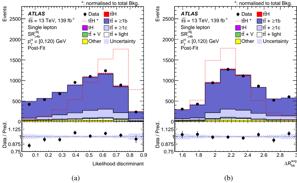
Figure 11: Comparison between data and prediction for (a) the likelihood discriminant, and (b) the average \Delta R for all possible combinations of b -tagged jet pairs, after the inclusive fit to the data in the single-lepton resolved channel for 0 \leq p_T^H < 120 GeV. The t\bar{t}H signal yield (solid red) is normalised to the fitted \mu value from the inclusive fit. The dashed line shows the t\bar{t}H signal distribution normalised to the total background prediction. The uncertainty band includes all uncertainties and their correlations.
