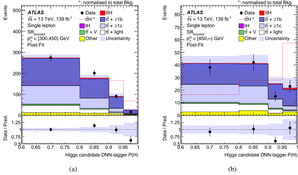
Figure 12: Comparison between data and prediction for the DNN P(H) output for the Higgs boson candidate after the inclusive fit to the data in the single-lepton boosted channel for (a) 300 \leq p_T^H < 450 GeV and (b) p_T^H \geq 450 GeV. The t\bar{t}H signal yield (solid red) is normalised to the fitted \mu value from the inclusive fit. The dashed line shows the t\bar{t}H signal distribution normalised to the total background prediction. The uncertainty band includes all uncertainties and their correlations.
