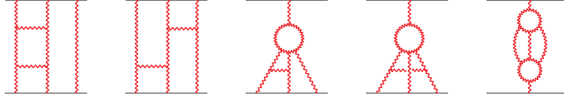
Figure 4: Representation of transitions involving Multi-Reggeon States (MRS), which contribute to the odd-signature amplitude at four loops.
