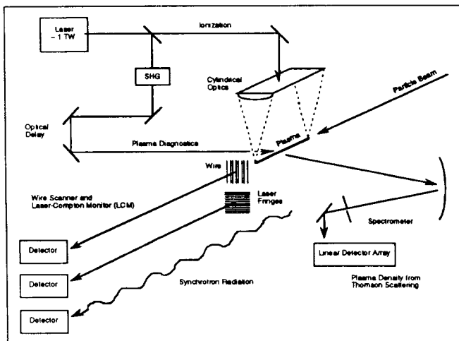
Figure 1: Outline of Plasma Lens Experimental Setup
