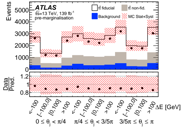
Figure 5: Comparison of data to the prior prediction for the \Delta E vs. \theta_j distribution used in the unfolding. The 3 differential bins in \theta_j and 4 \Delta E bins are concatenated to give 12 bins as shown in Figure 3. The shaded red bands correspond to the total uncertainty of the prediction.
