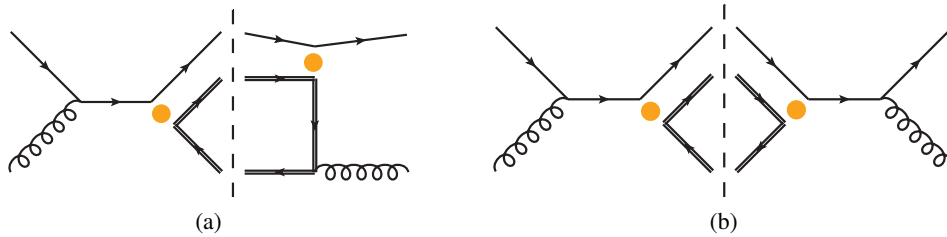
Figure 1: Examples of contributions to the energy asymmetry in terms of Feynman diagrams. The double lines indicate top quarks; the orange filled circles stand for possible insertions of four-quark operators in SMEFT. The dashed line symbolizes the interference \mathcal{M}_1 \mathcal{M}_2^* of the two qg \rightarrow t\bar{t}q amplitudes \mathcal{M}_1 and \mathcal{M}_2^* to its left and right sides. Contributions to the asymmetry in QCD are obtained by replacing the orange filled circles in the left diagram by gluons. Further details about the QCD prediction and SMEFT contributions can be found in Ref. [18] and Ref. [19], respectively.
