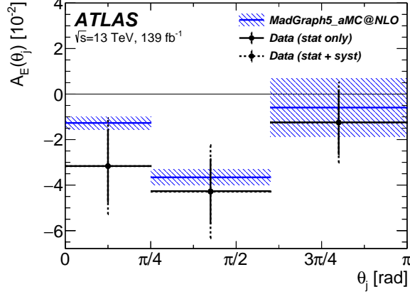
Figure 7: Data Measurements (black points with errors) and predictions (blue lines) of the energy asymmetry in three bins of the jet angle \theta_j . The SM prediction was obtained from simulations of t\bar{t}j events with MADGRAPH5_AMC@NLO + PYTHIA 8 at NLO in QCD for t\bar{t}j + PS, including MC statistical and scale uncertainties (blue shaded bands) as described in Section 5.1.
