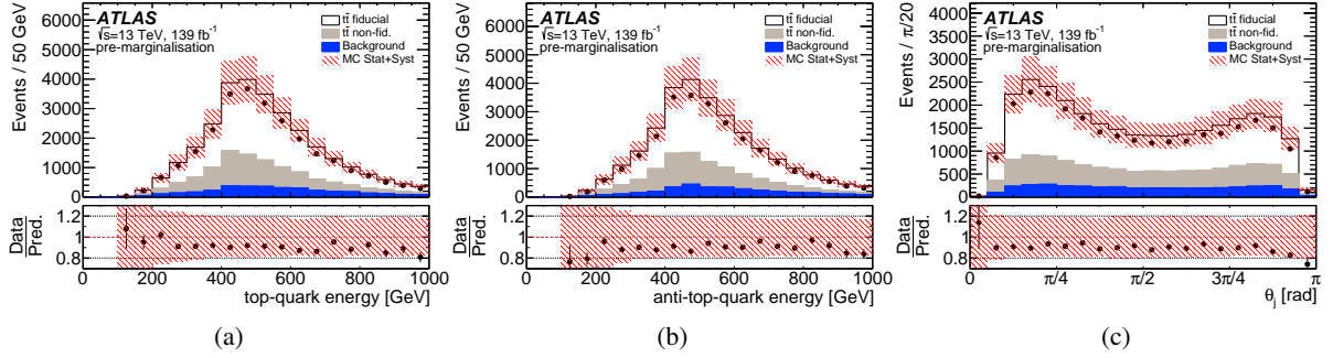
Figure 2: Comparison of observed data with the predicted distribution of (a) the top-quark energy, (b) the antitop-quark energy, and (c) the angle \theta_j . The expectations for the t\bar{t} fiducial and non-fiducial signal are represented by the white and grey areas, respectively, while all non- t\bar{t} backgrounds are added up in the blue area. The shaded red bands correspond to the total uncertainty of the prediction, while the statistical uncertainty on the data is indicated by the black error bars, that are mostly smaller than the size of the marker.
