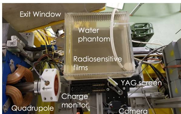
Figure 1: The experimental setup for the focusing VHEE experiments in CLEAR. The water phantom is mounted on a movable stage, to allow for several irradiations between accesses and in-air beam size measurements by the YAG screen.
