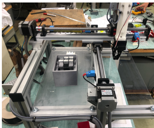
Figure 2: Robotic system to pick and place the samples.
