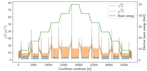
Figure 2: Representation of the beta functions and the beam energy along the multi-turn ERL operation.
