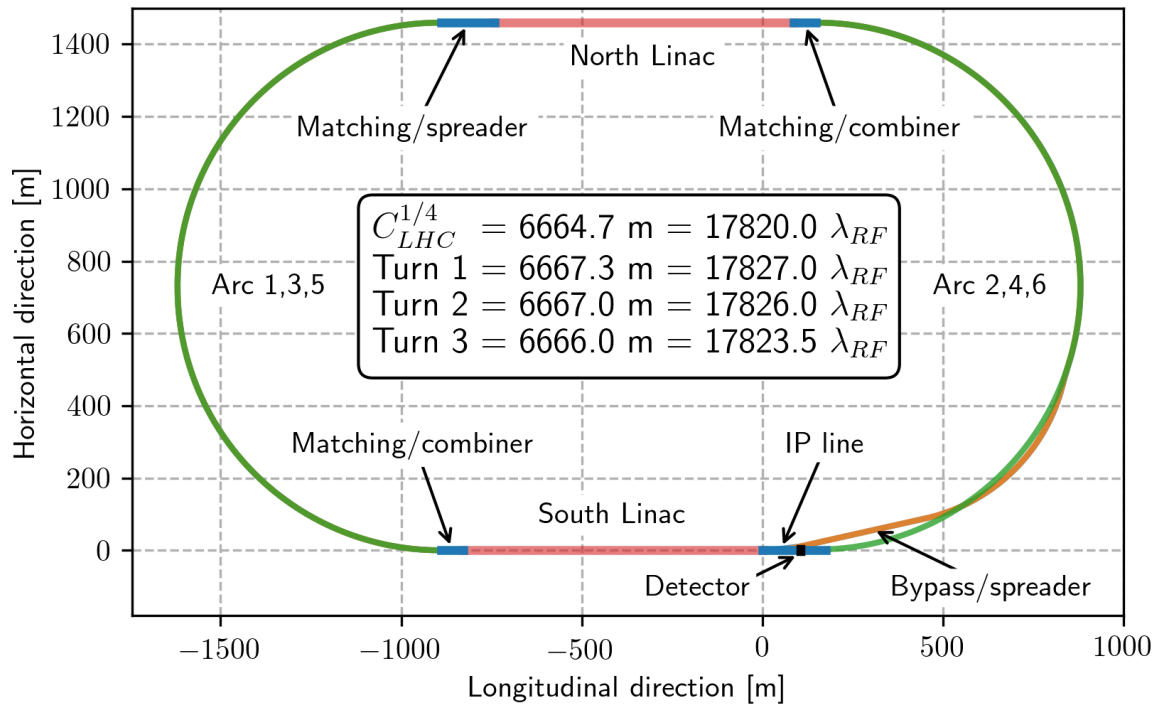
Figure 1: Layout for the 1/4 LHC circumference ERL representing the different sections composing the machine.
