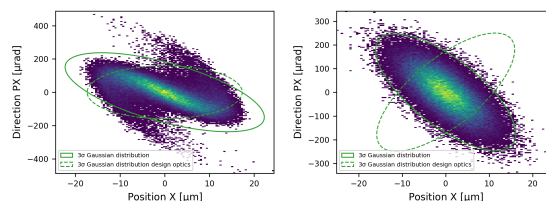
Figure 4: Phase space electrons distribution post collision. Left: Optical matching with HL-LHC proton beam. Right: Luminosity optimum settings.
