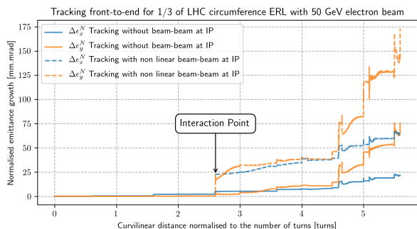
Figure 3: Emittance growth along the curvilinear coordinate for the 1/3 of LHC circumference ERL design.
