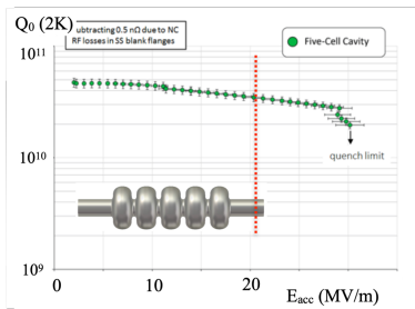
Figure 2: Q-parameter of the 5 cell cavity prototype.
