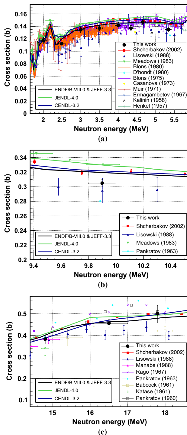
Fig. 7 Cross-section results from this work (black points) along with the experimental data available in EXFOR [5] and the latest evaluated libraries ENDF/B-VIII.0 [32] (which agrees with JEFF-3.3 [40]) (black line), JENDL-4.0 [41] (green line) and CENDL-3.2 [42] (blue line) at a the energy region from 2.0 to 5.3 MeV, b 9.9 MeV and c at the energy region from 14.8 to 17.8 MeV
