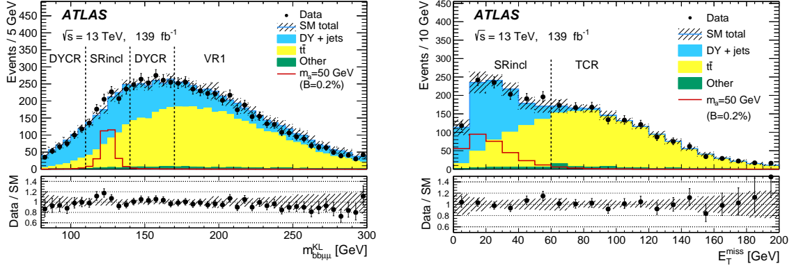
Figure 4: Post-fit m_{bb\mu\mu}^{KL} in DYCR, SRincl and VR1 (left); E_T^{\text{miss}} in SRincl and TCR (right). No selection based on the BDT discriminants is applied in the analysis regions shown in the figures. The signal distributions are normalized to the SM Higgs boson cross-section (including ggF, VBF, and VH production) and assume \mathcal{B}(H \rightarrow aa \rightarrow bb\mu\mu) as indicated in the legends of the figures (chosen to ensure good visibility in the plot). The hatched bands show the total post-fit statistical and systematic uncertainties of the backgrounds. The histogram labeled as “Other” in the legend includes the contributions from the diboson, single-top-quark, t\bar{t}+V and W +jets backgrounds.
