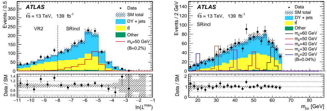
Figure 5: Post-fit \ln(L^{\text{max}}) in VR2 and SRincl (left); m_{\mu\mu} in SRincl (right). No selection based on the BDT discriminants is applied in the analysis regions shown in the figures. The signal distributions are normalized to the SM Higgs boson cross-section (including ggF, VBF, and VH production) and assume \mathcal{B}(H \rightarrow aa \rightarrow bb\mu\mu) as indicated in the legends of the figures (chosen to ensure good visibility in the plot). The hatched bands show the total post-fit statistical and systematic uncertainties of the backgrounds. The histogram labeled as “Other” in the legend includes the contributions from the diboson, single-top-quark, t\bar{t}+V and W +jets backgrounds.
