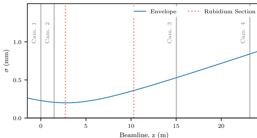
Figure 2. The standard deviation of the transverse proton bunch profile versus the beamline position for nominal bunch parameters without plasma. Gray solid lines show positions of four beam observation systems. The position of the plasma section is shown by red dotted lines.
