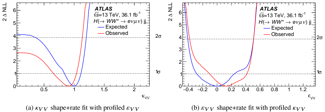
Figure 9: Likelihood scans over (a) \kappa_{VV} and (b) \varepsilon_{VV} , with the other parameter profiled. The fits are performed using both shape and rate information. All relevant experimental and theoretical systematic uncertainties are considered in the fits.
