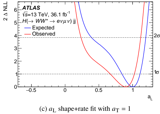
Figure 8: Likelihood scans over the transversely (a, b) and longitudinally (c) polarised couplings. Fits using shape-only (a) and shape+rate (b, c) information are shown. All relevant experimental and modelling systematic uncertainties are considered in the fits.
