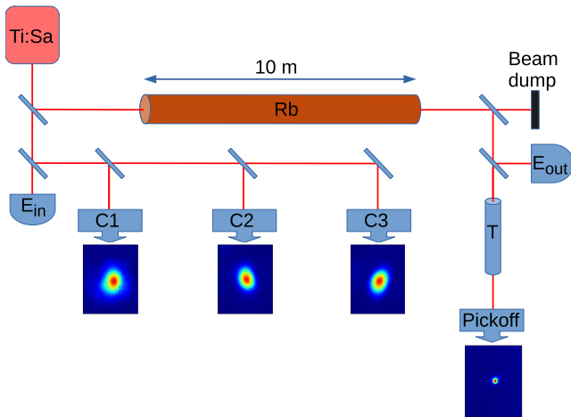
FIG. 1. Sketch of the experimental setup. E_{in} and E_{out} are the input and output energy meters, respectively. Cameras in the virtual laser line correspond to the vapor chamber entrance (C1), center (C2) and exit (C3). Transmitted light distribution is detected by the pickoff camera after the imaging telescope (T). Images below the cameras are illustrative images from a single pulse measurement. Optical paths are not drawn to scale, the optical path from the final focusing telescope of the Ti:Sa laser to the vapor source entrance (and the C1 camera) is \approx 40 m.
