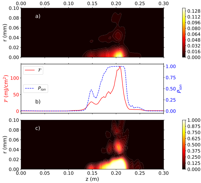
FIG. 11. The propagation and self-focusing of a low energy, E_{in} = 0.04 mJ pulse of parameter set C). a) fluence \mathcal{F}(r, z) , b) on-axis fluence \mathcal{F}(r = 0, z) and ionization probability P_{ion}(r = 0, z) and c) ionization probability P_{ion}(r, z) .
