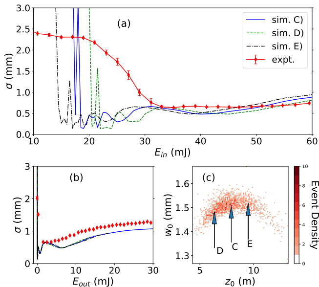
FIG. 10. (a) Transmitted beam width vs. input pulse energy for the original simulation C) and the two simulations with modified Gaussian beam parameters D) and E). Binned experimental data with error of the mean is also plotted. (b) The same quantities plotted with respect to the transmitted pulse energy. (c) 2D histogram of the input beam parameters obtained for \mathcal{N} = 6.6 \cdot 10^{14} \text{ cm}^{-3} density shots with arrows pointing to the mean values C) and perturbed parameter simulation values D) and E).
