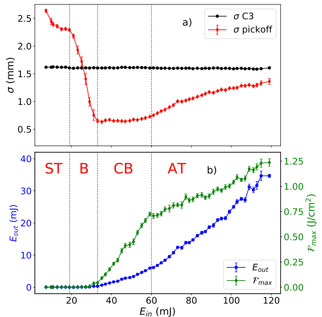
FIG. 3. a) Width parameter \sigma for transmitted pulse and virtual exit camera image as a function of input pulse energy for \mathcal{N} = 6.6 \cdot 10^{14} \text{cm}^{-3} vapor density shots. b) Transmitted laser pulse energy (left axis) and peak fluence (right axis). The points depict averages of binned data, error bars mark the error of the mean. Vertical dotted lines mark the approximate domain boundaries, which are labeled as: ‘ST’ for sub-threshold domain, ‘B’ for breakthrough domain, ‘CB’ for confined beam domain and ‘AT’ for asymptotic transparency domain.
