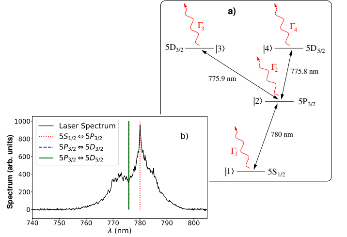
FIG. 5. a) Electronic levels of the rubidium atom that are included in the model and their numbering. Three excited states are resonantly accessible from the ground state, ionization leads to level loss from each of the levels. b) Measured spectrum of the ionizing laser oscillator before amplification and interaction with the vapor. The resonance wavelengths included in the model are marked, lines 5P_{3/2} \leftrightarrow 5D_{3/2} and 5P_{3/2} \leftrightarrow 5D_{5/2} are a closely spaced doublet, difficult to resolve on this scale.
