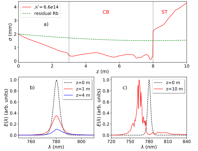
FIG. 12. The propagation of a E_{in} = 16 mJ pulse for simulation parameter set C). a) Beam width \sigma as a function of propagation distance z . Vertical dotted lines delimit the regions that can be associated with the confined-beam (CB) and sub-threshold (ST) domains. Dashed line marks the width parameter w(z) for the unperturbed Gaussian beam. b) Pulse energy spectrum at the vapor entrance z = 0 m and at z = 1 m inside the vapor, drawn to scale. c) Normalized pulse energy spectrum at the two ends of the vapor source, z = 0 m and z = 10 m.
