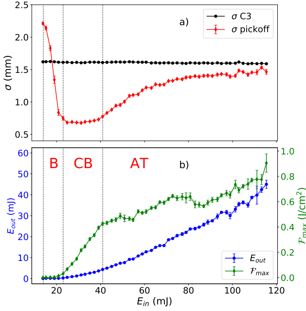
FIG. 4. Plot identical to Fig. 3 for \mathcal{N} = 4.895 \cdot 10^{14} \text{ cm}^{-3} vapor density shots. The sub-threshold domain is not captured by the dataset.
