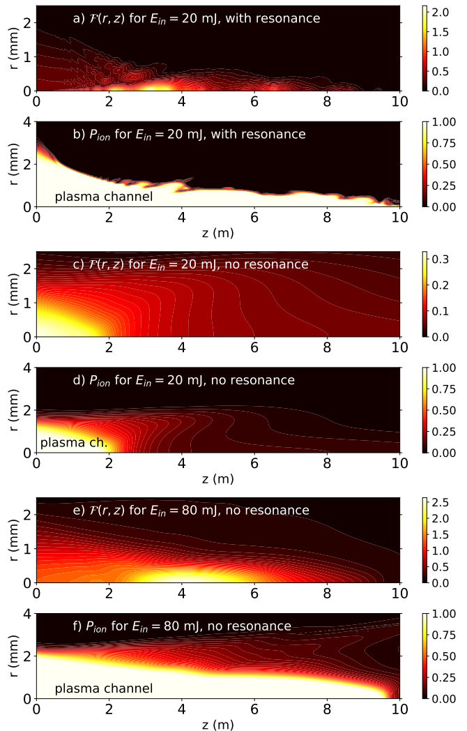
FIG. 8. Pulse fluence (in \text{J}/\text{cm}^2 ) and atomic ionization probability profiles as a function of propagation distance z and transverse radius r . a) \mathcal{F}(r, z) and b) P_{ion} from full theory with resonance E_{in} = 20 mJ pulse. c) \mathcal{F}(r, z) and d) P_{ion} reduced theory calculation, E_{in} = 20 mJ pulse. e) \mathcal{F}(r, z) and f) P_{ion} reduced theory calculation, E_{in} = 80 mJ pulse. Data was taken from simulation set C). ‘Plasma channel’ marks area with complete conversion to \text{Rb}^{1+} ions near axis.
