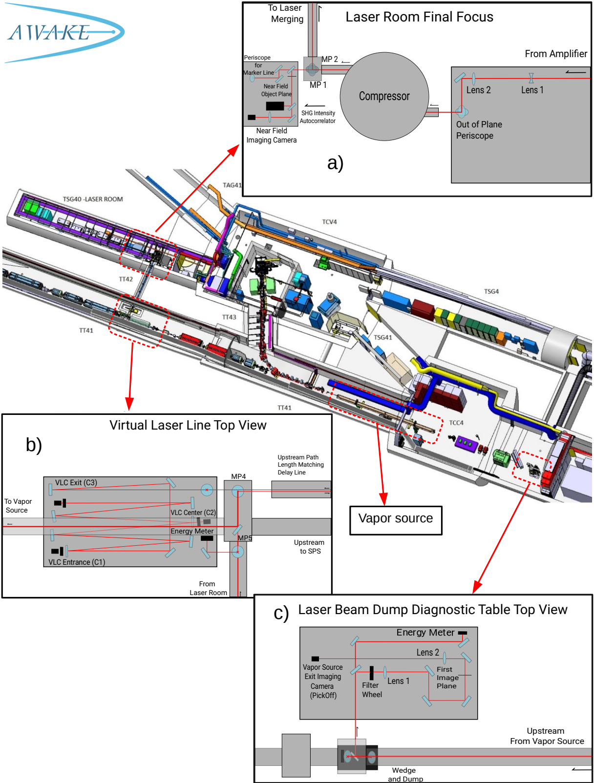
FIG. 1. Figure of the AWAKE experimental area at CERN with the location of the various components of the experiment indicated and details of each area shown in the subfigures. a) Laser room with compressor and final focus. b) Laser and proton beam merging point with the virtual laser line setup. c) Laser beam dump diagnostic table with the pickoff camera and output energy meter.
