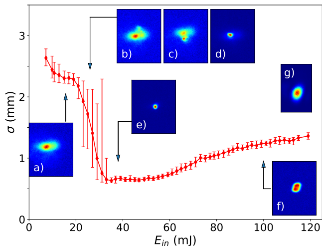
FIG. 2. Width parameter \sigma from Gaussian fit for transmitted laser pulses, \mathcal{N} = 6.6 \cdot 10^{14} \text{cm}^{-3} . Mean values of binned data shown with asymmetric standard deviation indicated. Insets depict pickoff camera images for selected shots with: a) E_{in} = 15.6 mJ, b)-d) E_{in} = 26 mJ, e) E_{in} = 38 mJ and f) E_{in} = 100 mJ, each also marked by the arrows. Aspect ratio of the insets corresponds to the detector physical aspect ratio, color coding of individual images are unique, scaled to individual image maxima. Inset g) depicts the virtual exit camera image (C3) for E_{in} = 38 mJ, drawn to the same spatial scale.
