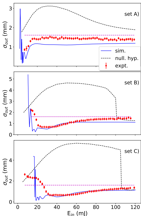
FIG. 7. Transmitted beam width vs. input pulse energy for the measurements and corresponding simulations. Labels A)-C) correspond to the parameter set labels of table I. Solid blue line: simulation with atomic resonances, dashed black line: reduced theory simulation (no resonances), red symbols: binned experimental data averages with error bars showing error of the mean (mostly smaller in size than the symbol marking the points). Dashed horizontal line marks the beam width measured on the virtual exit camera C3.
