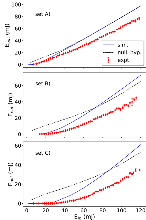
FIG. 6. Transmitted pulse energy vs. input pulse energy for the measurements and the corresponding simulations. Labels A)-C) correspond to the parameter set labels of table I. Solid blue line: simulation with atomic resonances, dashed black line: reduced theory simulation (no resonances), red symbols: binned experimental data averages with error bars showing error of the mean (mostly smaller in size than the symbol marking the points).
