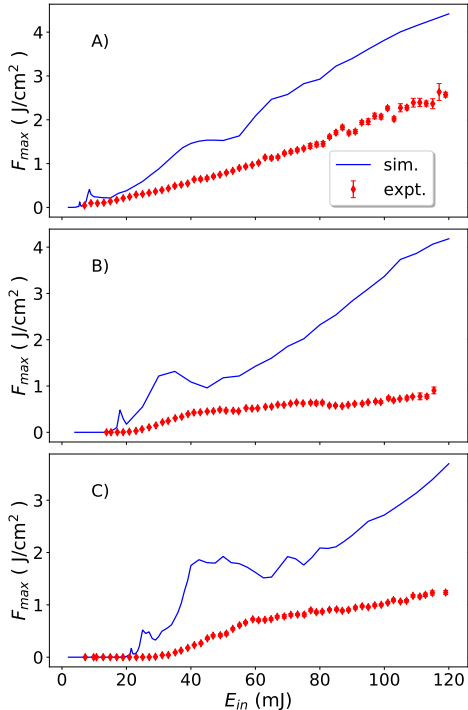
FIG. 9. Transmitted pulse on-axis fluence in \text{J}/\text{cm}^2 as a function of input energy for the three simulation series. Labels A)-C) correspond to the parameter set labels of table I. Solid blue line: simulation, red symbols: binned experimental data averages with error bars showing error of the mean (mostly smaller in size than the symbol marking the points).
