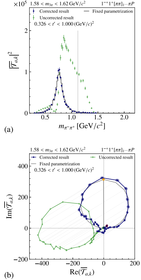
FIG. 14. Similar to Fig. 6 but showing the effect of resolving the zero-mode ambiguity in the 1^{-+}1^+[\pi\pi]_{1-\pi P} wave using, as an example, the highest t' bin and an m_{3\pi} bin in the \pi_1(1600) resonance region. (a) shows the intensity distribution and (b) the corresponding Argand diagram as a function of m_{\pi^-\pi^+} . The green data points correspond to the set \{\mathcal{T}_k^{\text{fit}}\} of binned transition amplitudes [defined in Eqs. (7) and (9)] as extracted in the freed-isobar PWA. The blue data points represent the transition amplitudes \{\mathcal{T}_k^{\text{fit}} - \mathfrak{C}\tilde{\Delta}_k\} after resolving the zero-mode ambiguity by minimizing Eq. (B17). The upper limit m_{\pi^-\pi^+} = 1.12 \text{ GeV}/c^2 of the range used in this minimization is indicated by the vertical line in (a). The gray histogram represents the \rho(770) Breit-Wigner amplitude used to resolve the zero-mode ambiguity. In the Argand diagram, corresponding green and blue data points are connected by gray lines representing the \{\mathfrak{C}\tilde{\Delta}_k\} values.
