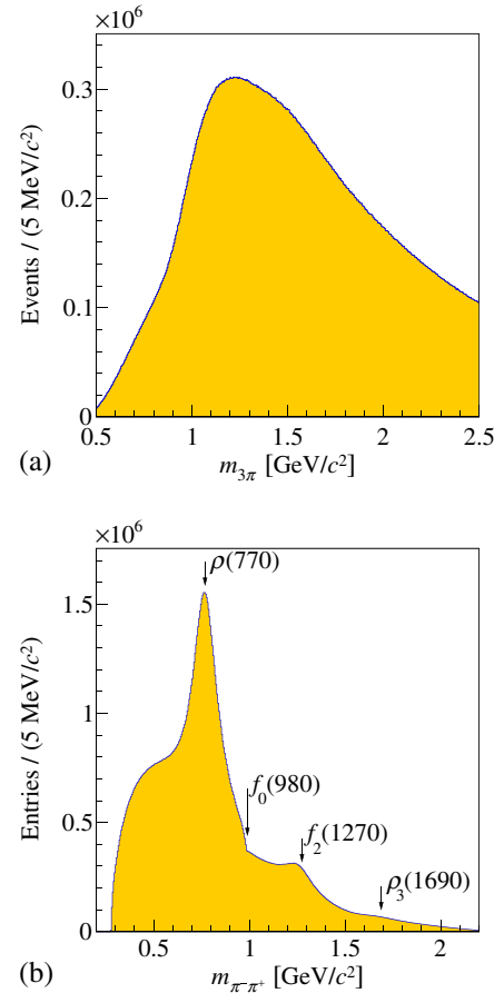
FIG. 11. (a) \pi^-\pi^-\pi^+ invariant mass spectrum for the Deck Monte Carlo sample. (b) invariant mass distribution of the \pi^-\pi^+ subsystem (two entries per event). The arrows indicate 2\pi resonances included in the Deck model.
