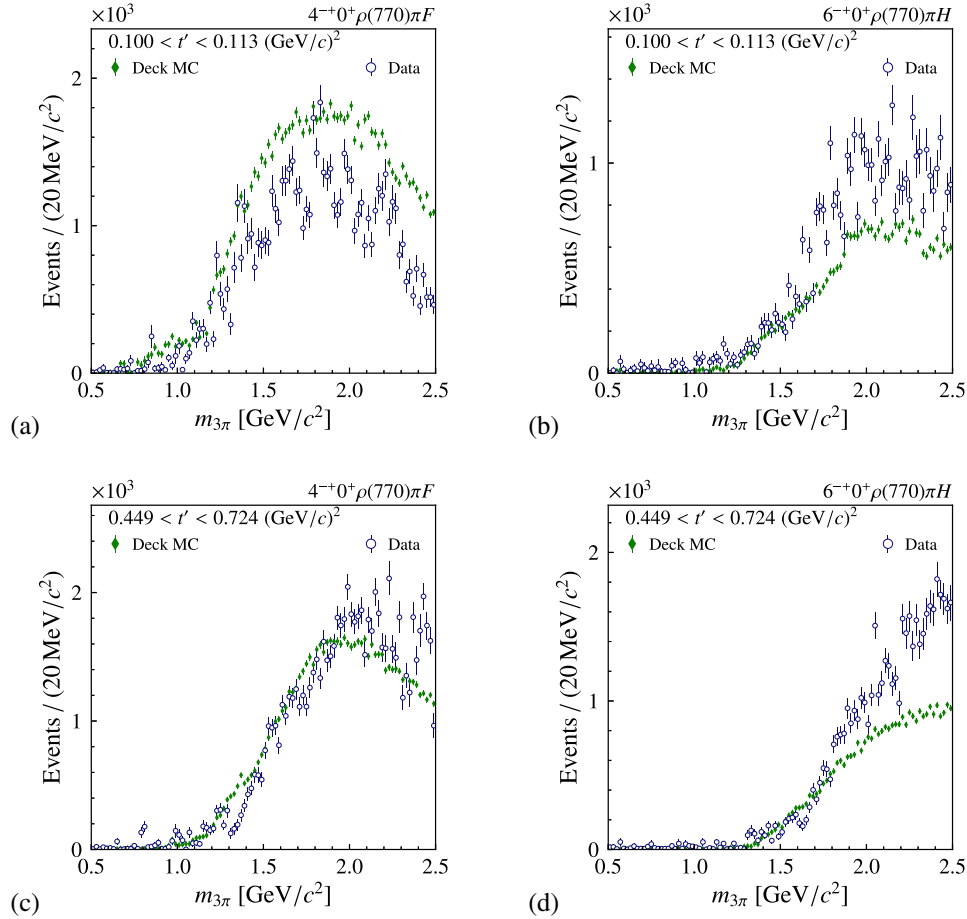
FIG. 12. Intensity distributions of the 4^{-+}0^+\rho(770)\pi F wave (left column) and the 6^{-+}0^+\rho(770)\pi H wave (right column) for two t' bins as obtained from the 88-wave PWA. The real data are represented by the blue data points; the Deck pseudodata by the green data points. The pseudodata are normalized using a common factor for all waves (see text for details).
