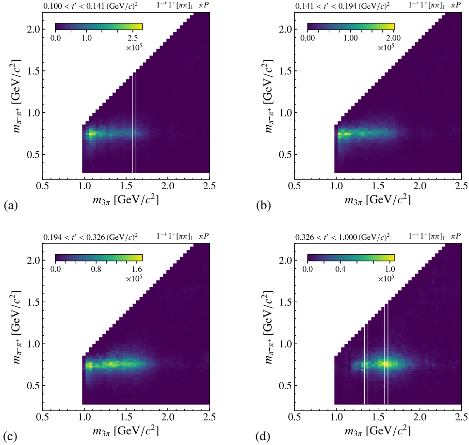
FIG. 5. Two-dimensional intensity distribution of the 1^{-+}1^{+}[\pi\pi]_{1^{-}}\pi P wave obtained in the freed-isobar PWA (after correction for the zero mode) as a function of m_{3\pi} and m_{\pi^{-}\pi^{+}} for all four t' bins. The color scale represents the intensity in units of number of events per 40 MeV/ c^2 interval in m_{\pi^{-}\pi^{+}} and in m_{3\pi} . The white vertical lines indicate the m_{3\pi} bins shown in Fig. 6.
