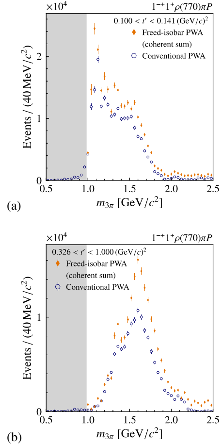
FIG. 8. Comparison of the m_{3\pi} intensity distributions of the 1^{-+}1^+[\pi\pi]_{1--}\pi P wave from the freed-isobar PWA (orange data points) and of the 1^{-+}1^+\rho(770)\pi P wave from the conventional PWA (blue data points). For the former, the intensities are calculated by coherently summing the contributions from all m_{\pi^-\pi^+} intervals. (a) shows the lowest and (b) the highest t' bin. The shaded m_{3\pi} range is excluded from the freed-isobar PWA.
