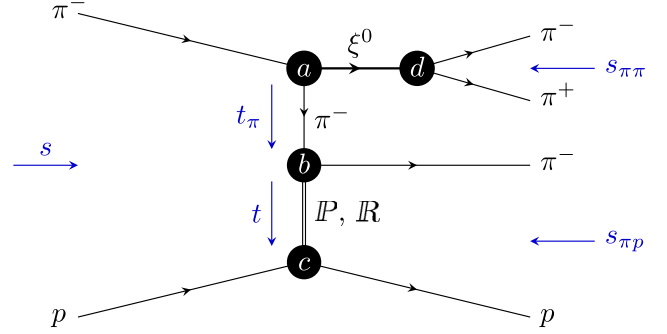
FIG. 10. Schematic diagram of the Deck process with the relevant kinematic variables.
