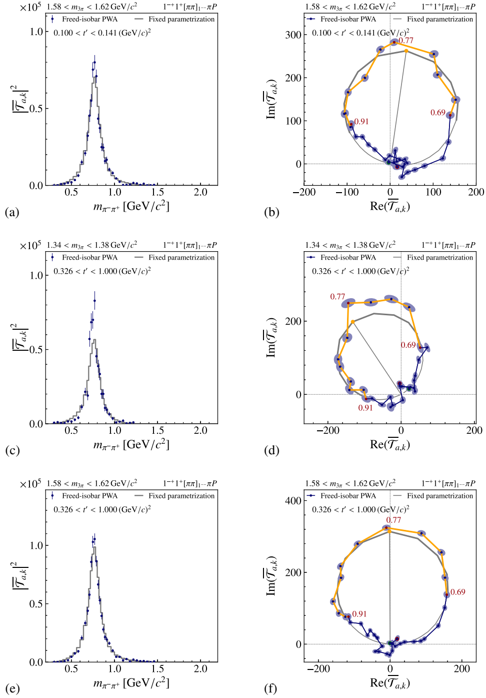
FIG. 6. The [\pi\pi]_{1--} dynamic isobar amplitude in the 1^{-+}1^{+}[\pi\pi]_{1--}\pi P wave as a function of m_{\pi^{-}\pi^{+}} for selected m_{3\pi} and t' bins. Left column: intensities; right column: Argand diagrams. The blue data points with error bars or error ellipses, respectively, are the result of the freed-isobar PWA corrected for the zero mode. In the Argand diagrams, the data points are connected by lines to indicate the order and the red numbers correspond to m_{\pi^{-}\pi^{+}} values in \text{GeV}/c^2 . The line segments highlighted in orange correspond to the m_{\pi^{-}\pi^{+}} range from 0.64 to 0.92 \text{GeV}/c^2 around the \rho(770) . The overall phase of the Argand diagrams is fixed by the 4^{++}1^{+}\rho(770)\pi G wave. For comparison, the fixed parametrization of the dynamic isobar amplitude for the \rho(770) as used in the conventional PWA is shown by the gray lines with the \rho(770) region indicated by thicker lines. In the Argand diagrams, the orange point indicates the nominal \rho(770) mass and the green- and red-circled points indicate the lowest and the highest m_{\pi^{-}\pi^{+}} interval, respectively.
