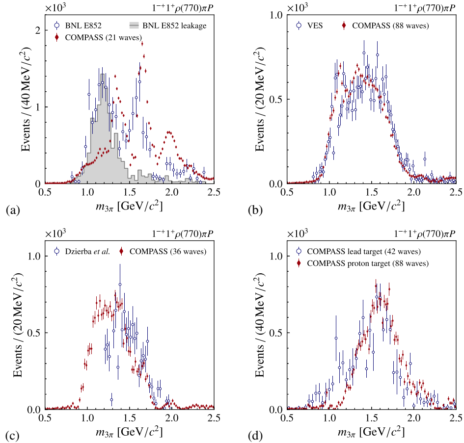
FIG. 3. Comparison of intensity distributions of the spin-exotic 1^{-+}1^{+}\rho(770)\pi P wave as obtained by different experiments measuring diffractive dissociation of a pion beam into 3\pi . Blue data points: (a) 21-wave fit of BNL E852 data in the range 0.05 < t' < 1.0 (\text{GeV}/c)^2 , (b) 44-wave fit of VES data in the range 0.03 < t' < 1.0 (\text{GeV}/c)^2 , (c) 36-wave fit of BNL E852 data in the range 0.18 < t' < 0.23 (\text{GeV}/c)^2 , and (d) 42-wave fit of COMPASS lead-target data in the range 0.1 < t' < 1.0 (\text{GeV}/c)^2 . The gray shaded area in panel (a) shows the result of a leakage study performed by the BNL E852 experiment [42]. The red data points show the results of corresponding analyses of the COMPASS proton-target data using 11 t' bins in the range 0.1 < t' < 1.0 (\text{GeV}/c)^2 : (a) t' -summed intensity distribution from the 21-wave PWA, (b) t' -summed intensity distribution from the 88-wave PWA, (c) intensity distribution from the 36-wave PWA in the range 0.189 < t' < 0.220 (\text{GeV}/c)^2 , and (d) intensity distribution from the 88-wave PWA in the range 0.449 < t' < 0.724 (\text{GeV}/c)^2 . The red data points are scaled such that the intensity integrals of the blue and red data points in the region where they overlap are equal. The blue data points are taken from (a) Fig. 18(b) in Ref. [42], (b) Fig. 4(a) in Ref. [37], (c) Fig. 25(a) in Ref. [45], and (d) Fig. 2(d) in Ref. [43]. The red data points in (d) are taken from Fig. 43(j) in Ref. [46].
