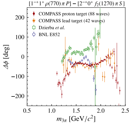
FIG. 4. Comparison of the phases of the spin-exotic 1^{-+}1^+\rho(770)\pi P wave with respect to the 2^{-+}0^+f_2(1270)\pi S wave as obtained by different experiments measuring diffractive dissociation of a pion beam into 3\pi . Blue data points: 21-wave fit of BNL E852 data in the range 0.05 < t' < 1.0 (GeV/c) 2 (shifted by -180^\circ ); green data points: 36-wave fit of BNL E852 data in the range 0.18 < t' < 0.23 (GeV/c) 2 (shifted by +180^\circ ); orange data points: 42-wave fit of COMPASS lead-target data in the range 0.1 < t' < 1.0 (GeV/c) 2 ; red data points: 88-wave fit of COMPASS proton-target data in the range 0.449 < t' < 0.742 (GeV/c) 2 (values for m_{3\pi} < 1.1 GeV/c 2 not shown). Note that phase shifts of 180^\circ may be caused, e.g., by different choices of the analyzers in the definition of the coordinate systems or by different conventions used for the Wigner D functions. The data points were taken from Fig. 19(i) in Ref. [42] (blue), Fig. 33 in Ref. [45] (green), Fig. 3(b) in Ref. [43] (orange), and Fig. 121 in Ref. [53] (red).
