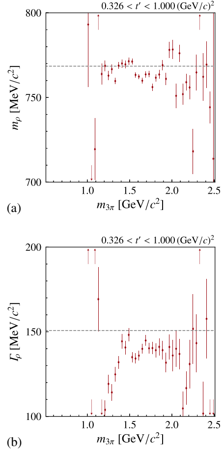
FIG. 7. Parameters of the \rho(770) resonance obtained by fitting the J^{PC} = 1^{-+} dynamic isobar amplitudes of the spin-exotic wave from the freed-isobar PWA. The fit is performed independently in every (m_{3\pi}, t') cell; the results shown are for the highest t' bin. (a) shows the \rho(770) mass and (b) the \rho(770) width. The gray lines indicate the corresponding parameter values used in the conventional PWA.
