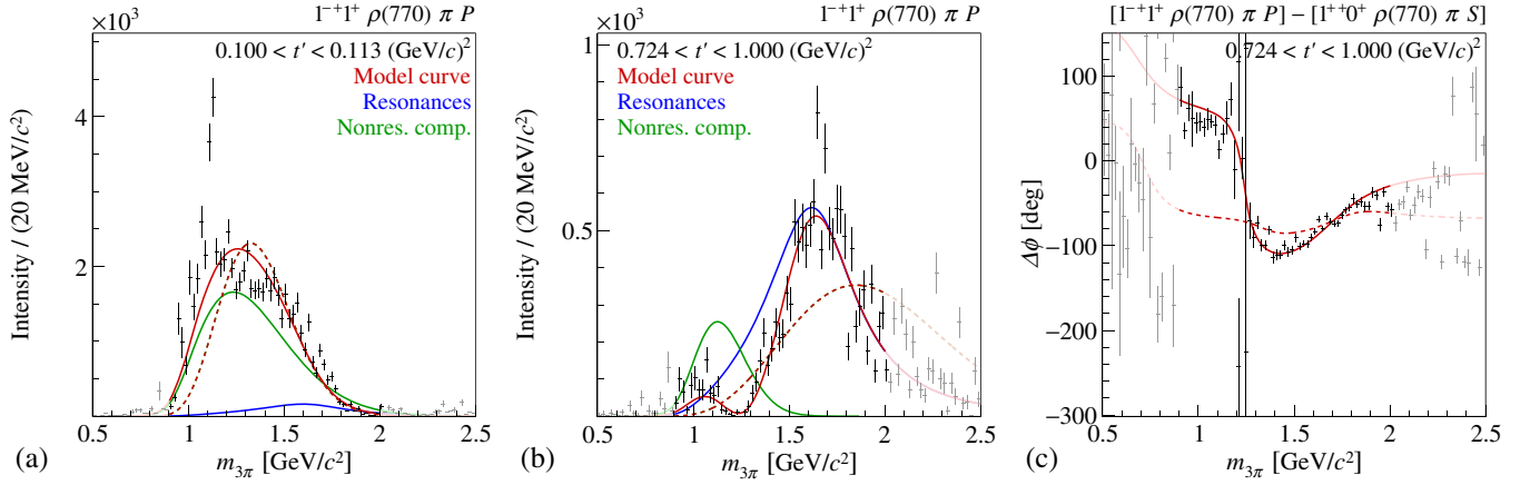
FIG. 1. Excerpt from the results of a previous study of resonance production in \pi^- p \rightarrow \pi^- \pi^- \pi^+ p at 190 GeV/c pion-beam momentum by the COMPASS collaboration [46,47]. The partial-wave intensities of the spin-exotic \rho(770)\pi P -wave carrying J^{PC} = 1^{-+} are shown in (a) and (b) for the lowest and highest t' bins, respectively, covered by the experiment. Panel (c) shows the phase relative to the \rho(770)\pi S -wave carrying J^{PC} = 1^{++} . The red solid curve represents the full resonance model (see Table II in Ref. [46]), which is the coherent sum of wave components that are represented by the other solid curves: \pi_1(1600) resonance (blue curves) and nonresonant component (green curves). The extrapolation of the model and the wave components beyond the fit range are shown in lighter colors. The narrow enhancement at 1.1 GeV/c 2 in (a) is likely an artifact induced by imperfections in the analysis method (see Sec. IV A). The dashed red curves represent a fit, where the \pi_1(1600) resonance was omitted from the fit model. This curve hence corresponds to a purely nonresonant \rho(770)\pi P -wave.
