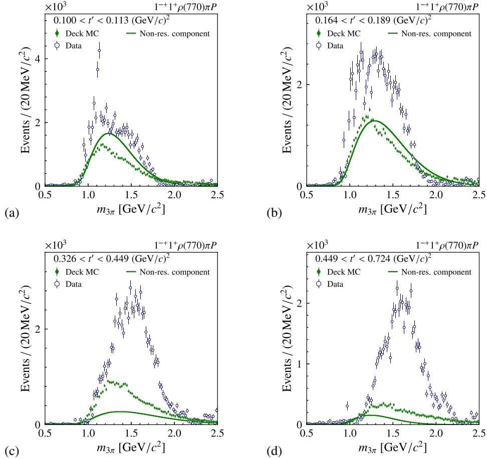
FIG. 13. Intensity distributions of the 1^{-+}1^{+}\rho(770)\pi P wave in different t' bins as obtained from the 88-wave PWA. The real data are represented by the blue data points; the Deck pseudodata by the green data points. The green curve represents the nonresonant component determined in the resonance-model fit in Ref. [46]. The pseudo data are normalized using a common factor for all waves (see text for details).
