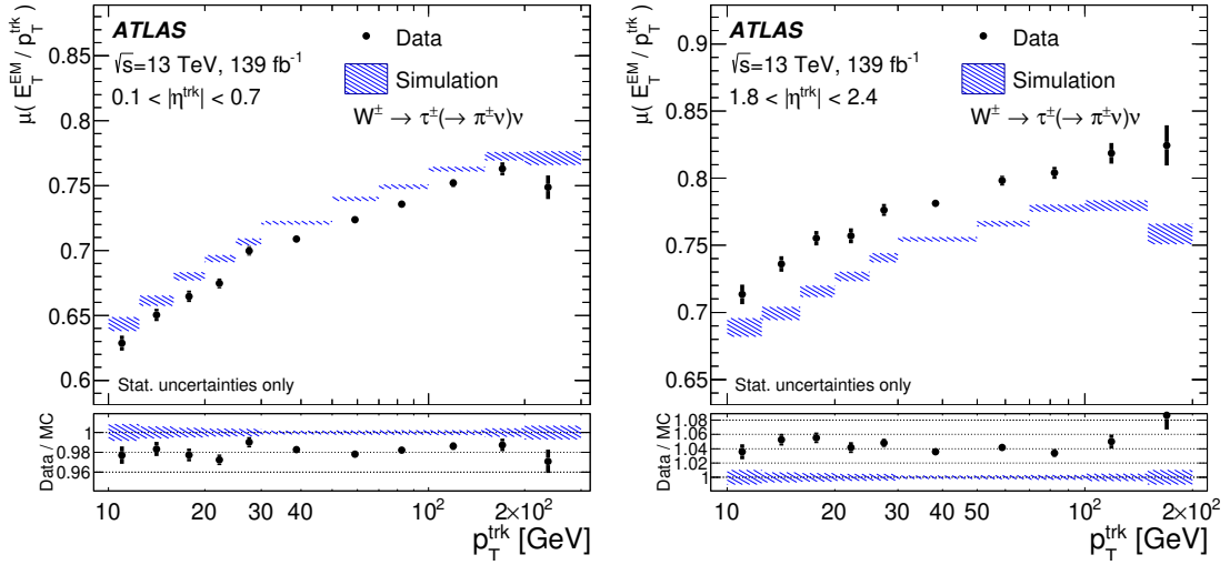
Figure 2: The fitted mean of the signal E_T^{\text{EM}}/p_T^{\text{trk}} distribution as a function of the track p_T in the central region (left) and endcap region (right). The error bars and uncertainty band show only the statistical uncertainties from the size of the dataset and simulated samples respectively.
