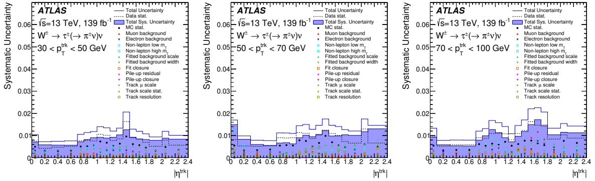
Figure 5: The various systematic uncertainties which affect the measurement of the calorimeter energy scale for charged pions as a function of |\eta^{\text{trk}}| for three p_{\text{T}}^{\text{trk}} ranges: 30 < p_{\text{T}}^{\text{trk}} < 50 GeV, 50 < p_{\text{T}}^{\text{trk}} < 70 GeV and 70 < p_{\text{T}}^{\text{trk}} < 100 GeV.
