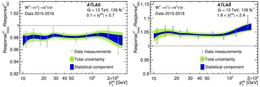
Figure 6: The measured data to simulation ratio of the response as a function of p_{\text{T}}^{\text{trk}} for the barrel (left) and endcaps (right). Points represent the different measurement bins with their total uncertainty from both the statistical and systematic sources. Also shown is the smooth calibration curve with its associated uncertainties.
