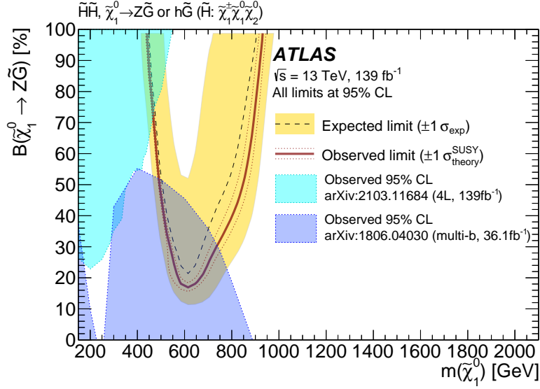
Figure 16: Expected (dashed) and observed (solid red) 95% CL exclusion limits derived for the (\tilde{H}, \tilde{G}) model, as a function of the lightest higgsino mass m(\tilde{\chi}_1^0) and the branching ratio \mathcal{B}(\tilde{\chi}_1^0 \rightarrow Z\tilde{G}) (= 1 - \mathcal{B}(\tilde{\chi}_1^0 \rightarrow h\tilde{G})) . The excluded region is indicated by the area inside the contour. The exclusion limits from the previous ATLAS search using 4-lepton final states [31] (cyan, denoted by “4L”), or final states with three or more b -jets [30] (violet, denoted by “multi- b ”) are shown by the shaded areas.
