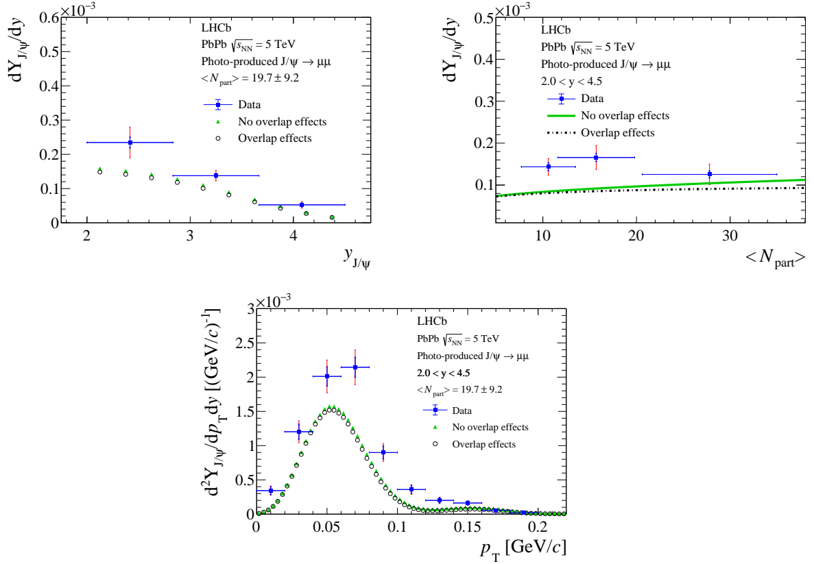
Figure 2: (Top left) Differential yields of photo-produced J/\psi candidates as a function of rapidity and (top right) \langle N_{part} \rangle . (Bottom) Double differential yields as a function of p_T . The vertical inner blue bars represent the statistical uncertainty and the outer red bars the total uncertainty. The horizontal bars in the \langle N_{part} \rangle results correspond to the standard deviation of the N_{part} distribution of the MB events. The yields are compared to the prediction from Ref. [16,33] that take (black) or not take (green) into account the effect from the overlap region of the collision.
