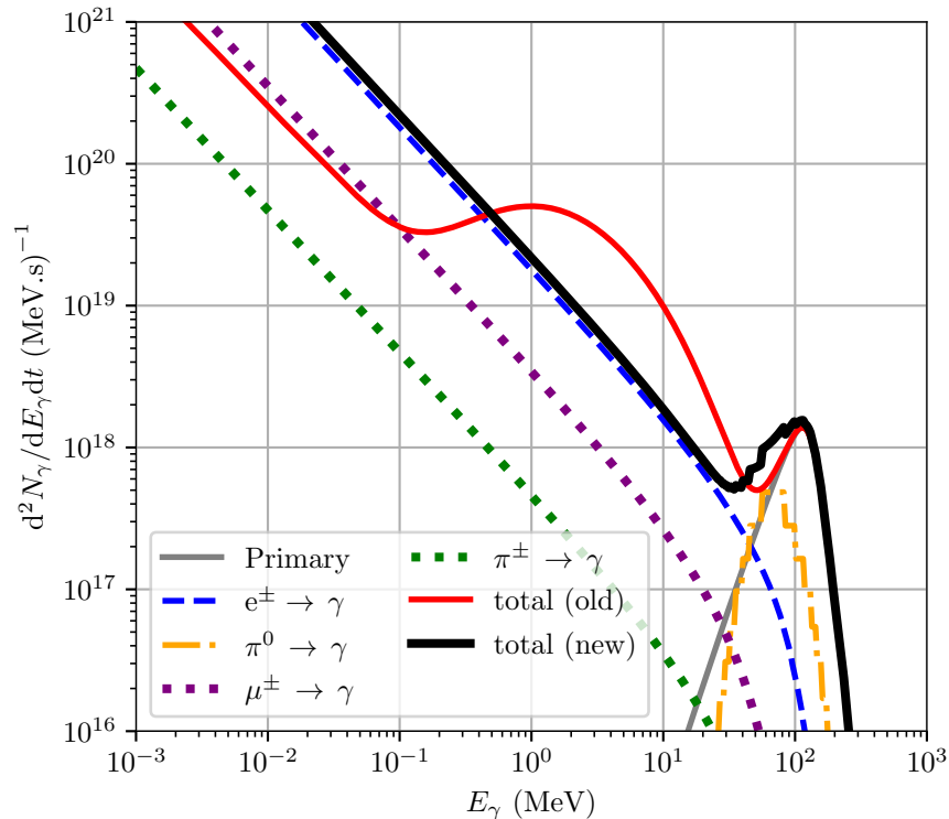
FIG. 4. Comparison between the old PYTHIA extrapolated (solid red) and new Hazma computed (solid black) BlackHawk instantaneous total photon spectrum for a M_{\text{BH}} = 5.3 \times 10^{14} g. From left to right: primary photon spectrum (grey solid); neutral pion decay (orange dot-dashed); electron FSR (blue dashed); muon decay+FSR (purple dotted); charged pion decay+FSR (green dotted). To be compared with Fig. 2 upper left panel of [12].
