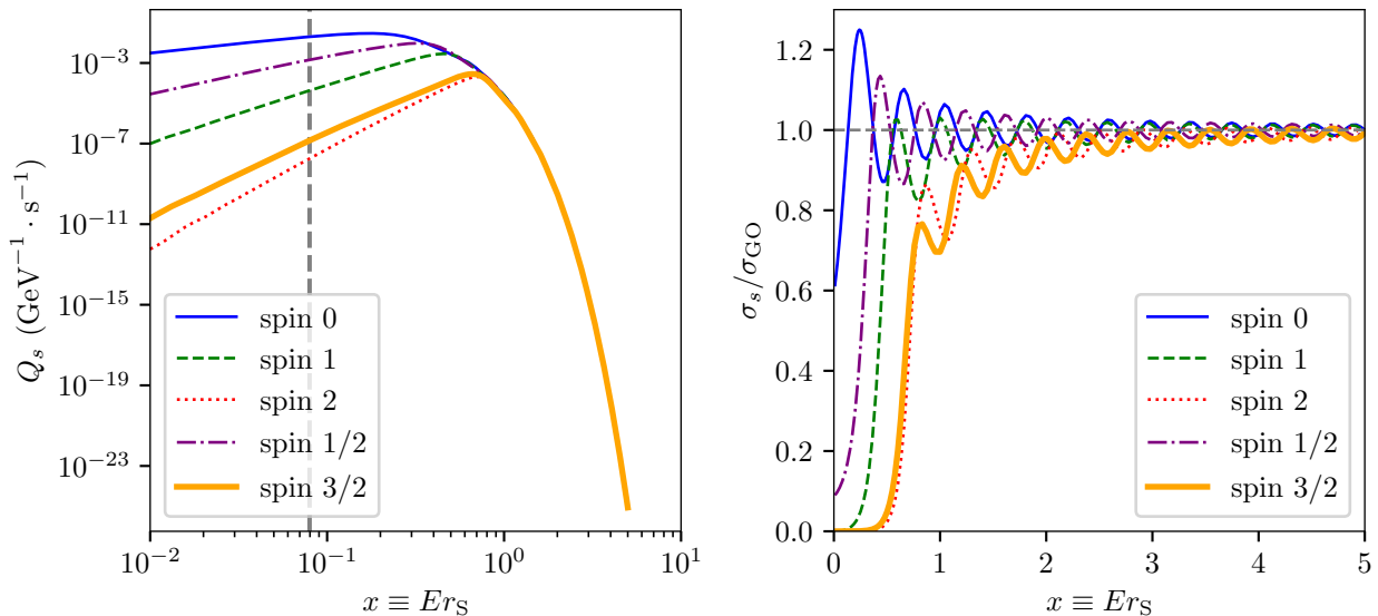
FIG. 1. Hawking spectra of massless particles of spins 0 (solid blue), 1 (dashed green), 2 (dotted red) and 1/2 (dot-dashed purple) as well as the new spectrum of the massless spin 3/2 fermion (thick solid orange) for a Schwarzschild BH. Left: Full spectra in logarithmic scale, the black vertical line represents the BH temperature. These spectra are shape invariant when changing the BH mass. Right: High energy oscillations of the cross-section, the black horizontal line represents the geometrical optics approximation.
