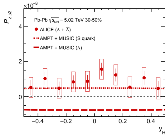
Figure 4: (color online) The rapidity dependence of P_{z,s2} averaged for \Lambda and \bar{\Lambda} in Pb–Pb collisions at \sqrt{s_{\text{NN}}} = 5.02 TeV in semi-central collisions. The model calculations [38] for \Lambda and strange quark for Pb–Pb collisions at \sqrt{s_{\text{NN}}} = 5.02 in the 30–50% centrality interval using the approach described in Ref. [23] are shown by dash-dotted lines.
