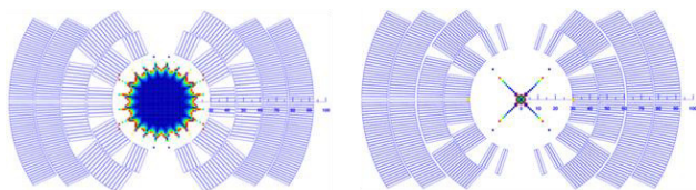
Figure 5: Cross-sections of optimized (left) and “interim” (right) coils with the field quality in coil bore.
