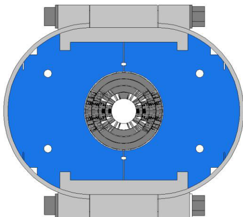
Figure 6: Cold mass cross-section with the 11 T dipole coil.
