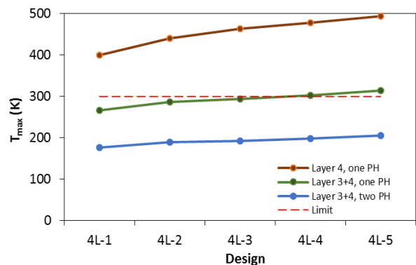
Figure 4: Average coil quench temperature at maximal bore field for the studied coil designs.
