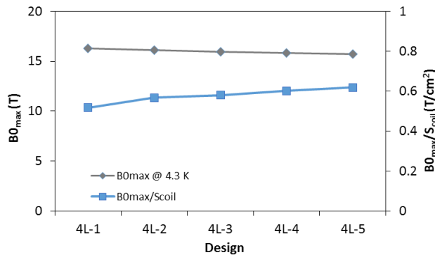
Figure 2: Maximum bore field and ratio of the bore field to the coil cross-section area for the studied coil designs.
