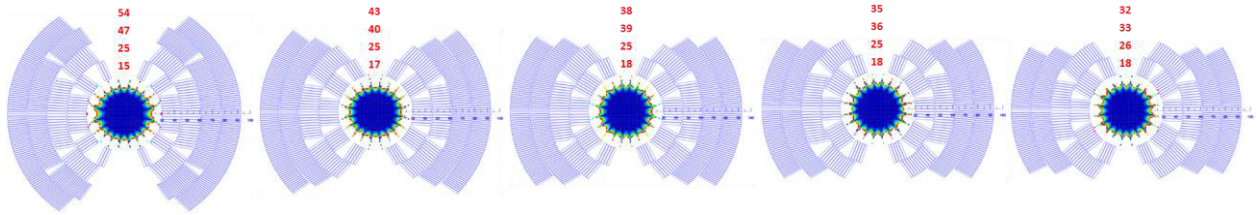
Figure 1: Coil cross-sections with relative field errors in the aperture (dark blue area).
