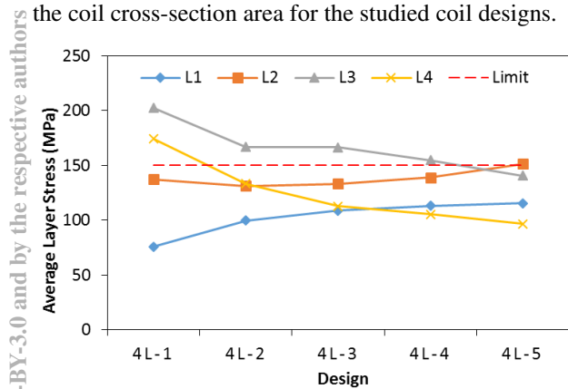
Figure 3: Average azimuthal stress in the coil mid-plane at the maximal bore field for the studied coil designs.
