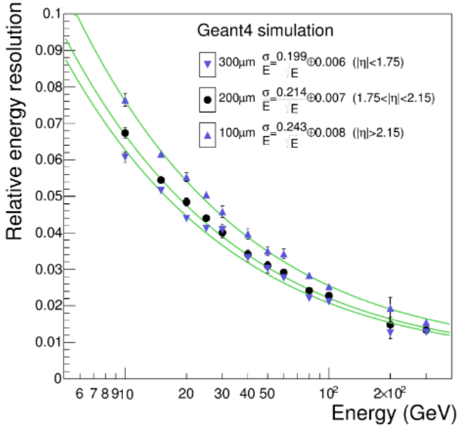
Figure 9.5: Energy resolution as a function of energy from a standalone simulation of incident electrons on HGCALE, for different thickness of silicon sensors [203].
