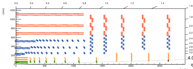
Figure 9.1: Layout of one quarter longitudinal section of the CMS Tracker for the HL-LHC. The upgraded tracking detector will extend the coverage for charged particles up to |\eta| = 4 . In green (yellow) the silicon pixel detectors of the Inner Tracker with two (four) readout chips per module. In blue (red) the PS (2S) silicon detector modules of the Outer Tracker [203].
