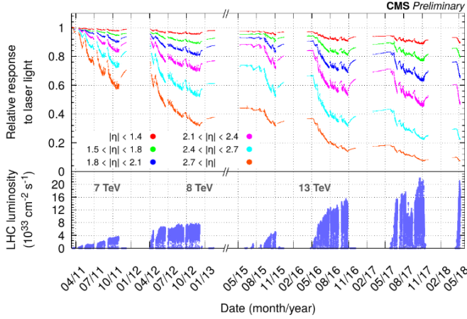
Figure 9.3: Upper panel: relative ECAL response as a function of time at different \eta regions as monitored by laser calibrations since 2011. Lower panel: corresponding LHC luminosity. From Ref. [212].
