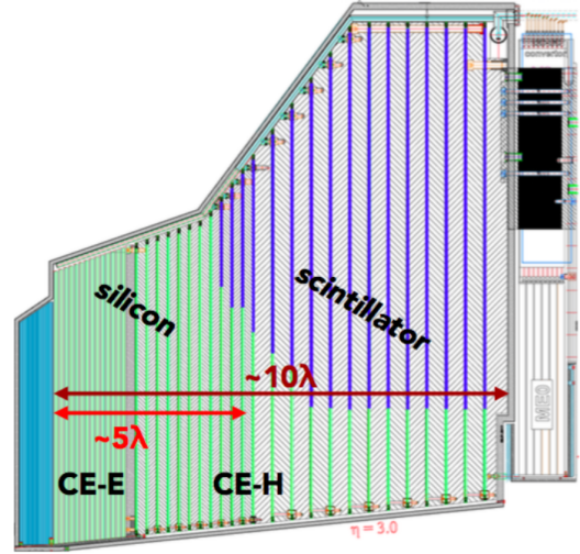
Figure 9.4: Schematic drawing of the CMS HGCAL design [165].
