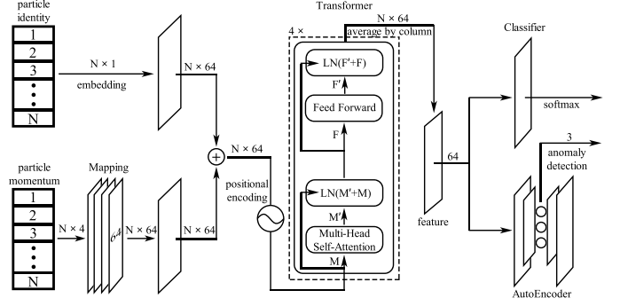
Figure 8.1: Architecture of neural network [189].
