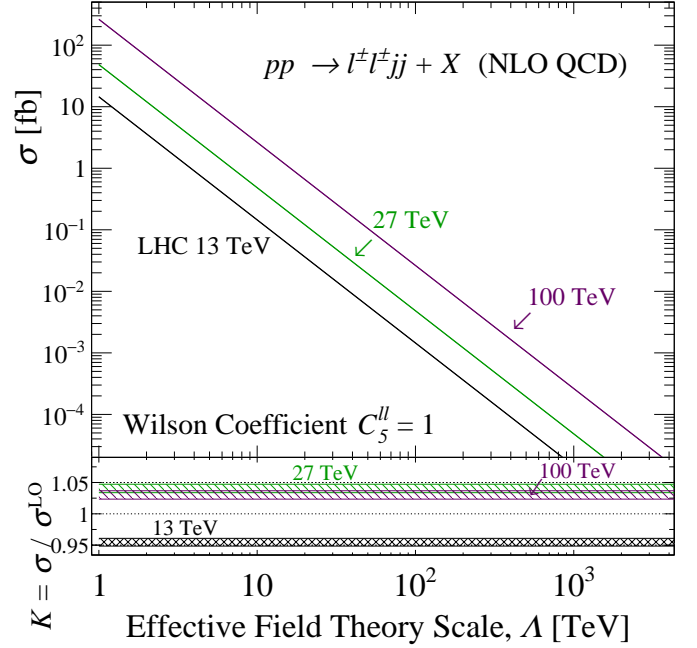
Figure 6.4: Cross section predictions at NLO in QCD for the W^\pm W^\pm \rightarrow \ell_i^\pm \ell_j^\pm process when mediated by the Weinberg operator for representative pp collider energies [78].
