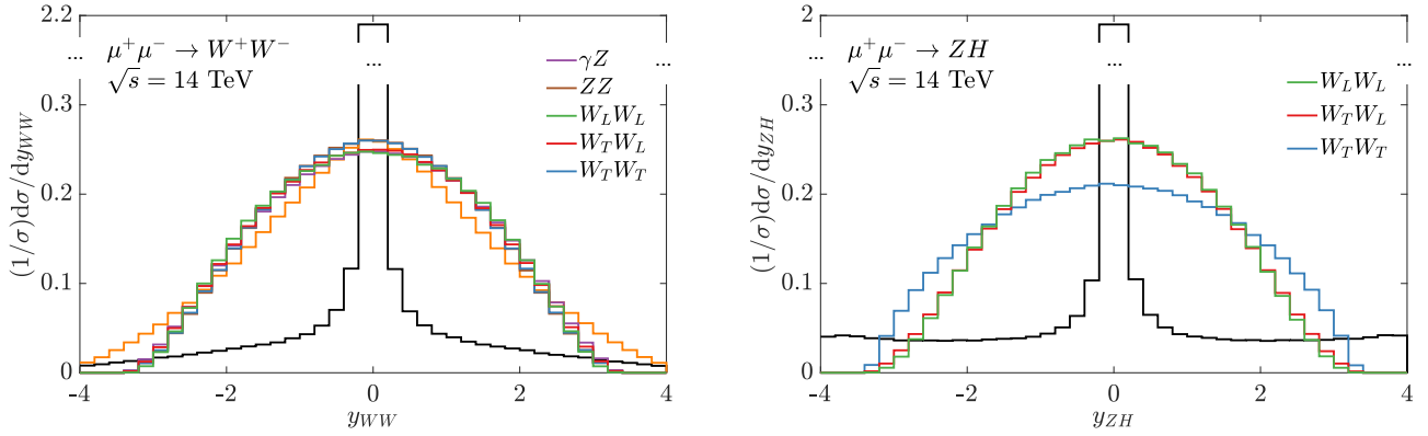
Figure 11.3: Normalized di-boson rapidity distributions for W^+W^- (Left) and ZH (Right) production at a muon collider at \sqrt{s} = 14 TeV. Annihilation ( \mu\mu , black) and diboson fusion (colored) processes are compared.
