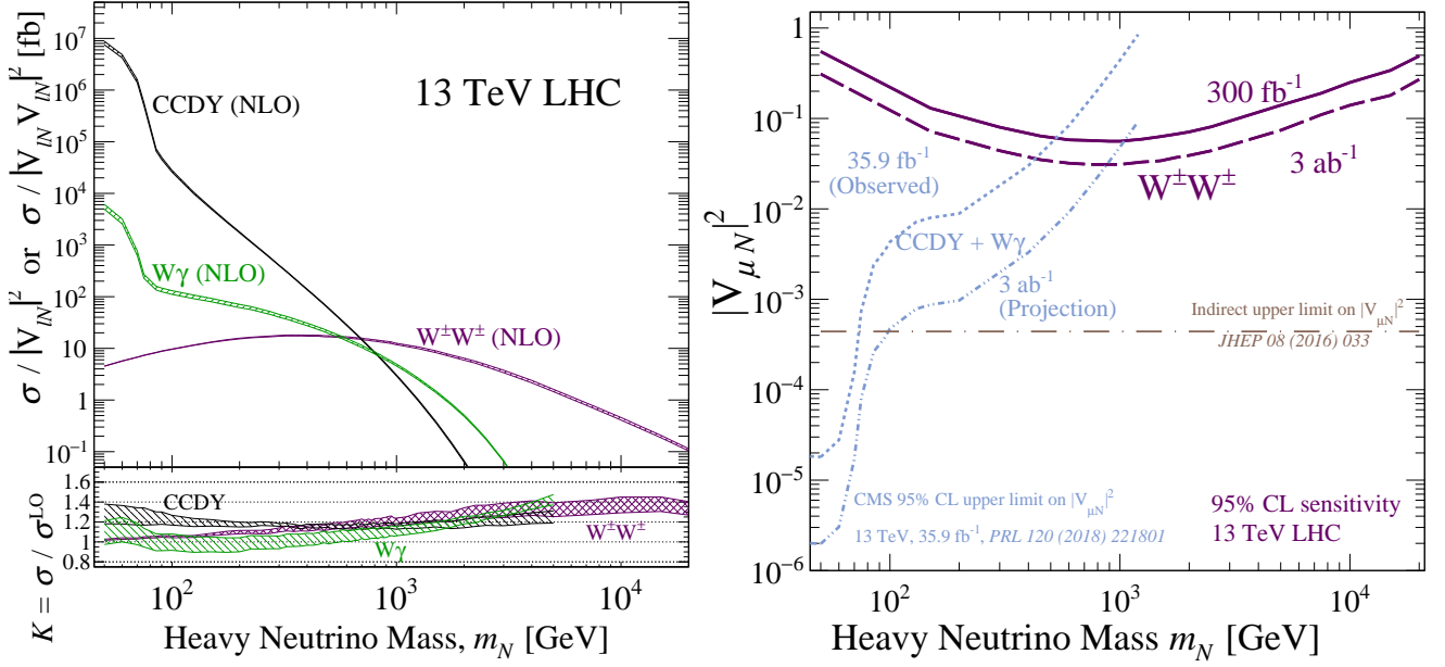
Figure 6.1: Left: Cross section predictions at NLO in QCD at the \sqrt{s} = 13 TeV LHC for heavy Majorana neutrinos N production via the charged current Drell-Yan (CCDY), W\gamma fusion, and same-sign W^+W^+ fusion mechanisms, assuming a benchmark active-sterile mixing of |V_{lN}| = 1 . Right: Sensitivity projections for active-sterile mixing of |V_{lN}|^2 at the LHC for the W^+W^+ channel in comparison to experimental limits [133, 134]. Figures adapted from Ref. [77].
