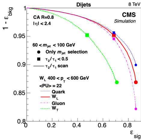
Figure 7.3: Efficiency for correctly identifying longitudinal (red) and transverse (dotted green) vector bosons versus 1-efficiency for tagging quark (dotted blue) or gluon (dotted pink) jets [172].
