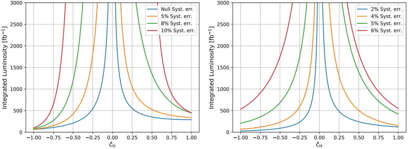
Figure 8.3: Integrated luminosity required to probe the signal (with different \bar{c}_H ) at 95% C.L. in the dileptonic channel (Left) and semi-leptonic channel (Right). Several different systematic uncertainties are considered. From Ref. [189].
