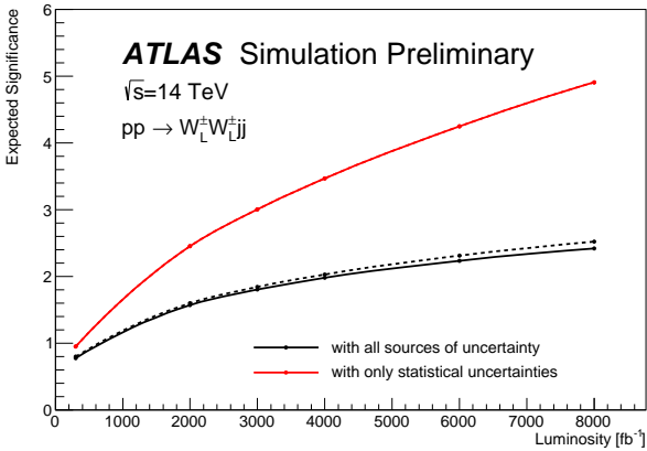
Figure 4.7: Projection of the expected significance of the W_L^\pm W_L^\pm scattering process as function of integrated luminosity, considering all sources of uncertainty (black) or only the statistical uncertainty (red). The dashed line show the expectation for the optimistic scenario [109].
