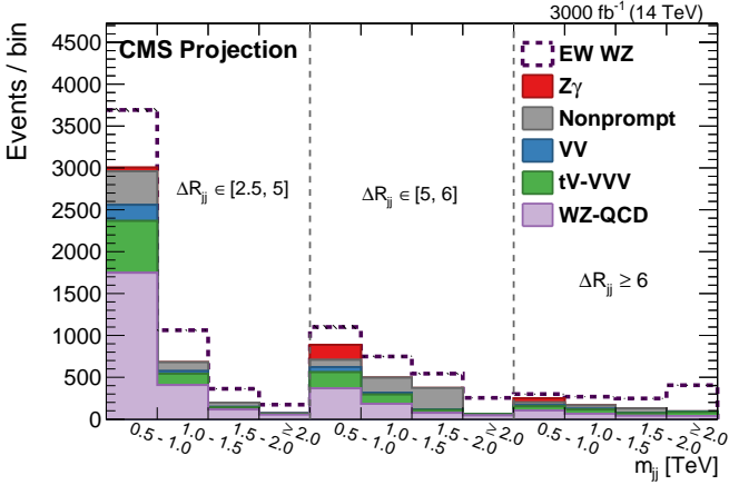
Figure 4.3: Distribution of m_{jj} in bins of \Delta R_{jj} , i.e. the distance (in the \eta, \phi space) between jets. From Ref. [107].
