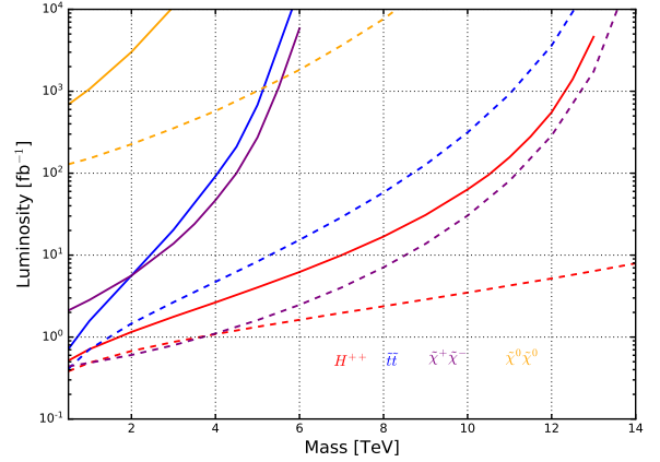
Figure 14.2: Required luminosity [ \text{fb}^{-1} ] for a 5\sigma discovery of H^{++} (red) in the Georgi-Machacek model; \tilde{t}\tilde{t} (blue), \tilde{\chi}^+\tilde{\chi}^- (purple), and \tilde{\chi}^0\tilde{\chi}^0 (yellow) from in the MSSM, using VBF in \sqrt{s} = 14 TeV (solid) and 30 TeV (dashed) muon collisions. Adapted from Ref. [302].
