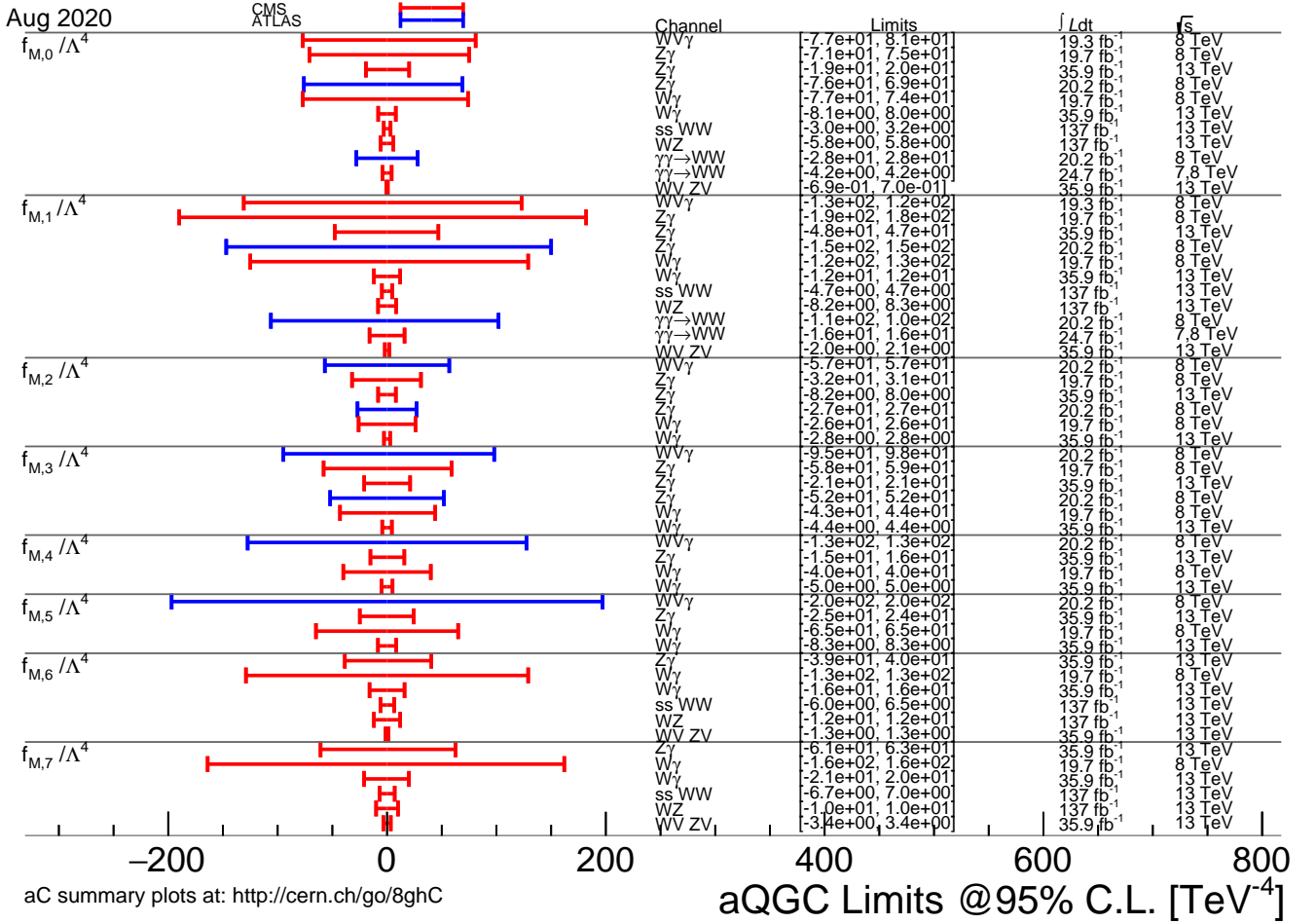
Figure 1.4: Summary of constraints on the couplings to the EFT operator F_{M,7} from experimental measurements. For details, see the URL at http://cern.ch/go/8ghC .
