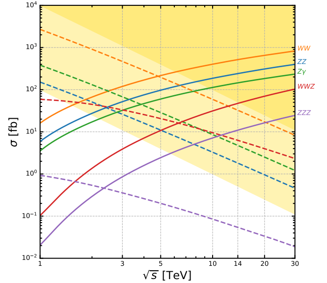
Figure 13.2: Multi-boson production cross sections at a muon collider as a function of colliding energy. Solid lines show VBS production while dashed lines show s -channel ones. The former benefits from a logarithmic growth with respect to the latter that decreases with energy. The light-shaded region corresponds to at least 10k expected events, while the darker shaded region to 1M. Adapted from Ref. [302].
