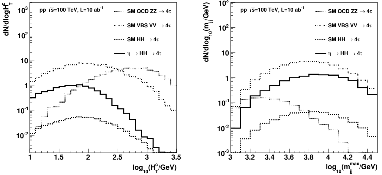
Figure 15.2: Left: The distribution of H_T^c , the scalar sum of the transverse momenta of the central jets. Right: The distribution of dijet mass of the forward jets. Figures are adapted from Ref. [329].
