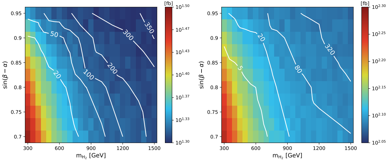
Figure 8.4: Contours corresponding to the required integrated luminosity to probe the signal (with different \sin(\beta - \alpha) and m_{H_2} ) at 95% C.L. Color grades correspond to the fiducial cross sections (requiring m_{jj} > 500 GeV at the parton level) times the branching rates. The systematic uncertainties are set to 5% for both the dileptonic channel (Left) and semi-leptonic channel (Right). Adapted from Ref. [189].
