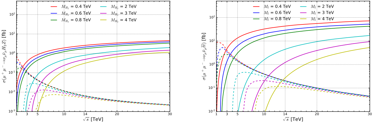
Figure 14.1: Cross section [fb] via VBF (solid lines) and s -channel annihilation (dashed lines) for H_2 Z associated production in the 2HDM (left) and \tilde{t}\tilde{t} pair production in the MSSM (right), from Ref. [302].
