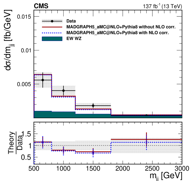
Figure 1.1: The unfolded results for the WZjj process from Ref. [32]. The contribution of the EW production and the impact of NLO EW corrections are shown.
