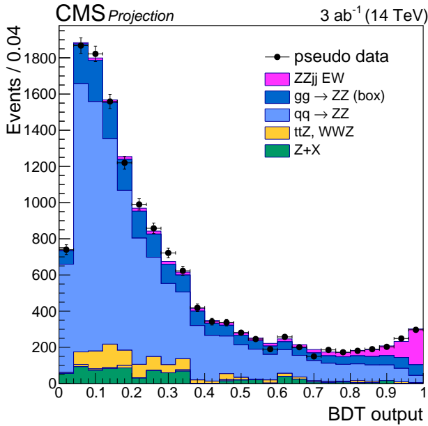
Figure 4.5: BDT discriminator output for a luminosity of 3000 \text{ fb}^{-1} at \sqrt{s} = 14 \text{ TeV} , for signal and for the backgrounds (from Ref. [108]). The purple filled histogram represents the EW signal ( ZZjj inclusive process), the other histograms represent the different backgrounds.
