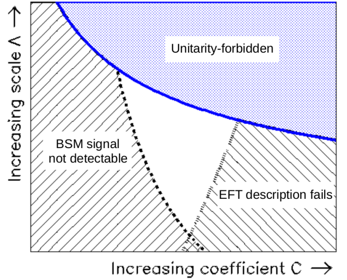
Figure 5.1: For a Wilson coefficient C and EFT cutoff scale \Lambda , a sketch of the regions in \Lambda-C space that are forbidden by unitarity (large \Lambda and large C ), are inconsistent with the assumptions of EFTs (small \Lambda and large C ), and are inaccessible to experiments (small C and/or large \Lambda ). Adapted from Ref. [115].
