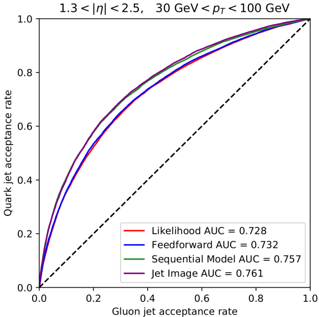
Figure 7.1: ROC curves showing the quark-jet acceptance rate as a function of the gluon-jet acceptance rate for each quark/gluon discriminator in the detector’s endcap region of 1.3 < |\eta| < 2.5 and 30 < p_T < 100 GeV, from Ref. [167]. The red line corresponds to the benchmark likelihood-based discriminator. The blue, green and purple lines correspond to three neural network models.
