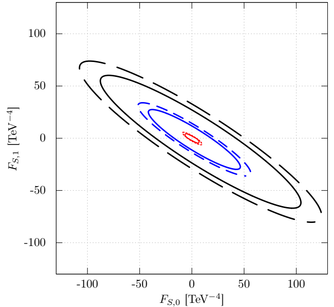
Figure 10.2: The 90 % exclusion sensitivities for polarized (solid) and unpolarized (dashed) particle beams at energies of \sqrt{s} = 1 (black), 1.4 (blue), 3 TeV (red) combined, assuming integrated luminosities of 5 \text{ ab}^{-1} at \sqrt{s} = 1 TeV, 1.5 \text{ ab}^{-1} at \sqrt{s} = 1.4 TeV, and 2 \text{ ab}^{-1} at \sqrt{s} = 4 TeV. Adapted from Ref. [224].
