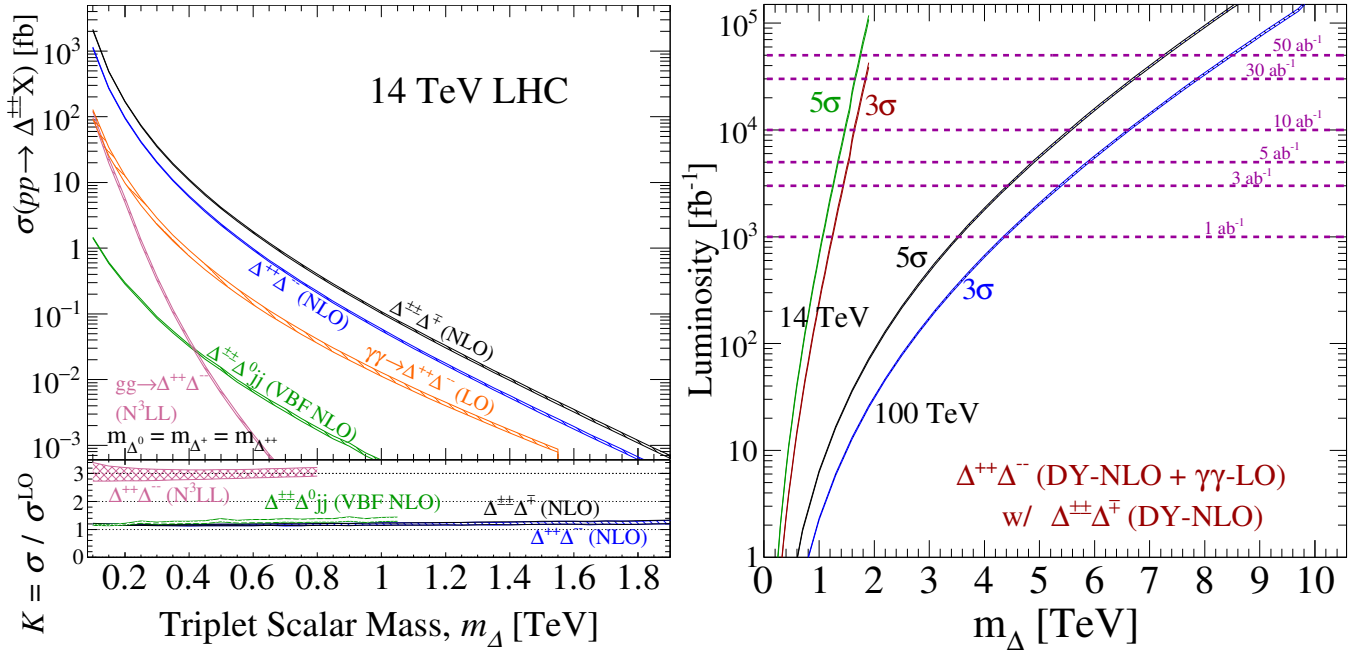
Figure 6.3: Left: High-precision cross sections predictions at the \sqrt{s} = 14 \text{ TeV} LHC for doubly charged Higgs \Delta^{\pm\pm} production via various mechanisms in the Type II Seesaw. Right: Sensitivity projections to \Delta^{\pm\pm} for the LHC and a hypothetical collider at \sqrt{s} = 100 \text{ TeV} [100].
