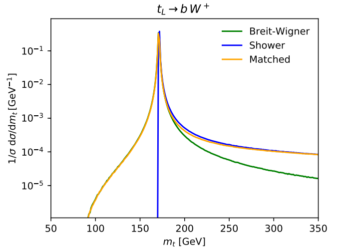
Figure 12.1: Mass spectra of the decay of a 1 TeV left-handed top quark. The matched spectrum (orange) is the numerical combination of the Breit-Wigner distribution (green) for small virtualities, and the shower distribution (blue) for large virtualities.
