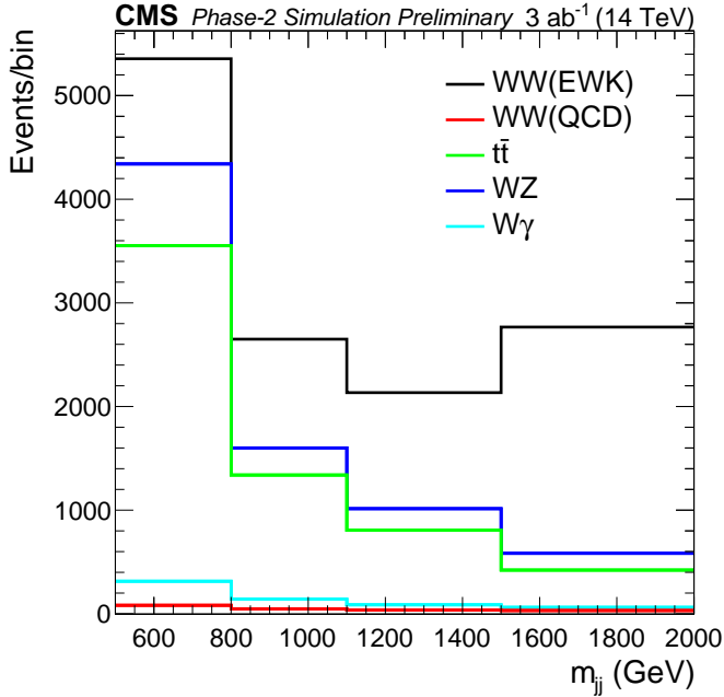
Figure 4.1: Invariant mass of the two leading jets of the W^\pm W^\pm jj process at \sqrt{s}=14 TeV and normalized to an integrated luminosity of 3000 \text{ fb}^{-1} , from Ref. [104].
