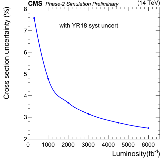
Figure 4.2: Total cross section uncertainty of the W^\pm W^\pm jj process as a function of the integrated luminosity, considering systematic uncertainties as in the YR18 scenario [106]. From Ref. [104].
