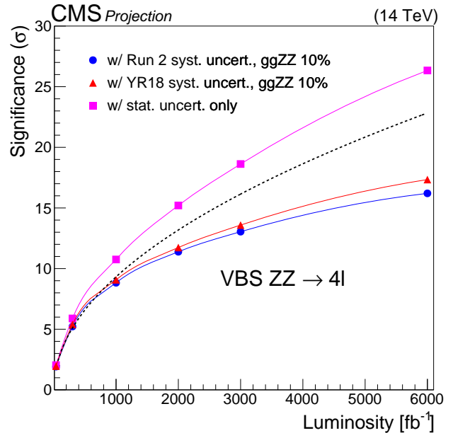
Figure 4.6: Significance as a function of the integrated luminosity in the Run 2 (blue line, circles) and YR18 (red line, triangles) scenarios. The QCD ggZZ background yield uncertainty is set to 10%. Results considering only the statistical uncertainties are also included (magenta line and squares), as well as those obtained by scaling the statistical uncertainties of the 2016 results by the luminosity ratio (dashed black line). From Ref. [108].
