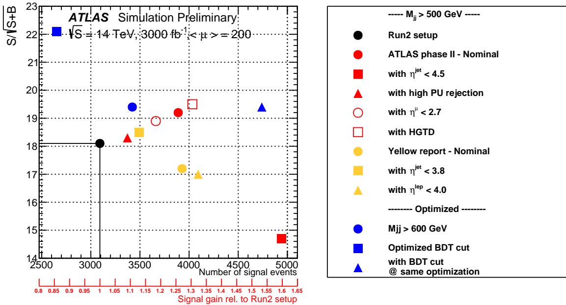
Figure 4.8: Overview over the anticipated sensitivity performance for the WZ process for the HL-LHC phase achieved using the event selections based on the detector performance parameters described in the text. Signal sensitivity as a function of the number of events and relative signal gain with respect to the Run 2 settings. Figure from Ref. [110].
