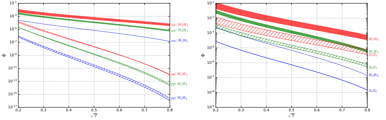
Figure 13.1: Parton luminosities \Phi as a function of the scattering energy fraction \sqrt{\tau} = M_{VV'}/\sqrt{s} (see text). Comparison between the WW parton luminosities at muon and proton colliders (Left), and the difference between Z and W bosons luminosities at a muon collider (Right). The parton luminosities have been decomposed among the various helicity combinations. Bands are given by variations of the factorization scales. Adapted from Ref. [302].
