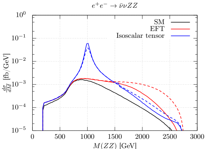
Figure 10.3: Differential cross sections depending on the invariant mass of the ZZ system in e^+e^- \rightarrow ZZ\nu\bar{\nu} at \sqrt{s} = 3 TeV. The solid lines show the signal process \bar{\nu}\nu ZZ with SM values F_{S,0} = F_{S,1} = 0 . The red lines show matched EFT results with F_{S,0} = 150.8 TeV ^{-4} and F_{S,1} = -50.3 TeV ^{-4} . The blue lines show an isoscalar tensor resonance f with m_f = 1 TeV, F_f = 17.4 TeV ^{-1} , and \Gamma_f = 100 GeV. (Dashed lines: naive EFT results, solid lines: unitarized results). Adapted from Ref. [224].
