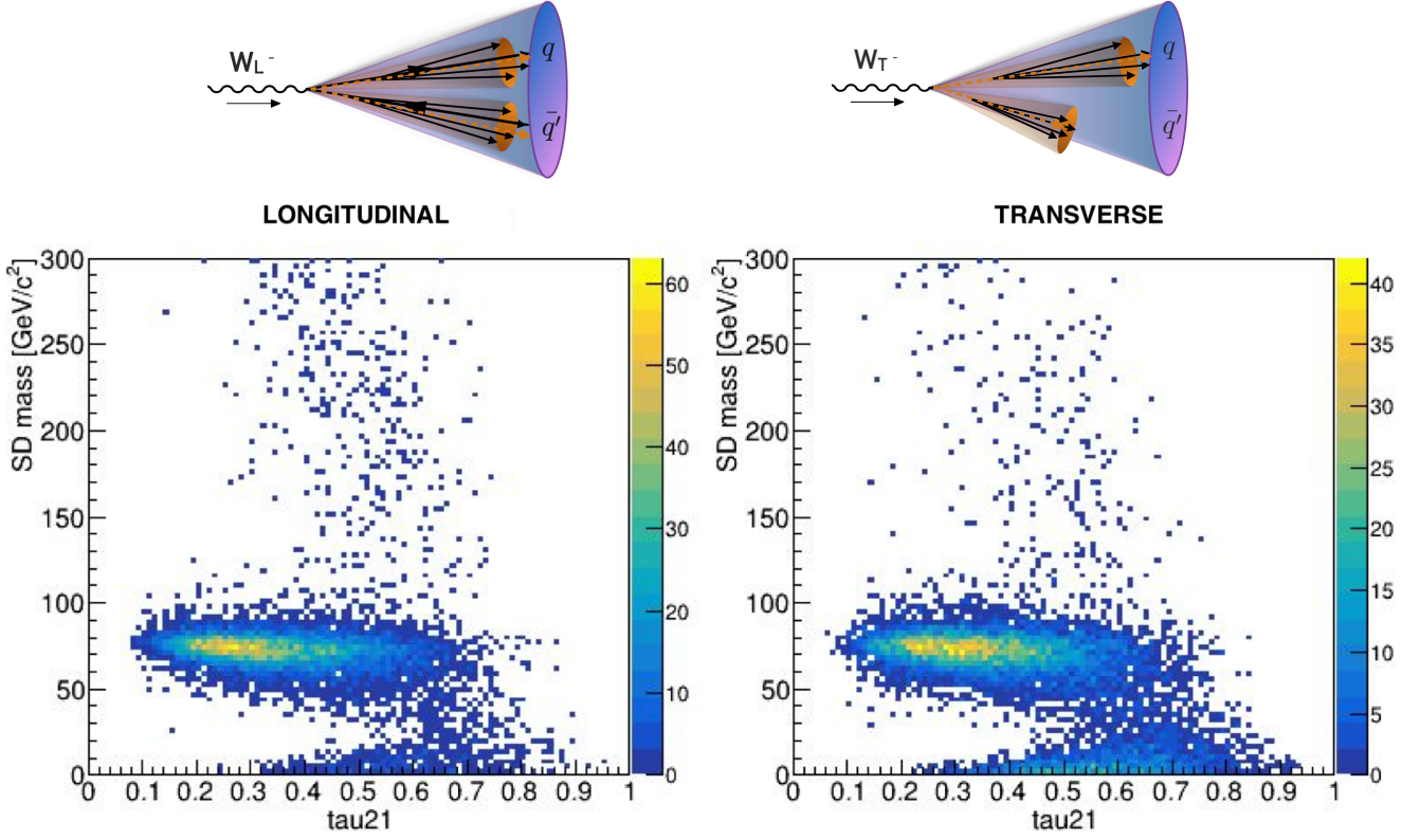
Figure 7.2: Top: Illustration of the decays of high- p_T W_L (Left) and W_T (Right) bosons in the lab frame showing that overlapping decay products are preferentially symmetric (for W_L ) or asymmetric (for W_T ) due to spin correlation. Lower: Scatter plot of the soft drop (SD) mass variable as a function of the “ N -subjettines” variable \tau_{21} for W_L (Left) and W_T (Right). Transversely polarized vector bosons (right) more frequently get reconstructed with a soft drop mass of zero and a 1-prong like substructure (i.e. larger \tau_{21} values) due to its decay products being emitted anti-parallel to the W momentum and falling out of the jet cone during the grooming process [172, 173].
