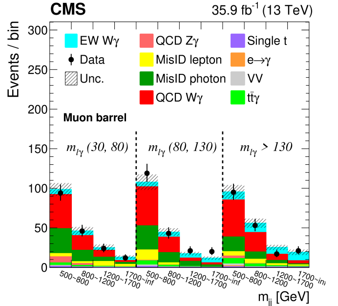
Figure 1.3: The two-dimensional distribution of m_{jj} and m_{\ell\gamma} used to extract the EW W\gamma cross section, from Ref. [41]
