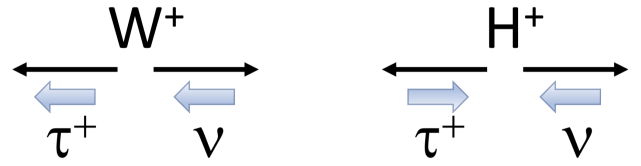
Figure 2.1: A cartoon depicting a spin-1 W boson (left) and a spin-0 charged Higgs boson (right) decaying in their rest frames to a \tau lepton and a neutrino. The resulting helicity (larger light-colored shaded arrow) of the \tau lepton depends on the originating boson: the \tau^+ polarization is P = +1 ( P = -1 ) if from a W^+ ( H^+ ).
