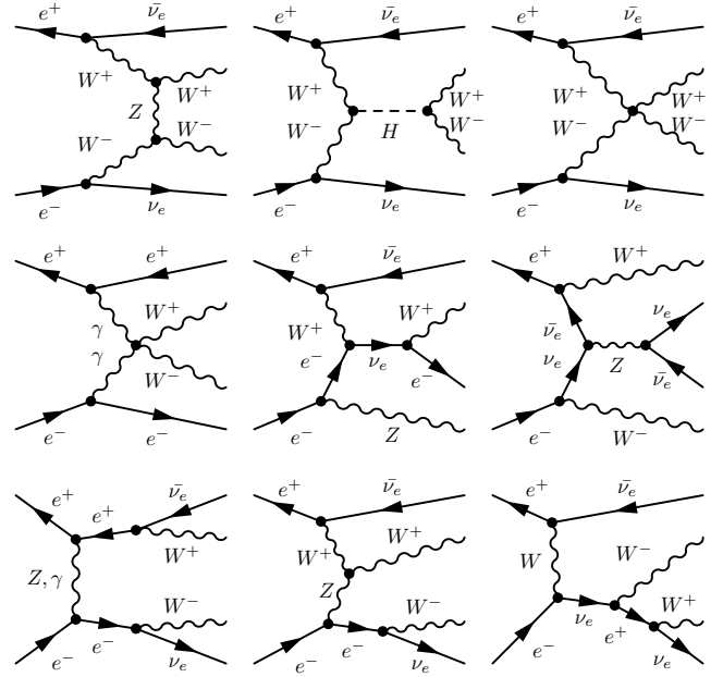
Figure 10.1: Topologies for W^+W^- scattering processes at e^+e^- colliders: signal diagrams (top row), reducible background diagrams (middle row), and irreducible diagrams (bottom row), respectively.
