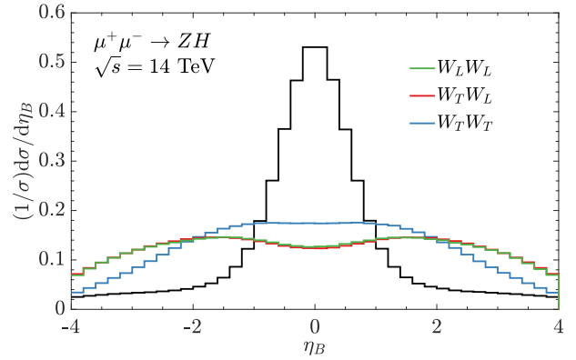
Figure 11.4: In W^+W^- (Left) and ZH (Right) production for a muon collider at \sqrt{s} = 14 TeV, the normalized pseudo-rapidity distributions of each boson ( \eta_W on the left, and \eta_B on the right). Annihilation ( \mu\mu , black histograms) and diboson fusion (colored histograms) processes are compared.
