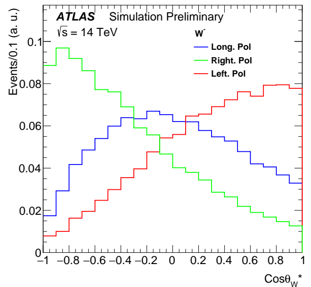
Figure 4.9: Normalized W^- polarization state templates at the reconstruction level and after the final event selection, including requiring m_{jj} > 600 GeV. Figure from Ref. [110].
