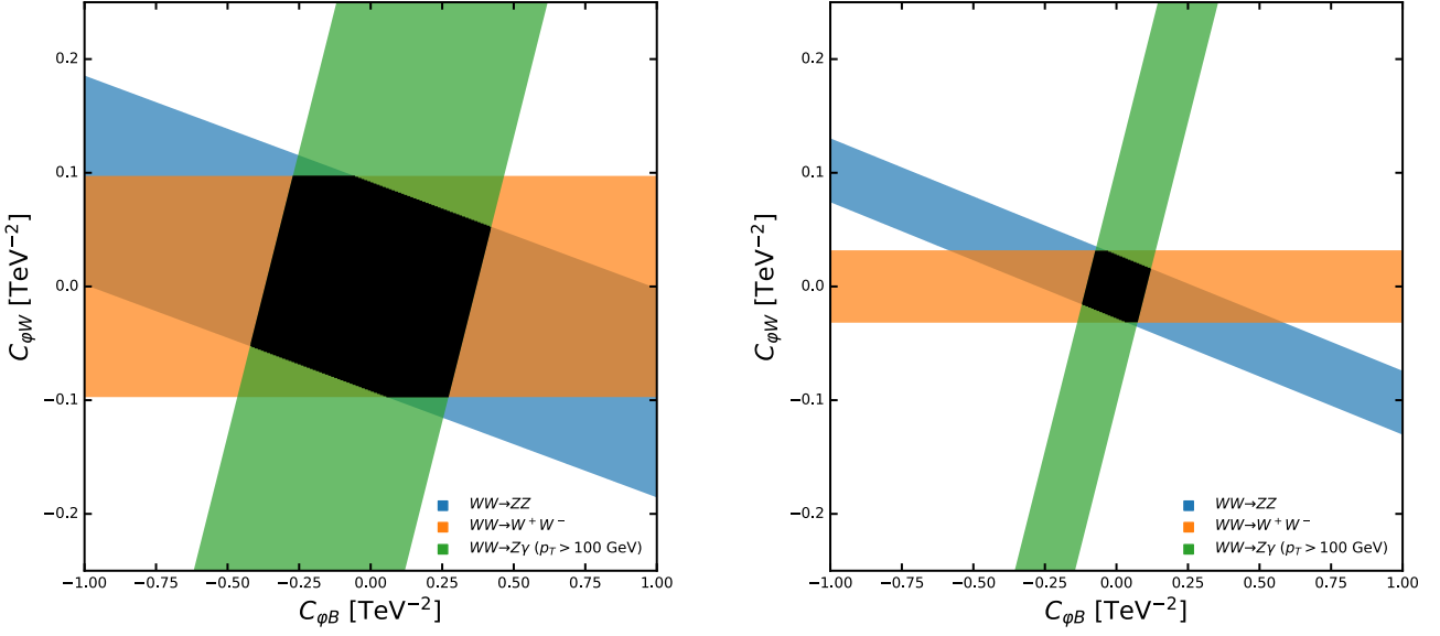
Figure 13.3: Projections for the limits imposed on the Wilson coefficients C of the operators \mathcal{O}_{\varphi B} and \mathcal{O}_{\varphi W} at a future muon collider at 3 TeV (Left) and 14 TeV (Right). Adapted from Ref. [302].
