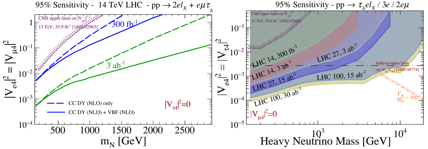
Figure 6.2: Left: Sensitivity projections for active-sterile mixing of |V_{eN}|^2 at the LHC when using only the Drell-Yan channel (dashed) and when augmented by the W\gamma fusion channel (solid) [139]. Also shown for reference are LHC limits with \mathcal{L} \approx 36 \text{ fb}^{-1} of data [133]. Right: Sensitivity projections for active-sterile mixing of |V_{eN}|^2 at the LHC and potential successor experiments using the Drell-Yan and W\gamma channels [139].
