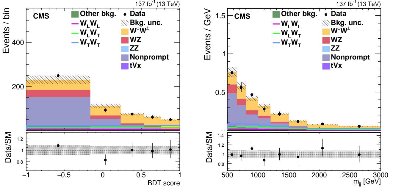
Figure 1.2: Left : The distribution of the BDT discriminant used to extract the signal strength for the polarized components of the WW cross section. Right : Dijet invariant mass distribution. Images from Ref. [29].
