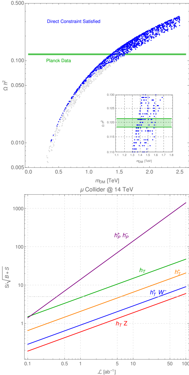
Figure 14.3: Upper: Relic density as a function of the DM. In blue (gray) the points that are allowed (disallowed) by the direct searches [325, 326, 327]. The green area represent the Planck results [328]. Lower: Significance vs luminosity for the h_T , h_T^\pm , h_T^+ W^- , h_T Z and h_P^+ h_P^- production processes through VBF at a 14 TeV muon collider. The production cross sections are multiplied by the branching ratios Br(h_T \rightarrow W^+ W^-) or Br(h_T^+ \rightarrow W^+ Z) , depending on the channel considered. The background considered is the VBF production of W^+ W^- Z in the SM, with M(W^+ W^-) = m_{h_T} or M(W^+ Z) = m_{h_T^+} . The process h_P^+ h_P^- is considered background-free because h_P^\pm is a long-lived state. Adapted from Ref. [315].
