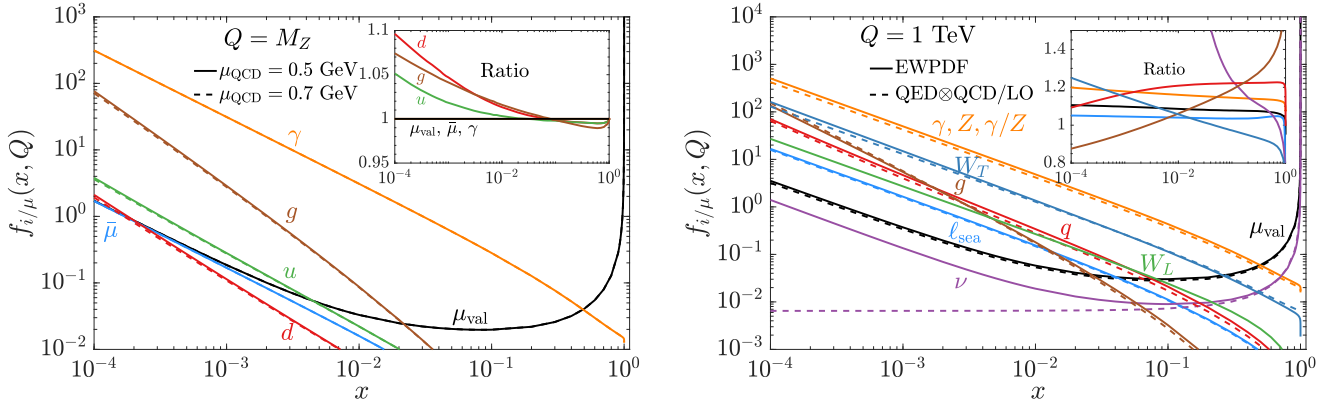
Figure 11.1: PDFs of a muon at Q = M_Z (Left) and 1 TeV (Right). Left: The solid (dashed) lines correspond to the PDFs with matching scale \mu_{\text{QCD}} = 0.5 (0.7) GeV. Right: The solid lines indicate the complete EW PDFs, while the dashed lines are the pure QED \otimes QCD evolution for \gamma, \ell_{\text{sea}}, q, g and the LO splittings for \nu, W , respectively. Inset: the ratios of the solid to dashed lines with the same colors.
