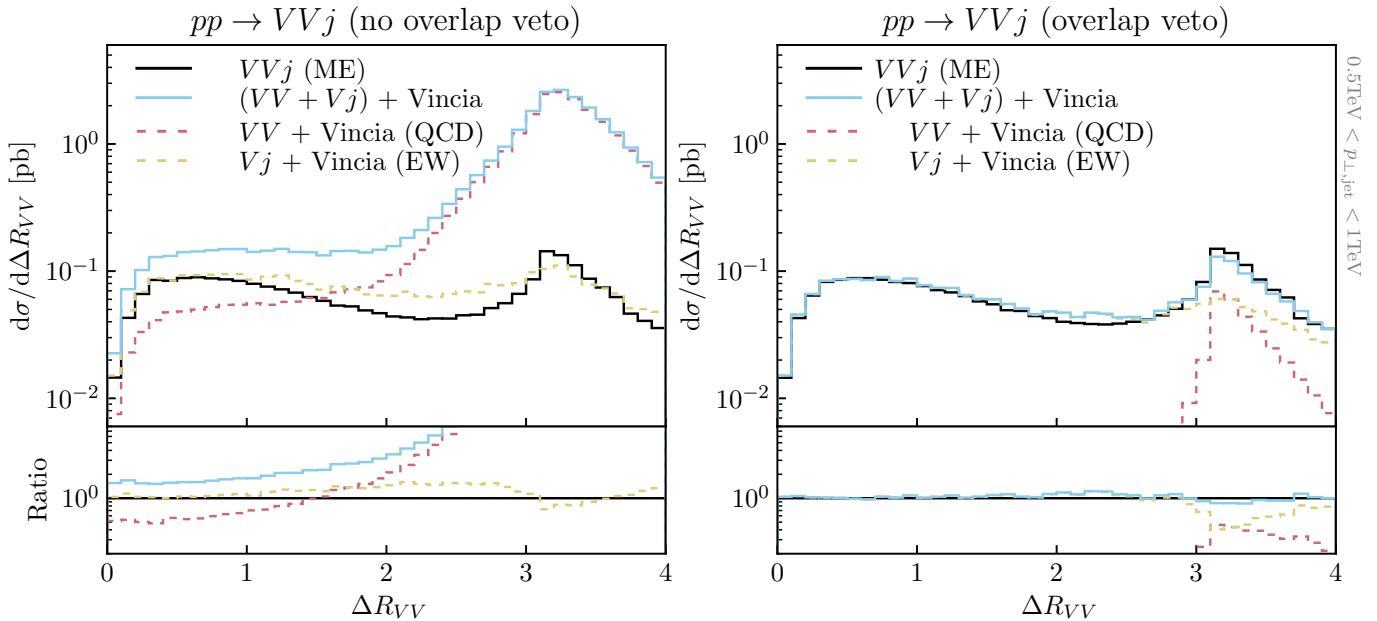
Figure 12.3: Upper: As a function of angular separation between the vector bosons \Delta R_{VV} , the LO matrix element (ME) for pp \rightarrow VVj (solid black) and the VINCIA prediction (solid blue), which consists of the sum of pp \rightarrow VV + \text{Vincia QCD} (dashed red) and pp \rightarrow Vj + \text{Vincia EW} (dashed yellow), evaluated at 14 TeV when the overlap veto is disabled (left) or enabled (right). Lower: Ratio with respect to LO ME. All simulations require jet p_T in the range p_T \in (0.5 \text{ TeV}, 1 \text{ TeV}) .
