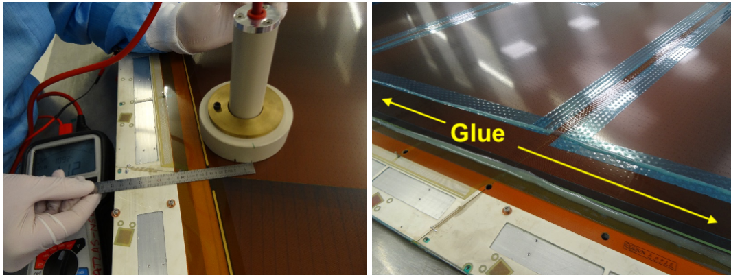
Figure 13: Left: Resistance measurement, with a 1\text{ cm}^2 probe (hidden by the plastic disk), as a function of the distance from the edge. Right: Passivation with tape masking and glue application.
