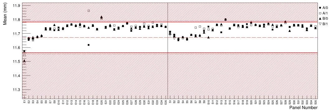
Figure 18: Mean thickness of panels as a function of the panel rank and for the two RO panels categories. Values are given for each of the four possible configurations (Side 1 or 2 [A/B], vacuum on or off [0/1]) of the measurements.
