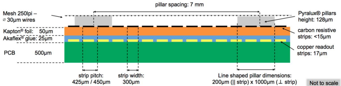
Figure 6: Structure of the RO boards. The mesh is also represented (250 Lines Per Inch).
