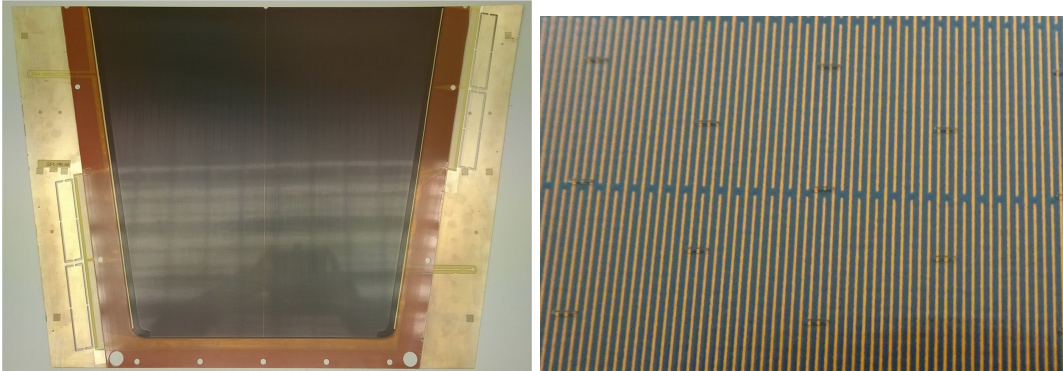
Figure 7: Left: Picture of a trapezoidal readout board (PCB1) already glued on a RO panel. Right: Detail of a Readout PCB where resistive strips and line shaped pillars are visible.
