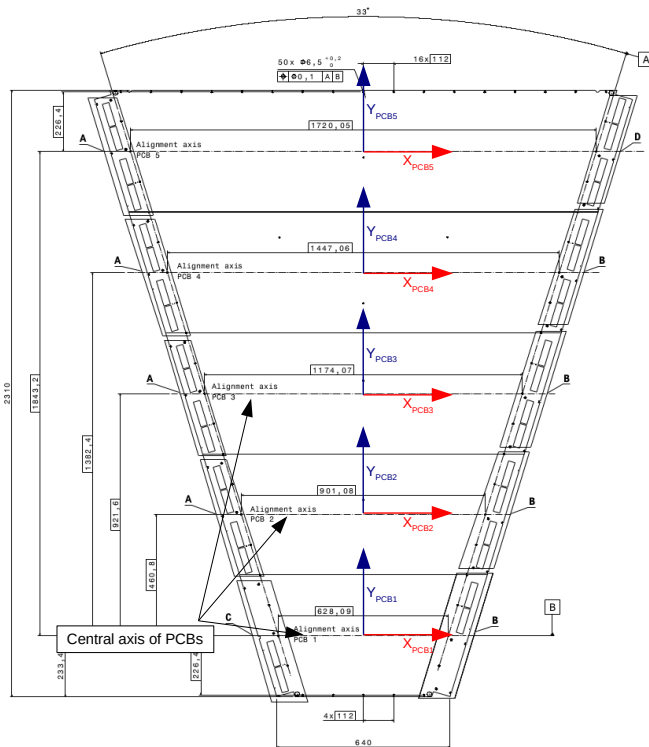
Figure 30: The PCB coordinate system used in the metrology reconstruction. The frames are aligned in the precision direction with the centres of the Rasnik masks along the central line of the PCBs, and with the nominal positions of the precision washers glued on each board. By definition, the coordinate systems of the layer coincides with that of the 5th PCB, and that of the panel coincides with that of the first layer. All coordinate systems are right-handed.
