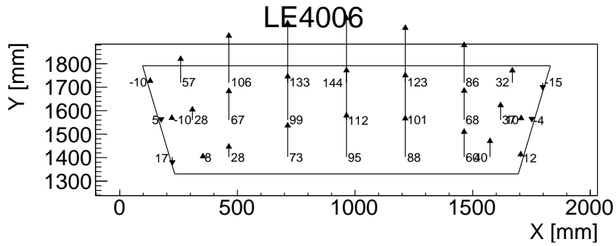
Figure 27: Gantry measurement of a (spare) RO PCB on which several cut-outs on the resistive layer have been performed, in order to measure the copper strips on multiple points across the PCB surface. The Right-most and left-most measurements are Rasknik masks. The other measurements are copper strips. The reported numbers are in \mu\text{m} and are deviations to the nominal along the precision (Y) direction.
