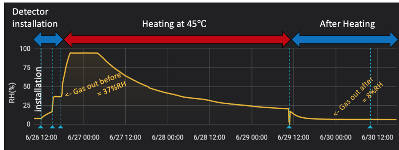
Figure 40: Gas relative humidity in % before and after the heating. Just after the connection of the module on the CTB gas system, the module output relative humidity is 37%. Then it is heated at 45 °C to help water out-gassing during three days. Once a stable mode is achieved (the humidity has decreased), the heating is turned off. The detector output reaches then 8% RH.
