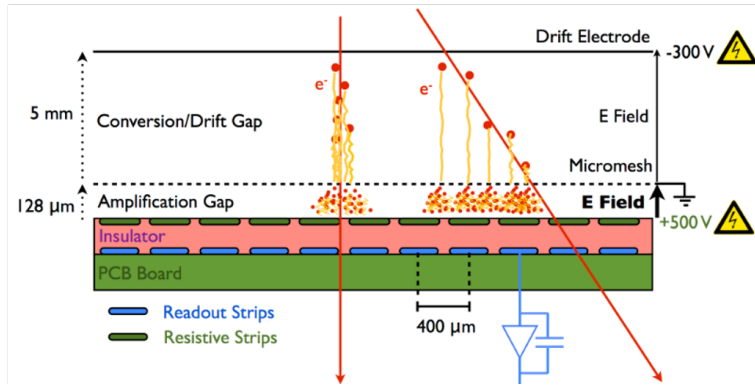
Figure 2: Design of the Micromegas architecture used in the NSW.
