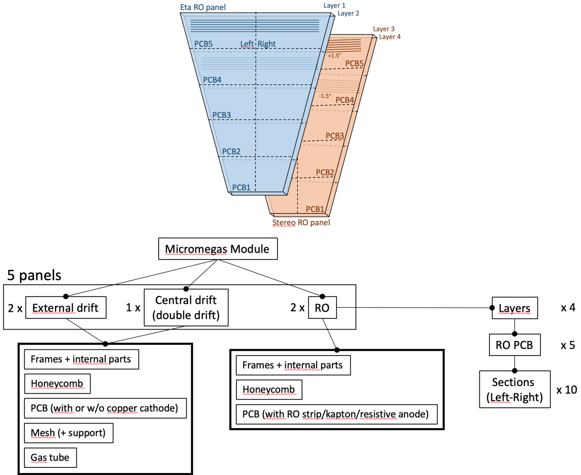
Figure 4: Top: Orientation of strips in different layers of LM1 modules. Each readout panel holds 2 layers (one on each side). Each layer is made of 5 boards, divided in 2 sections (left/right). Bottom: Breakdown structure of a LM1 MM module.
