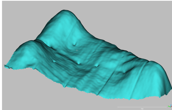
Figure 20: Typical reconstructed top surface of a module. Isometric projection. The scale bar applies to all 3 coordinates, but the Z coordinate is magnified by x1000 (X and Y in mm, Z in \mu\text{m} ). The observed peak-to-peak \Delta Z variation was 600 \mu\text{m} for this module (Module 21).
