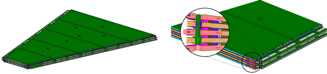
Figure 5: Left: Overview of an assembled quadruplet. The junctions between the 5 PCBs as well as the six interconnections that link the external sides of the outer drift panels are indicated by black circles. Right: Zoom on large base; details of gas and cooling inlets; transverse view of drift panels (cyan), readout panels (yellow) and gas-gap frames (pink). In the circle: cross-section of the module corner showing the alignment pin (green), the gas-gap frame (pink), the mesh frame (purple) and the gas distribution system (corner + gas insert + gas pipe).
