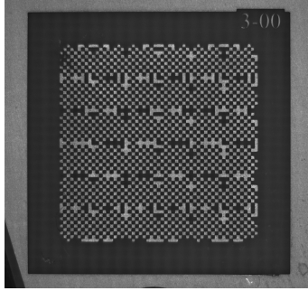
Figure 23: A Rasnik mask etched on PCB.
