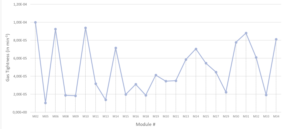
Figure 37: Module Gas Tightness measurements. The gas tightness has been defined as the volume of leak gas normalised by the detector volume per time unit.
