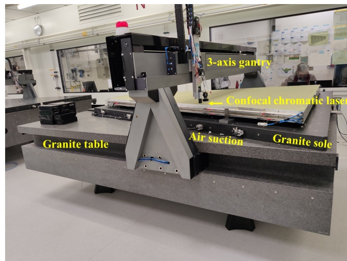
Figure 9: Planarity scan survey of a module.
