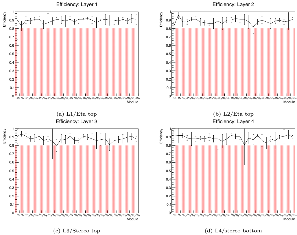
Figure 53: Average efficiency of each module validated on the cosmic bench. The uncertainty bars are the RMS evaluated from 10 different values, each one corresponding to a HV sector in the layer. Layer efficiencies falling below the red line do not fulfill the requirements.
