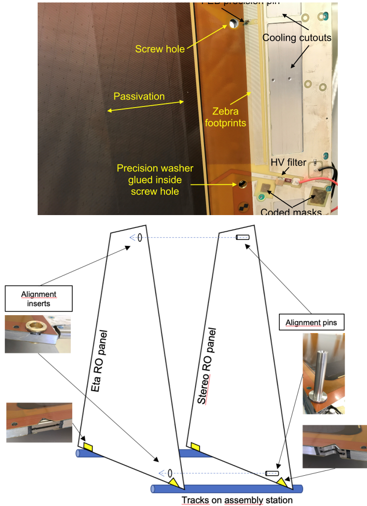
Figure 12: Top: Detail of a RO panel. Coded masks needed to glue the precision washer are indicated. The precision pin for electronics positioning and the RO strips footprints are also shown. Bottom: Positioning scheme of RO panels on the assembly station tracks (see Section 3.2.5). Alignment inserts and pins are represented.
