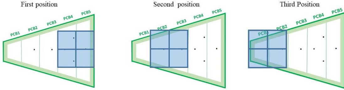
Figure 39: Sketch of the procedure to scan the LM1 quadruplet with the M^3 tracker. The cosmic muon scan starts with the two largest PCBS (4 and 5), the second position is devoted to the two intermediate PCBS (3 and 2) and the last position is devoted to PCB1. The interconnections are indicated by black dots in the sketch. The green band around the border of the module represents the average passivated area.
