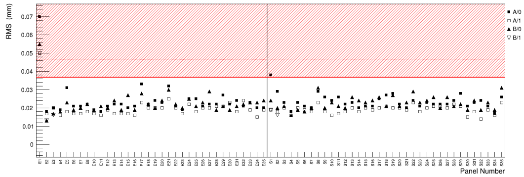
Figure 19: Panel thickness RMS as a function of the panel rank (see caption of Fig. 18 for the symbols explanations)
