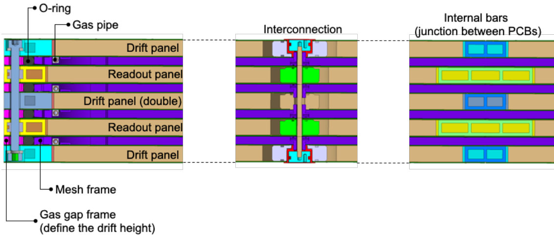
Figure 3: Section of a MM quadruplet with details of the internal components on the edges, at the interconnections and at a PCB junction. Panels are made of aluminum honeycomb (brown), external frames (cyan for drift and yellow for RO) and PCB (0.5 mm thick) where electrodes (drift cathode and anode strips) are printed. Gas-gap frames (pink) define the gas-gap thickness and the O-ring groove. Interconnections are made of two external nuts and one thread rod passing through all panels and reinforcement parts. Internal bars used to reinforce panels at PCB junctions are shown in blue for drift panels and green for RO panels (wider bars because of the angle on the PCB edge for stereo panels).
