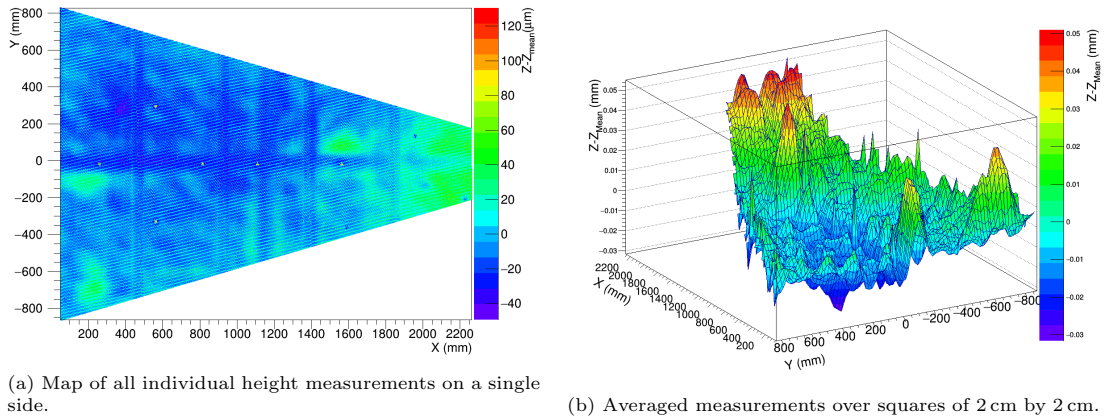
Figure 17: Examples of panel height measurements.
