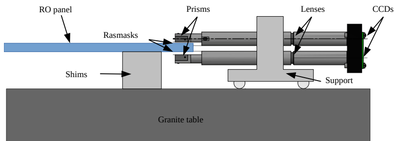
Figure 28: Rasfork principle.
