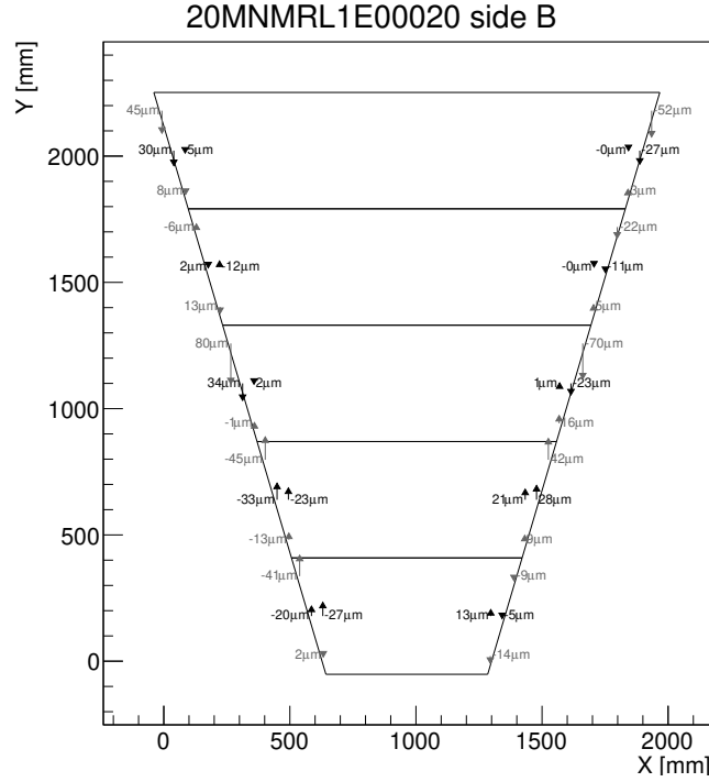
Figure 26: Example RO panel measurement with the gantry CMM.
