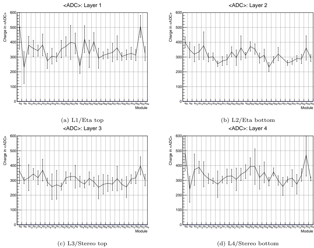
Figure 51: Average number of ADC counts for each module validated on the cosmic bench. The uncertainty bars are the RMS evaluated from 10 different values, each one corresponding to a HV sector in the layer.
