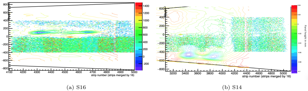
Figure 54: Comparison between signals observed on the cosmic test bench and the planarity scan made during construction. Contour lines correspond to height measurement from the planarity scans. The height is given by the vertical scales. The effect of holes is clearly seen in the inefficiency of detectors.
