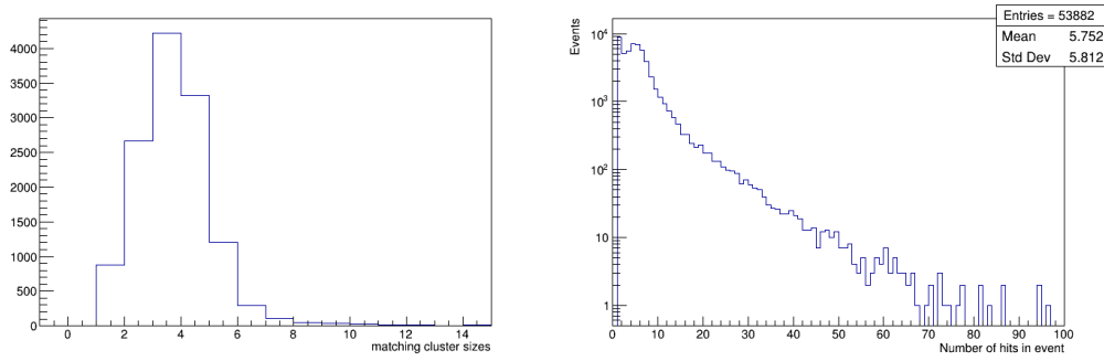
Figure 46: Left: Size of clusters matched to good M^3 tracks for the layer 1 of Module 11 PCB1. Right: Distribution of hit multiplicity in one FEU for events recorded in the module.
