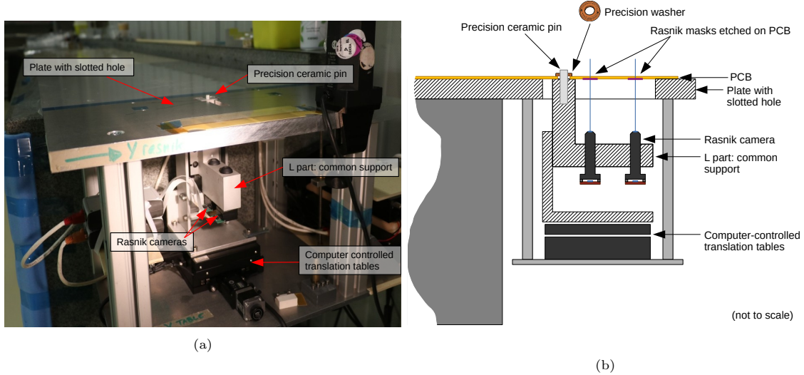
Figure 25: The precision washer gluing tool (a) and principle of operation (b).
