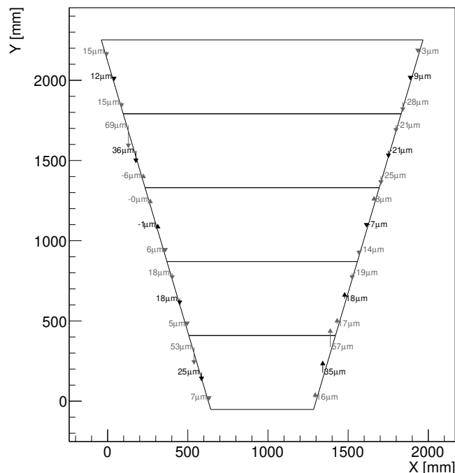
Figure 29: Example of a RO panel measured with the Rasfork. The reported measurements are the position differences in the precision coordinate Y between the Rasnik masks on the two faces of the panel. In black are the masks along the central line of the PCBs, in gray are the masks in the corner of the PCBs.
