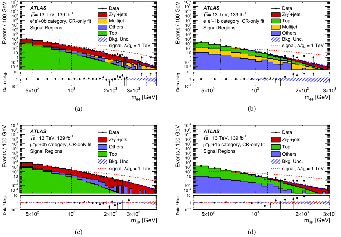
Figure 2: Data overlaid on SM background postfit m_{\ell\ell} distributions in the SRs of the (a) electron b -veto, (b) electron b -tag, (c) muon b -veto and (d) muon b -tag categories. “Others” refers to diboson and W +jets events. MC statistical uncertainties and systematic uncertainties are considered (hatched band). The prefit signal distribution is presented as well for a hypothesis of \Lambda/g_* = 1 TeV. The bottom panels show the ratio of the data to the background prediction, while the arrows correspond to bins where the ratio is beyond the limits of the figure. The last bin is an overflow bin, which contains the yields in the bins beyond it. The dashed and dotted lines mark the transition point where the extrapolation is used in the analysis for the top and multijet backgrounds, respectively.
