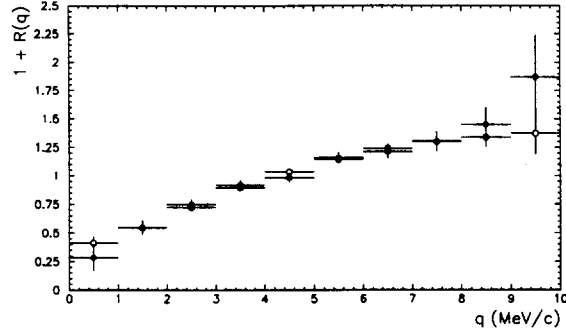
Figure 7. Experimental correlation function (solid circles) measured in SPEG compared to the correlation function (open circles) predicted by the classical model for the mean lifetime \tau = 3.9 \cdot 10^{-21} s and convoluted with the response function of the spectrometer.
