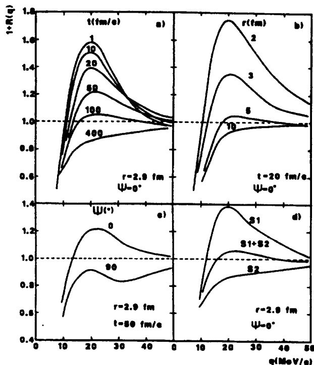
Figure 5. Theoretical p-p correlation functions obtained with different sets of parameters r and \tau and the angle \psi . In d) S1 corresponds to \tau = 20 fm/c and S2 to \tau = 400 fm/c. The result obtained with mixed sources (30%, 70%) is labelled S1+S2.
