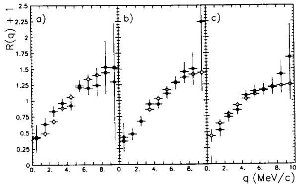
Figure 9. Experimental two-proton correlation function (solid circles) compared to the prediction of the classical model for the lifetime \tau = 3.9 \cdot 10^{-21} \text{s} and the source velocity v_s = 0.27c (open circles), constructed for three different gates on the relative orientation of the vector of the momentum difference and the pair velocity : \cos \psi \in (0, 1/3) (a), \cos \psi \in (1/3, 2/3) (b), \cos \psi \in (2/3, 1) (c).
