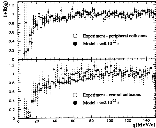
Figure 2. Experimental d-d correlation functions compared with the predictions of the classical model.
