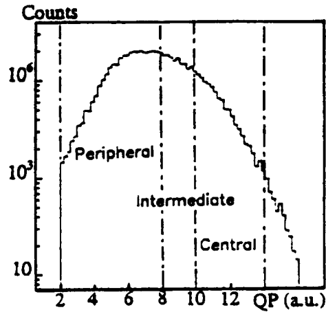
Figure 1. Distribution of all coincident events with respect to the centrality parameter QP determined in the text.
