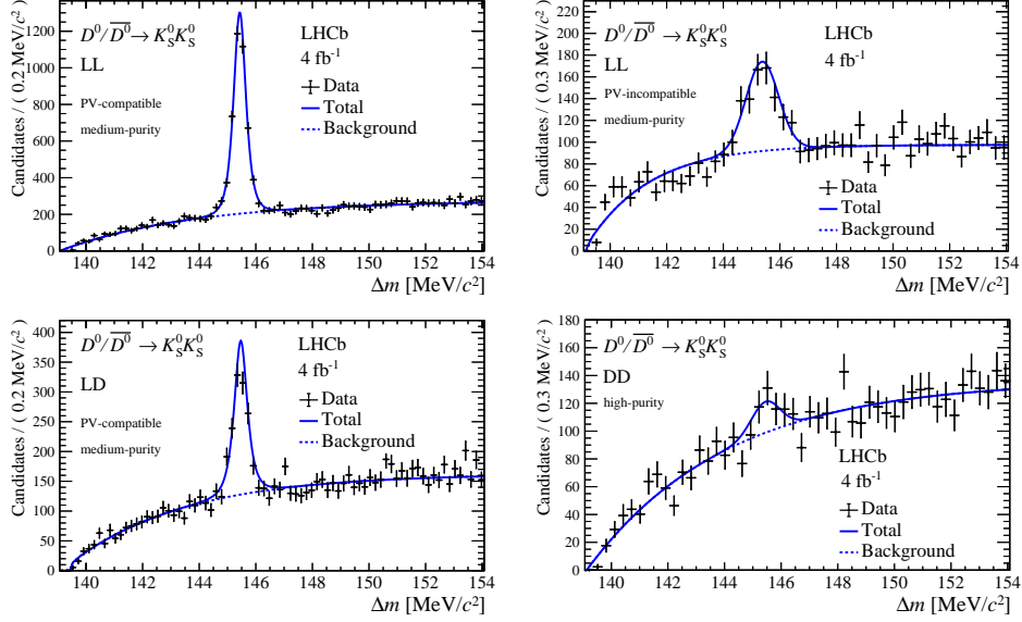
Figure 1: Distributions and fit projections of the \Delta m observable for representative candidate categories (2017–2018 data). See text for the definition of purities.
