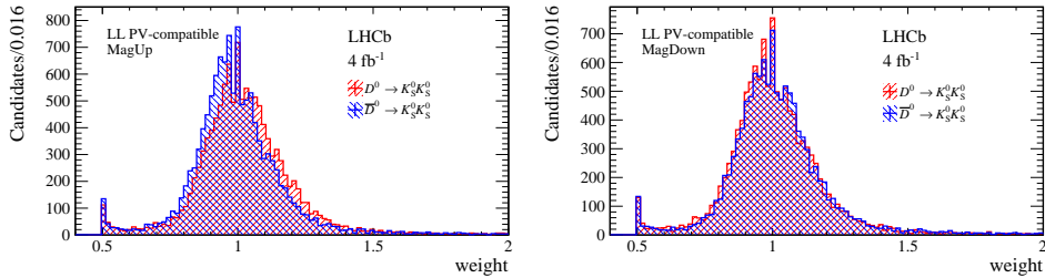
Figure 2: Distributions of weights (2017–2018 data) applied to signal candidates in the global fit to correct for detector, production, and physics of the calibration channel. Differences between MagUp (left) and MagDown (right) are a consequence of different D^0 and \bar{D}^0 acceptances, and of detector asymmetries. A small fraction of entries with large weights fall outside the range of the plot.
