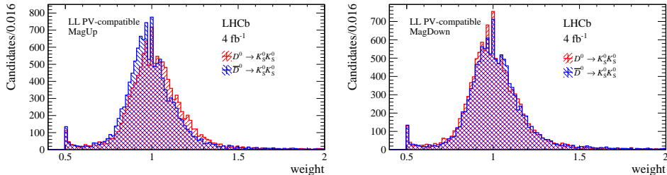
Figure 2: Distributions of weights (2017–2018 data) applied to signal candidates in the global fit to correct for detector, production, and physics of the calibration channel. Differences between MagUp (left) and MagDown (right) are a consequence of different D^0 and \bar{D}^0 acceptances, and of detector asymmetries. A small fraction of entries with large weights fall outside the range of the plot.
