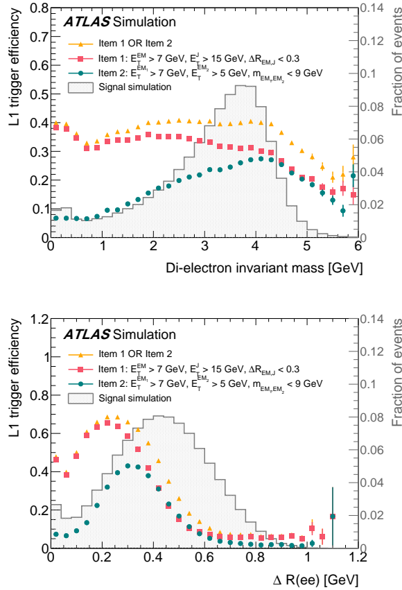
Figure 7: Efficiency of L1Topo triggers developed for B -meson decays with di-electron final states. The efficiency is determined using non-resonant B_d^0 \rightarrow K^{*0} e^+ e^- decays, and it is shown (a) as a function of the offline invariant mass of the signal electron pairs and (b) as a function of their angular separation \Delta R . The L1 efficiency (coloured filled markers) is displayed separately for the two considered L1 items as well as their combination. The expected signal distribution is superimposed (filled grey histogram).
