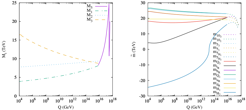
Figure 2: Left panel: Renormalization effects on the SU(5) gaugino mass M_5 , exhibiting its sharp decrease as \mu \rightarrow M_X from above, and the subsequent evolution of the SM gaugino masses M_{1,2,3} at lower scales, following threshold corrections at the GUT scale. Right panel: Corresponding evolution of the squark and Higgs masses. Our benchmark point with m_{1/2} = 20 TeV is assumed, with the other parameter values specified in the text.
