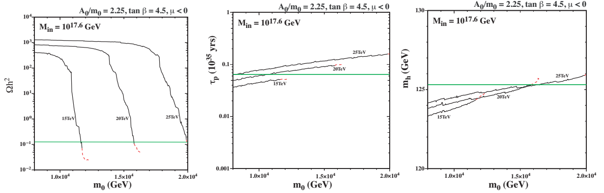
Figure 6: Values of \Omega_{\text{LSP}} h^2 (left panel), \tau(p \rightarrow K^+ \nu) (center panel) and m_h (right panel) as functions of m_0 for the indicated fixed values of m_{1/2} \in [15, 25] \text{ TeV} and for the same input parameters as in the upper left panel of Fig. 3. Values calculated when the LSP is a bino are shown as solid black lines, becoming dashed red lines when the LSP is the lighter stop and terminating when the RGE calculations break down. The horizontal green lines correspond to the cosmological value of \Omega_{\text{LSP}} h^2 , the experimental lower limit on \tau(p \rightarrow K^+ \nu) and the experimental value of m_h , respectively.
