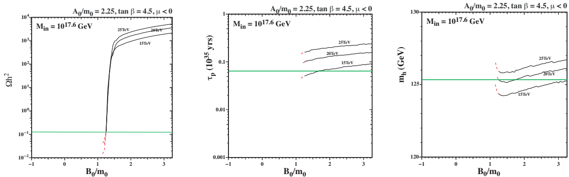
Figure 9: As in Fig. 6, as functions of B_0/m_0 for the indicated fixed values of m_{1/2} \in [15, 25] TeV and m_0 chosen to obtain the cosmological value of \Omega_{\text{LSP}}h^2 for B_0 = A_0 - m_0 , with the same values of the other input parameters as in Fig. 3.
