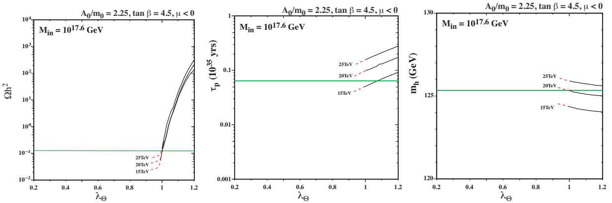
Figure 7: As in Fig. 6, as functions of \lambda_\Theta for the indicated fixed values of m_{1/2} \in [15, 25] TeV and m_0 chosen to obtain the cosmological value of \Omega_{\text{LSP}}h^2 for \lambda_\Theta = 1 , with the same values of the other input parameters as in Fig. 3.
