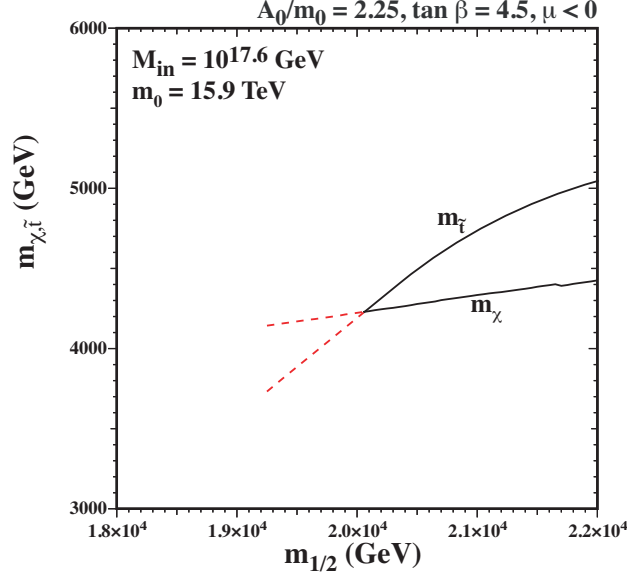
Figure 5: The values of m_\chi and m_{\tilde{t}_1} (solid black lines in the bino LSP region, dashed red lines in the stop LSP region) as functions of m_{1/2} for the parameters \tan \beta = 4.5 , M_{\text{in}} = 4 \times 10^{17} \text{ GeV} , M_\Theta = 3 \times 10^{17} \text{ GeV} , \lambda' = 0.005 and \lambda_\Theta = 1 , with m_0 chosen to obtain the cosmological value of \Omega_{\text{LSP}} h^2 for m_{1/2} = 20 \text{ TeV} .
