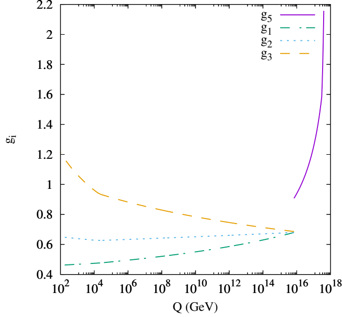
Figure 1: Evolutions of the SM gauge couplings g_{1,2,3} with the renormalization scale \mu below the GUT scale, exhibiting their unification and the rapid increase of g_5 above the GUT scale. We assume a benchmark point with m_{1/2} = 20 TeV: the values of the other benchmark parameters are specified in the text.
