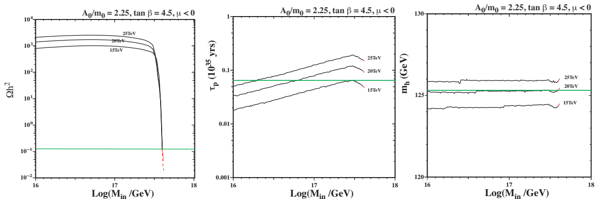
Figure 11: As in Fig. 6, as functions of M_{\text{in}} for the indicated fixed values of m_{1/2} \in [15, 25] TeV and m_0 chosen to obtain the cosmological value of \Omega_{\text{LSP}} h^2 for M_{\text{in}} = 4 \times 10^{17} GeV, with the same values of the other input parameters as in Fig. 3.
