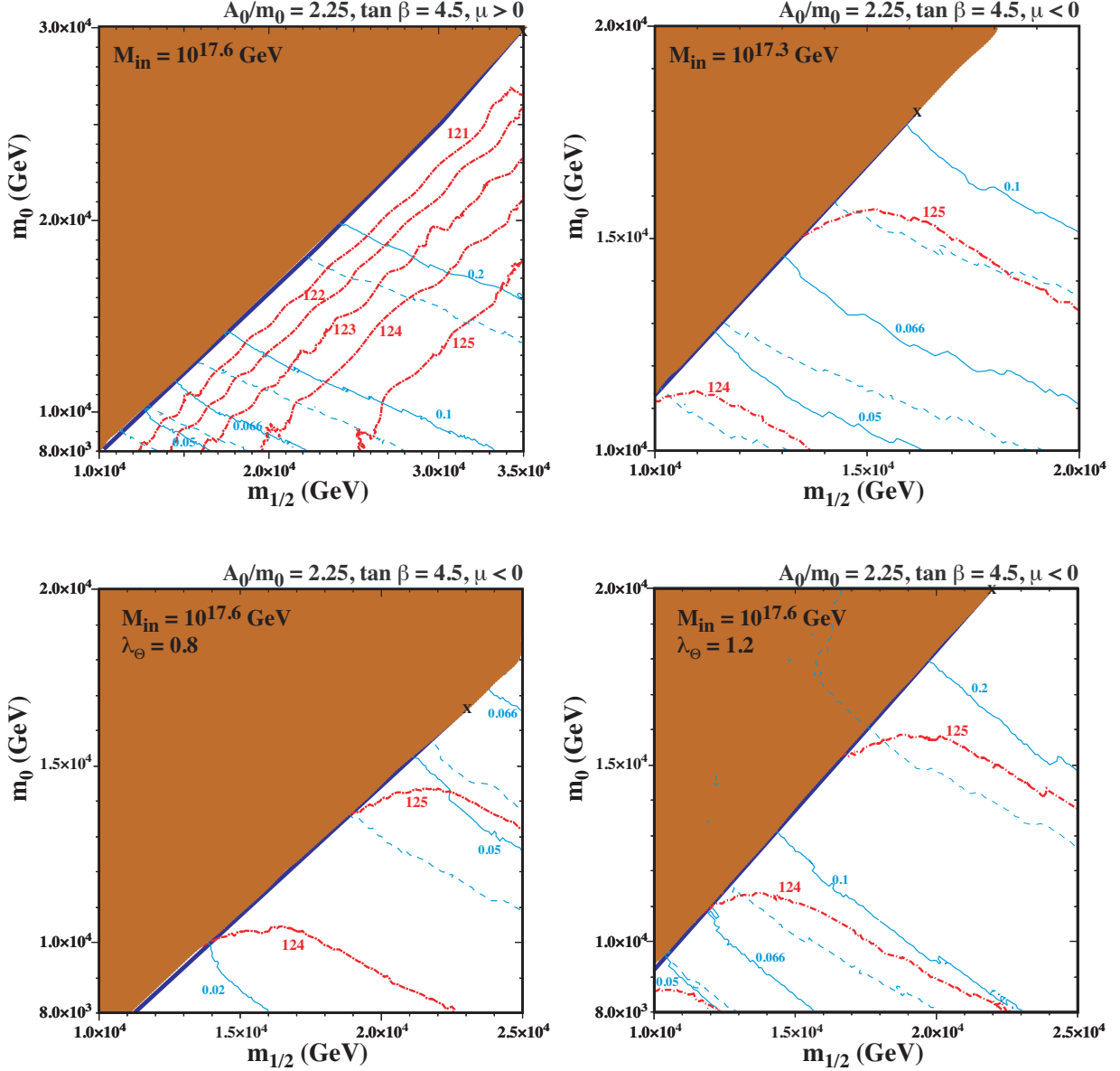
Figure 4: Upper left panel: The (m_{1/2}, m_0) plane for the parameters \tan\beta = 4.5 , A_0 = 2.25m_0 , B_0 = 1.25m_0 , M_{\text{in}} = 4 \times 10^{17} \text{ GeV} , M_{\Theta} = 3 \times 10^{17} \text{ GeV} , \lambda' = 0.005 and \lambda_{\Theta} = 1 with \mu > 0 . Upper right panel: The corresponding plane with M_{\text{in}} = 2 \times 10^{17} \text{ GeV} , \mu < 0 and unchanged values of the other parameters. Lower panels: The corresponding planes with \lambda_{\Theta} = 0.8 (left) and \lambda_{\Theta} = 1.2 (right), with \mu < 0 , and M_{\text{in}} = 4 \times 10^{17} \text{ GeV} and unchanged values of the other parameters. In each panel, the cross marks the endpoint of the stop coannihilation strip.
