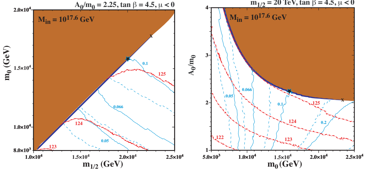
Figure 3: Left panel: The (m_{1/2}, m_0) plane for the parameters \tan \beta = 4.5 , A_0 = 2.25m_0 , B_0 = 1.25m_0 , M_{\text{in}} = 4 \times 10^{17} \text{ GeV} , M_{\Theta} = 3 \times 10^{17} \text{ GeV} , \lambda' = 0.005 and \lambda_{\Theta} = 1 with \mu < 0 . Right panel: The (m_0, A_0/m_0) plane with B_0 = A_0 - m_0 and unchanged values for the other model parameters. Here and subsequently, the brown shaded regions are excluded because the LSP is the lighter stop, in the narrow dark blue strips the relic LSP density \Omega_{\text{LSP}} h^2 \in (0.05, 0.2) , the dot-dashed red lines are contours of m_h calculated using FeynHiggs 2.18.0 , and the solid (dashed) blue lines are contours of \tau(p \rightarrow K^+ \nu) in units of 10^{35} \text{ y} calculated with central ( -1\sigma ) values of the decay matrix elements and \alpha_s .
