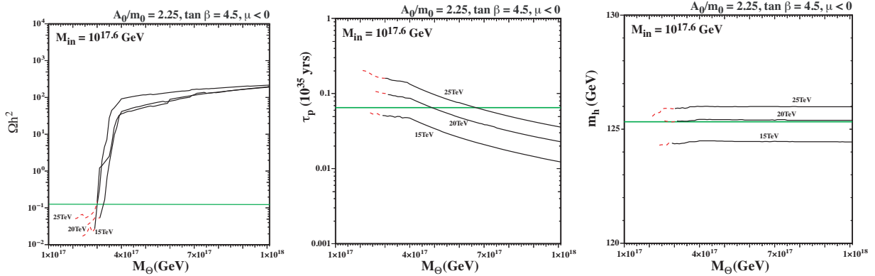
Figure 10: As in Fig. 6, as functions of M_\Theta for the indicated fixed values of m_{1/2} \in [15, 25] TeV and m_0 chosen to obtain the cosmological value of \Omega_{\text{LSP}} h^2 for M_\Theta = 3 \times 10^{17} GeV, with the same values of the other input parameters as in Fig. 3.
