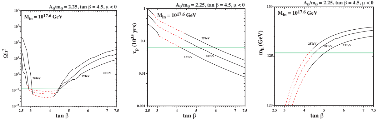
Figure 8: As in Fig. 6, as functions of \tan\beta for the indicated fixed values of m_{1/2} \in [15, 25] TeV and m_0 chosen to obtain the cosmological value of \Omega_{\text{LSP}}h^2 for \tan\beta = 4.5 with the same values of the other input parameters as in Fig. 3.
