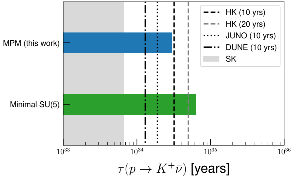
Figure 13: The ranges of p \rightarrow K^+ \bar{\nu} lifetimes found here in the CMSSM for the super-GUT MPM (blue band) and in the minimal SU(5) (green band; see Ref. [22]) compared with the sensitivities of the JUNO [30], DUNE [31] and Hyper-K [32] experiments. The gray shaded area is excluded by the Super-Kamiokande experiment [26].
