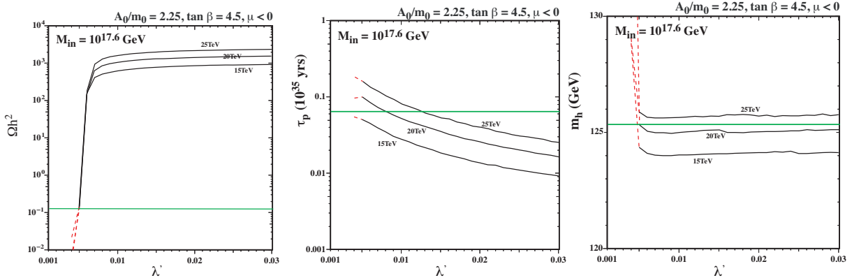
Figure 12: As in Fig. 6, as functions of \lambda' for the indicated fixed values of m_{1/2} \in [15, 25] TeV and m_0 chosen to obtain the cosmological value of \Omega_{\text{LSP}} h^2 for \lambda_\Theta = 0.005 , with the same values of the other input parameters as in Fig. 3.
