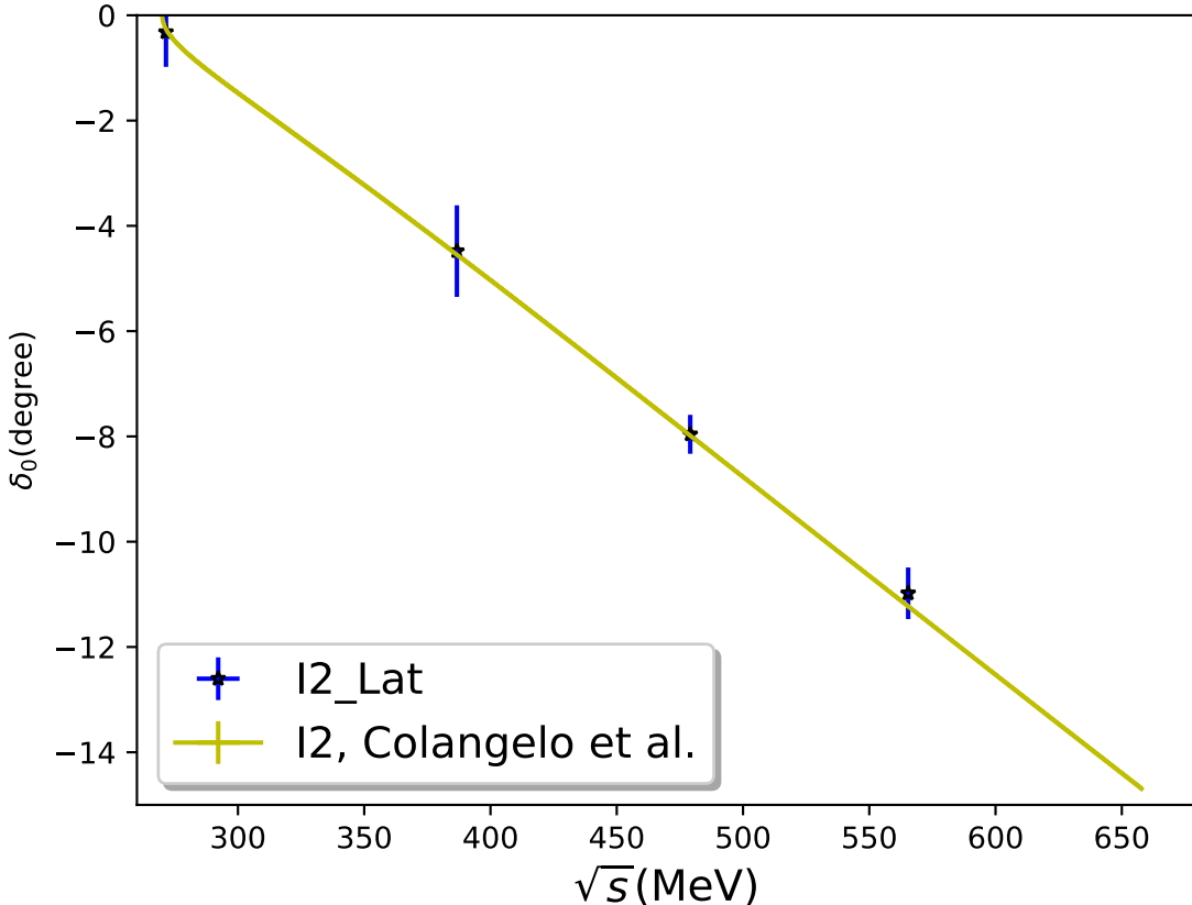
FIG. 14: The results for the I = 2 phase shifts together with the corresponding dispersive results [13] that are shown in Fig. 13, but here with an expanded scale.
