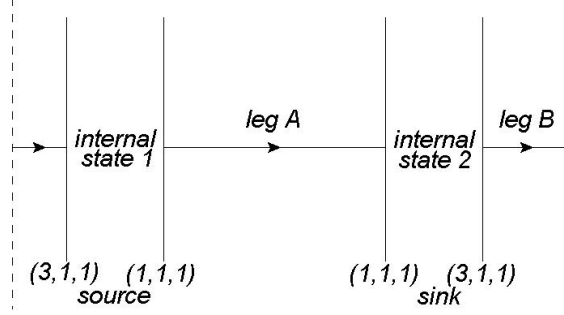
FIG. 7: A typical diagram for the decomposition of the ATW effect when the Green's function is constructed from two O_b operators. For the first-order ATW effect, both legs are pions with momentum (1, 1, 1)\pi/L , which means if one of the internal states is the vacuum, e.g., internal state 1, then the other internal state cannot be the vacuum. For the second order ATW effect, we can choose leg A to be (1, 1, 1)\pi/L and leg B to be (3, 1, 1)\pi/L , while keeping both internal states to be the vacuum state.
