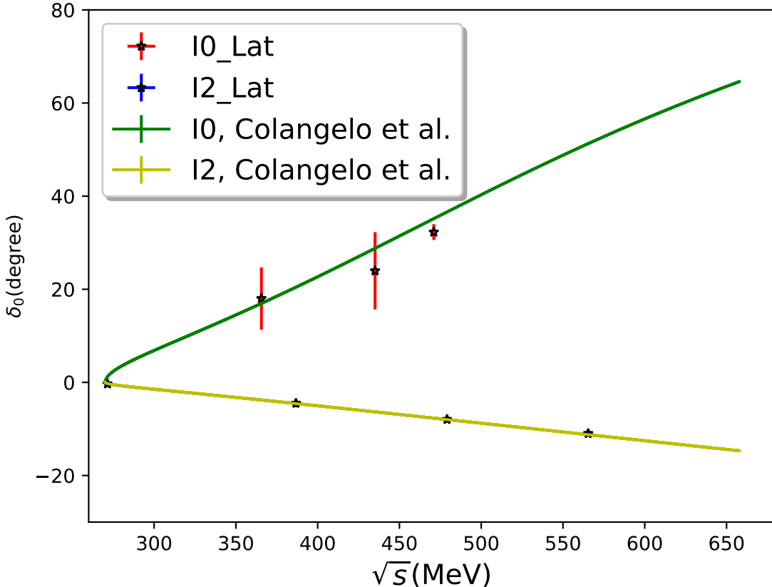
FIG. 13: A graph of our results for the seven phase shifts for I = 0 and I = 2 as a function of energy. Shown also on the plot are the corresponding dispersive results [13]. Note: the errors are not shown for the dispersive results.
