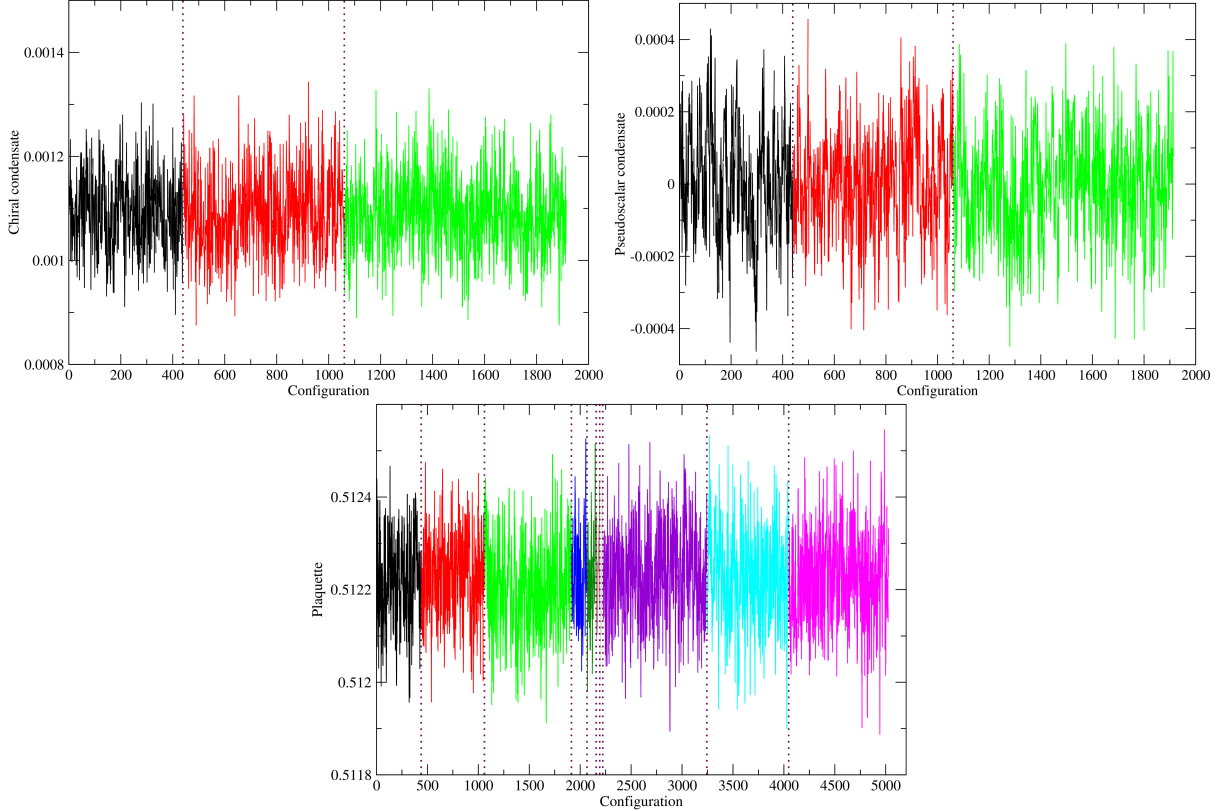
FIG. 1: Evolution of the chiral condensate (upper-left), pseudoscalar density (upper-right) and plaquette (lower). The different colors and vertical dotted lines indicate the boundaries of the 10 independent Markov chains. Note that measurements of the chiral condensate and pseudo-scalar density were performed only on the subset of configurations corresponding to the first three chains of the lower figure. The last three ensembles in the lower figure were generated using the EOFA technique.
