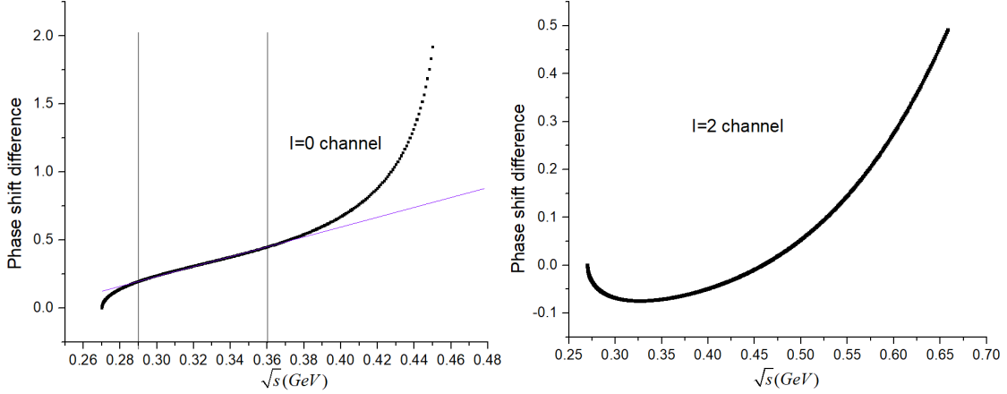
FIG. 12: A ChPT calculation of the difference between the scattering phase shift evaluated at the physical pion mass and the pion mass calculated for our ensemble, \delta_I(m_\pi = 142 \text{ MeV}) - \delta_I(m_\pi = 135 \text{ MeV}) , as a function of \sqrt{s} defined in Eq. (50) and shown in degrees. For the I = 0 channel, at large \sqrt{s} , the ChPT calculation begins to break down while at lower \sqrt{s} , the relation is approximately linear, which is consistent with the dispersive prediction. The straight line is a linear fit to the ChPT result in the region 290 \text{ MeV} \leq \sqrt{s} \leq 360 \text{ MeV} .
