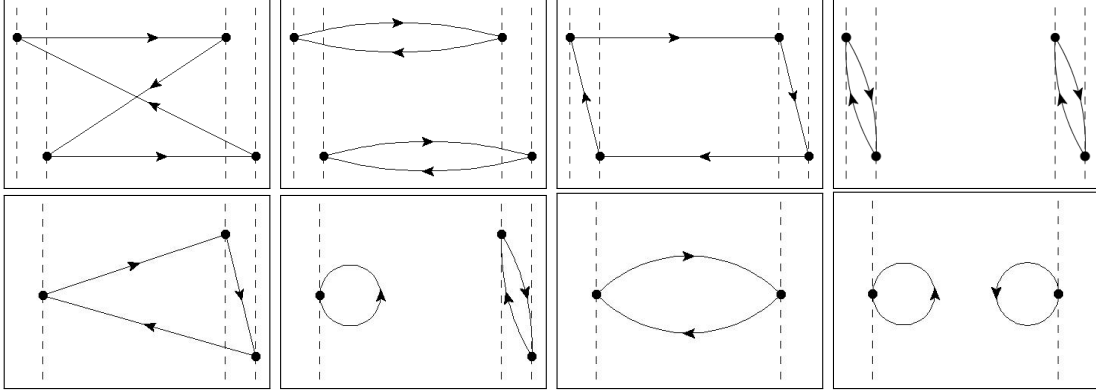
FIG. 3: Diagrams showing the contractions which contribute to the two-point functions involving the \pi\pi(\dots) and \sigma operators. The solid dots indicate the positions of the pion two-quark operators and the dotted vertical lines passing through these points indicate the separate 3-dimensional time slices on which these operators are placed, with the nearby pairs of lines separated by four time units as described in Eq. (15). Identical diagrams appear for the \sigma operator only with a single vertical line at the source and/or sink, with the dots now representing the scalar bilinear. The top 4 diagrams are labeled by C , D , R and V diagrams from left to right, and the lower 4 diagrams are labeled by C_{\sigma\pi\pi} , V_{\sigma\pi\pi} , C_{\sigma\sigma} and V_{\sigma\sigma} from left to right.
