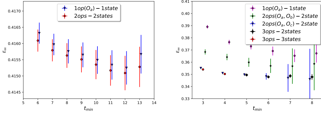
FIG. 5: The t_{\text{min}} dependence of fitted ground state energy for the stationary \pi\pi_{I=2} channel (left) with t_{\text{max}} = 25 and the stationary \pi\pi_{I=0} channel (right) with t_{\text{max}} = 15 . Left: The circles represent the two-operator, two-state fit and downward pointing triangles the one-operator, one-state fit. Right: The pentagons represent the one-operator, one-state fit. The stars and downward pointing triangles show the results from the two two-operator, two-state fits. Finally the circles show the three-operator, three-state fit for t_{\text{min}} = 3 and 4 while the diamonds show the three-operator, two-state fit for t_{\text{min}} = 5 - 8 . For the I = 0 channel, including additional operators (especially the \sigma ) substantially improves the determination of the ground state energy.
